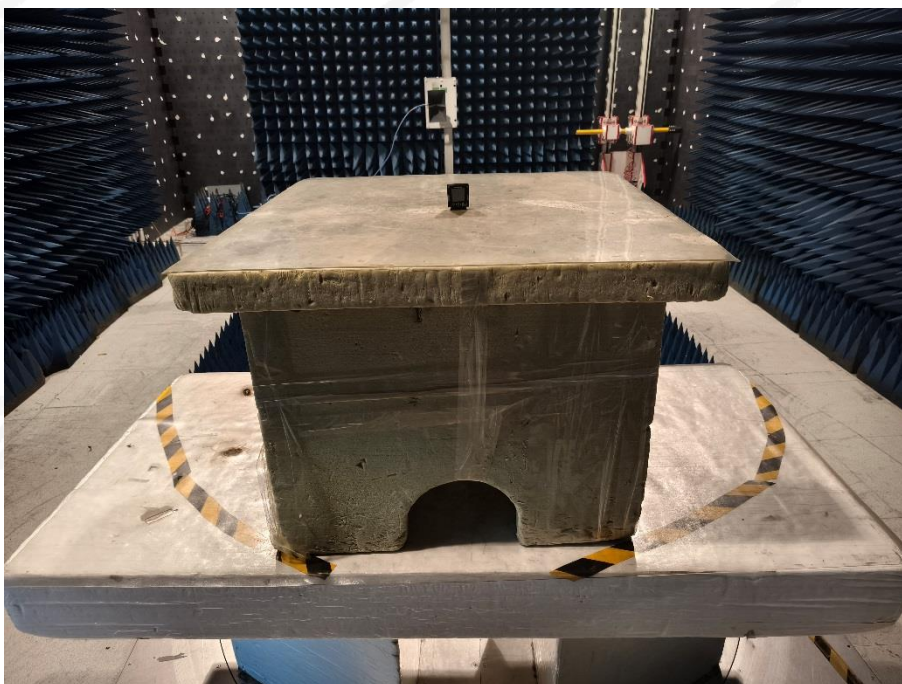
RE (18-40GHz)
