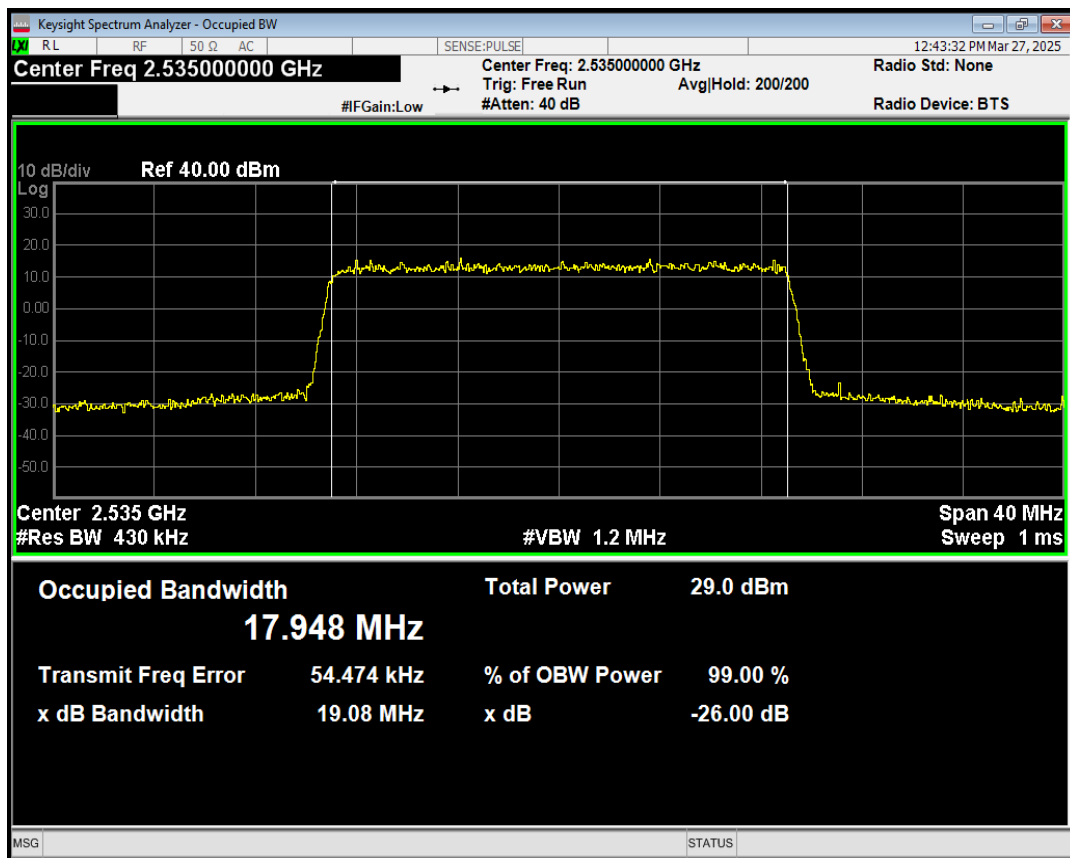
Band7 QAM16 BW=20MHz Channel=21100 RB Size=27 Position=#0
