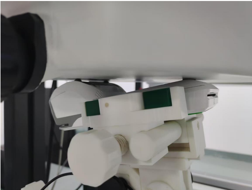
Body and hotspot Back side (separation distance is 0mm)
