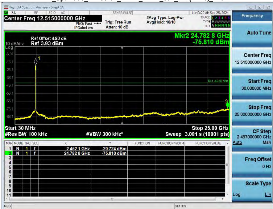
2_Spurious_Emission_NVNT_ANT2_802_11n(HT40)_2437
