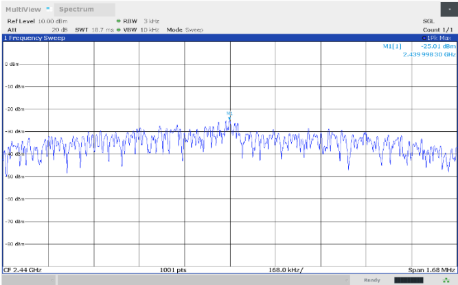
Figure 8.6-5: Power spectral density, GFSK, 2 Mbps, 2440 MHz
