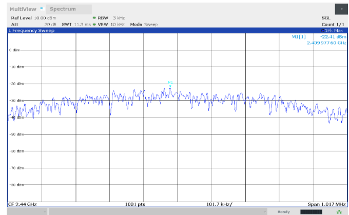
Figure 8.6-2: Power spectral density, GFSK, 1 Mbps, 2440 MHz
