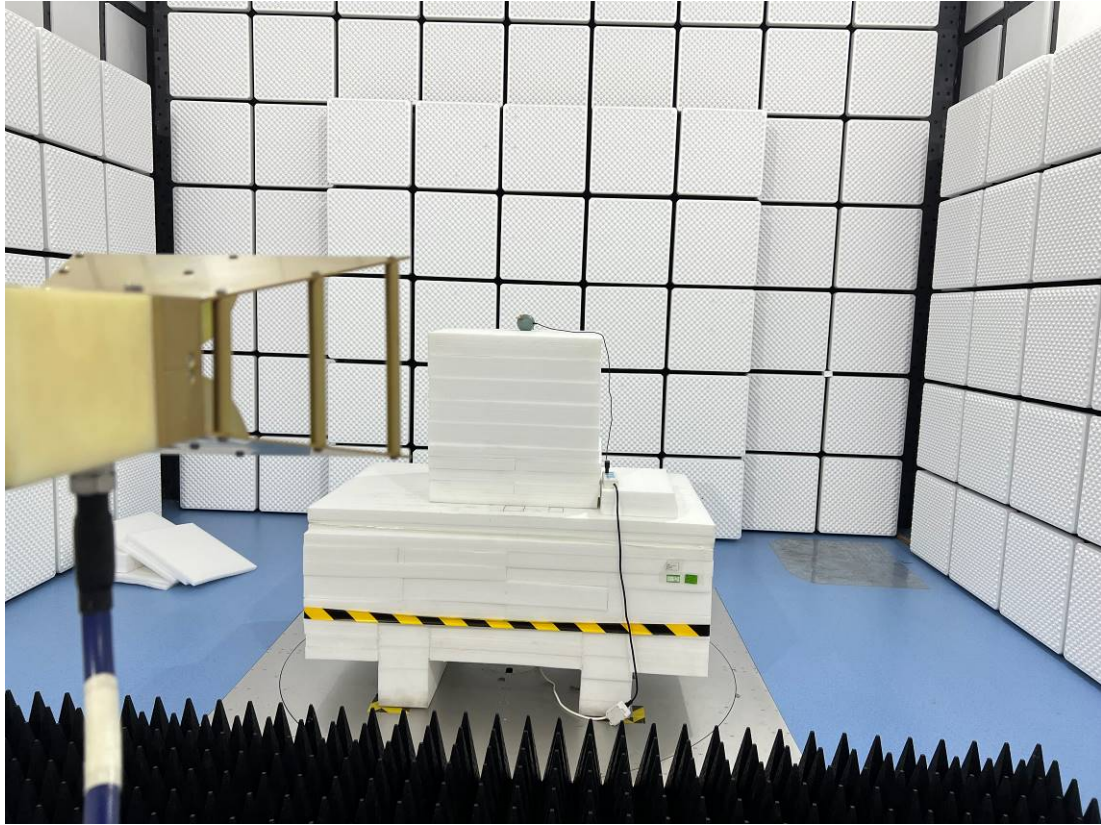
RE - Front Side (3GHz -18GHz)
