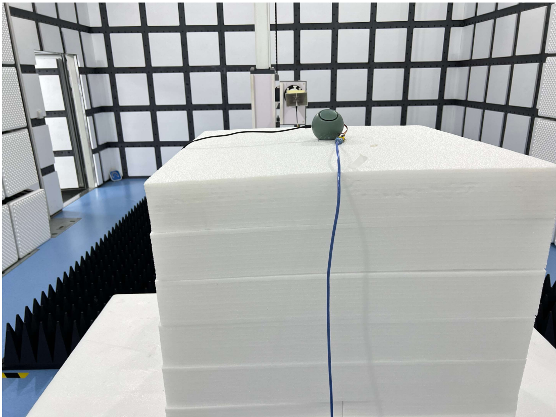
RE - Front Side (18GHz -25GHz)
