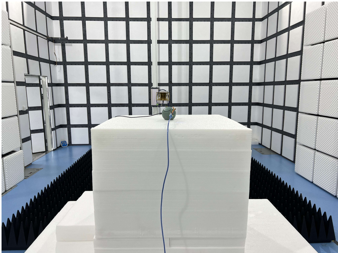
RE - Front Side (1GHz -3GHz)
