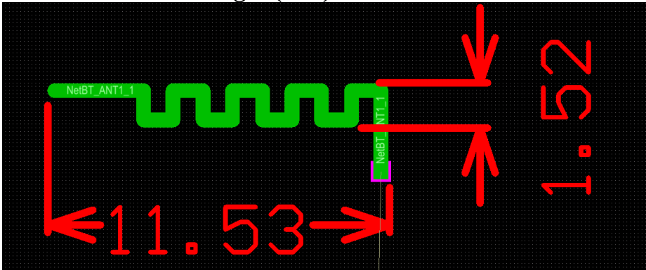
Antenna Photo & Length (mm)
