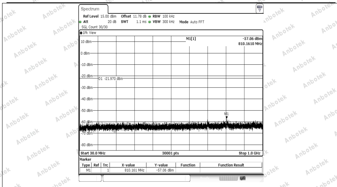
ZigBee-Ant1-2440-30~1000-PASS
