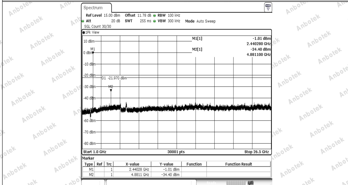
ZigBee-Ant1-2440-1000~26500-PASS
