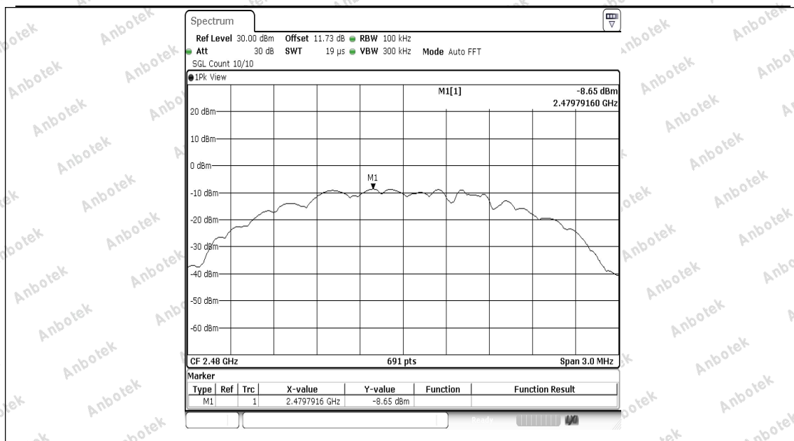
ZigBee-Ant1-2480-0~Reference-PASS
