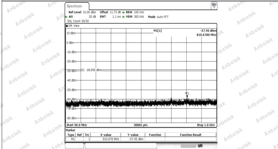
ZigBee-Ant1-2480-30~1000-PASS
