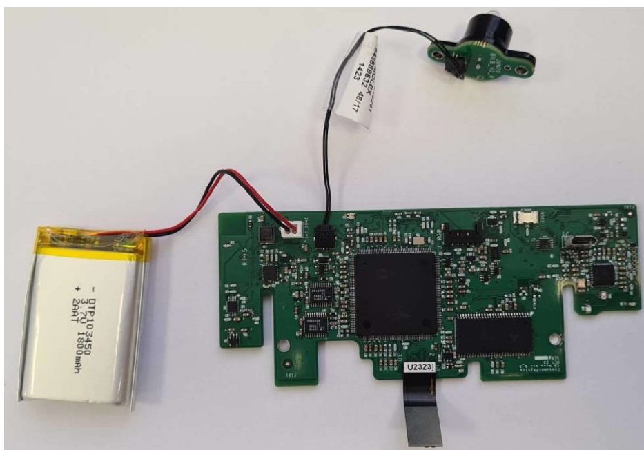
Photograph № 7, 8 SCIUCUP PCB internal view
