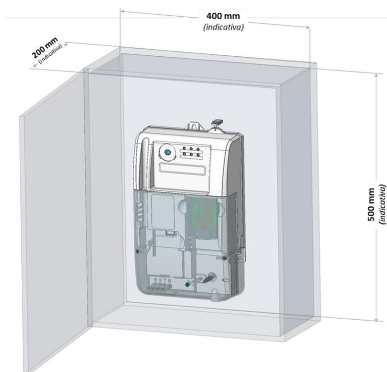
Figure 4 Example of LVM G3 Hybrid installation
