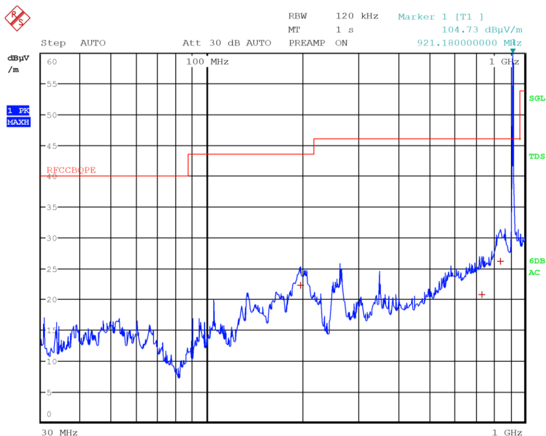
Figure 8.7-7: Radiated spurious emissions on mid channel with antenna in horizontal polarization – Frequency range 30 to 1000 MHz
