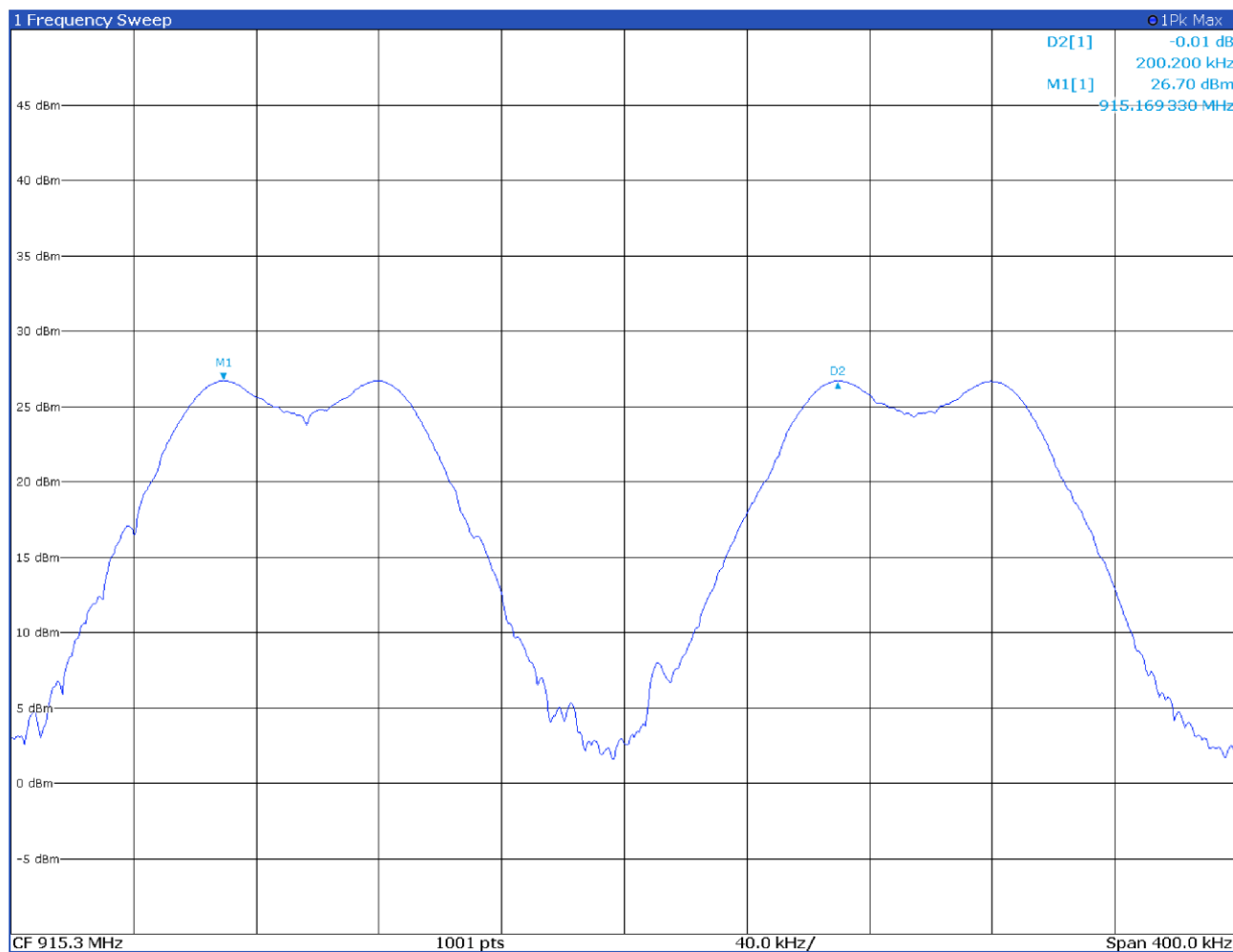
Figure 8.5-7: Carrier frequency separation
