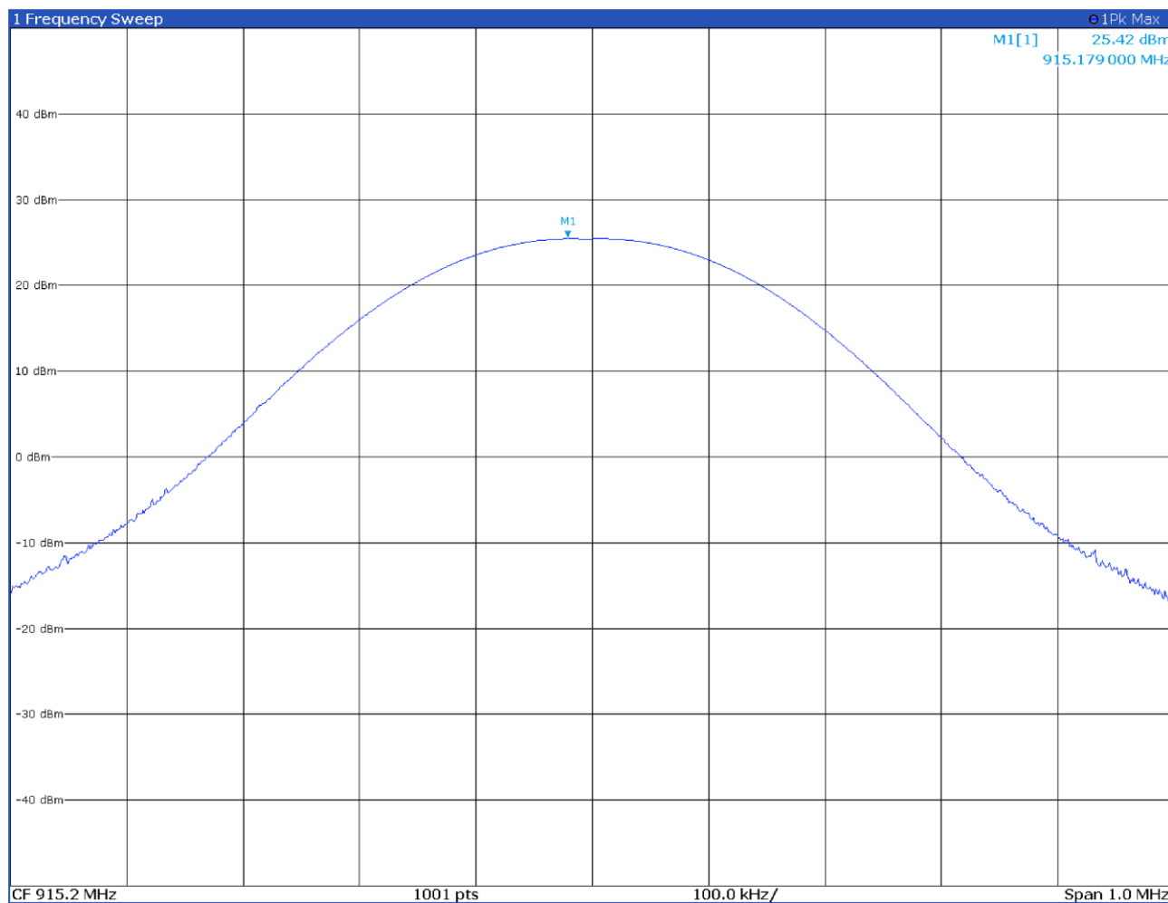
Figure 8.6-1: Output power on low channel
