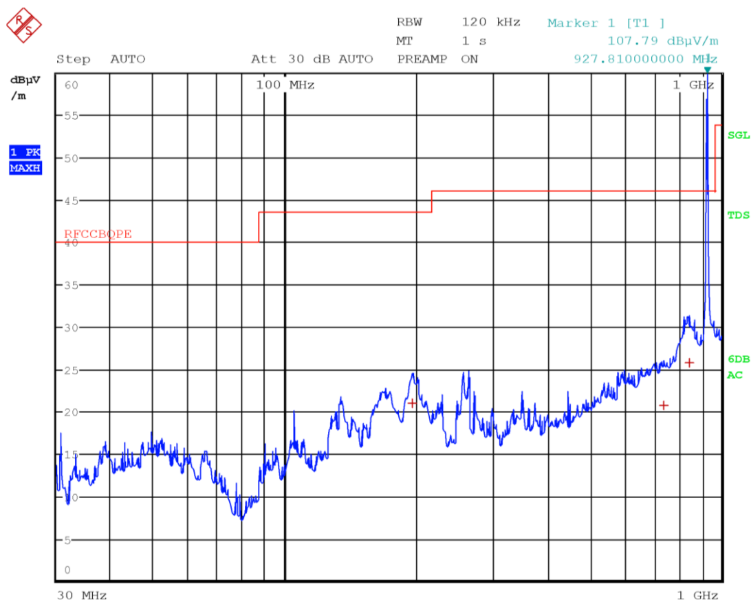
Figure 8.7-13: Radiated spurious emissions on high channel with antenna in horizontal polarization – Frequency range 30 to 1000 MHz
