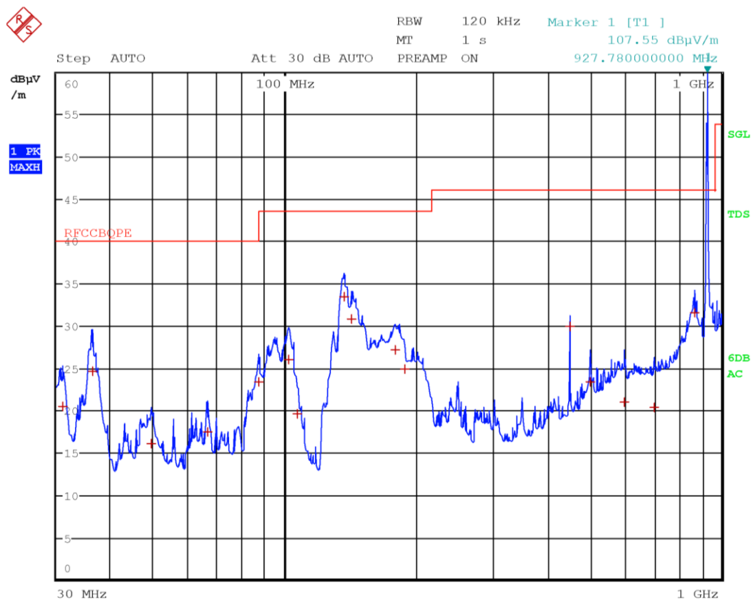
Figure 8.7-14: Radiated spurious emissions on high channel with antenna in vertical polarization – Frequency range 30 to 1000 MHz
