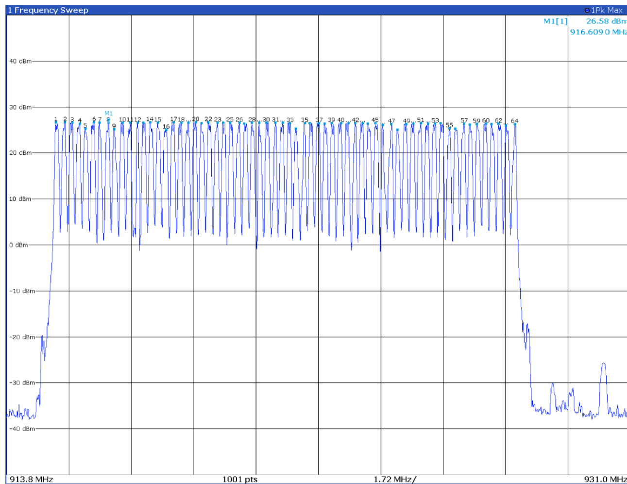
Figure 8.5-8: Number of hopping channels
