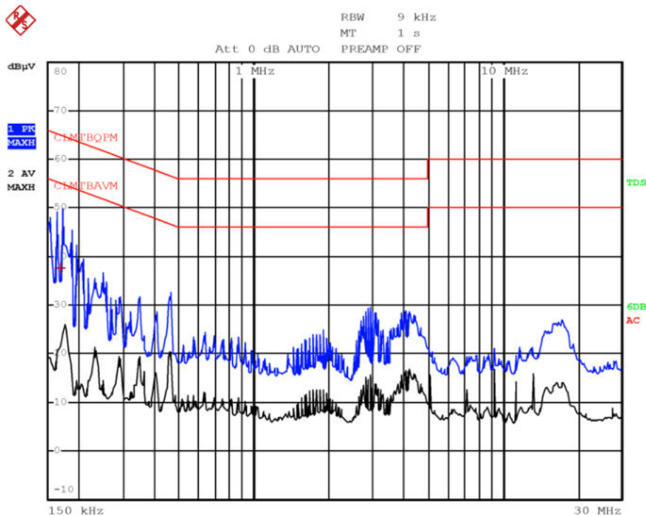
Plot 8.4-7: Conducted emissions on phase line 3, 220V 60Hz
