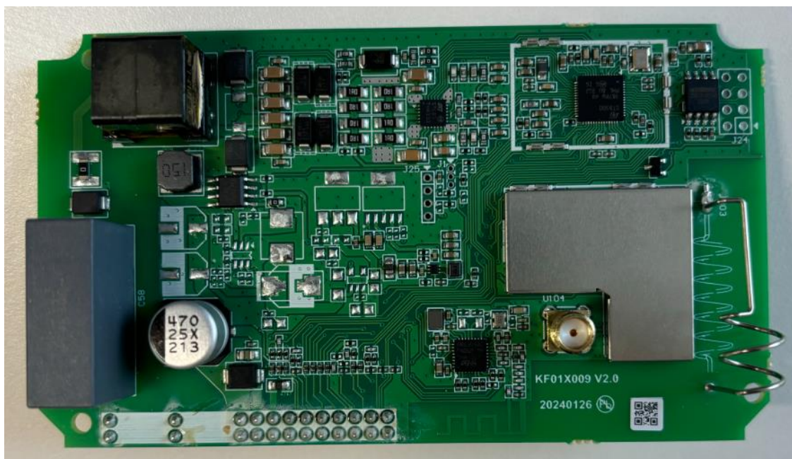
Figure 5 - GLOBYSGNG3 communication module top view
