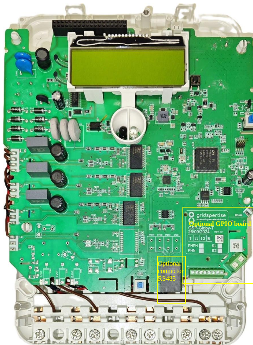
Figure 1- GLOBYSGNG3 top open view
