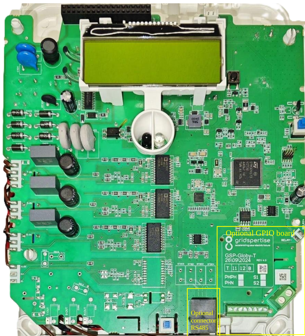
Figure 3 - GLOBYSGNG3 top PCB open view
