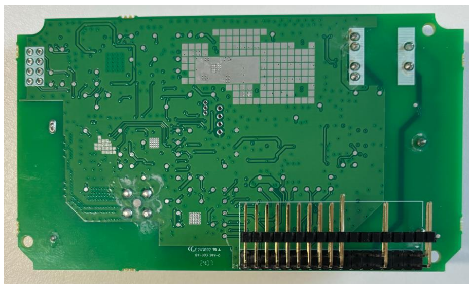
Figure 8 - GLOBYSGNG3 communication module bottom view
