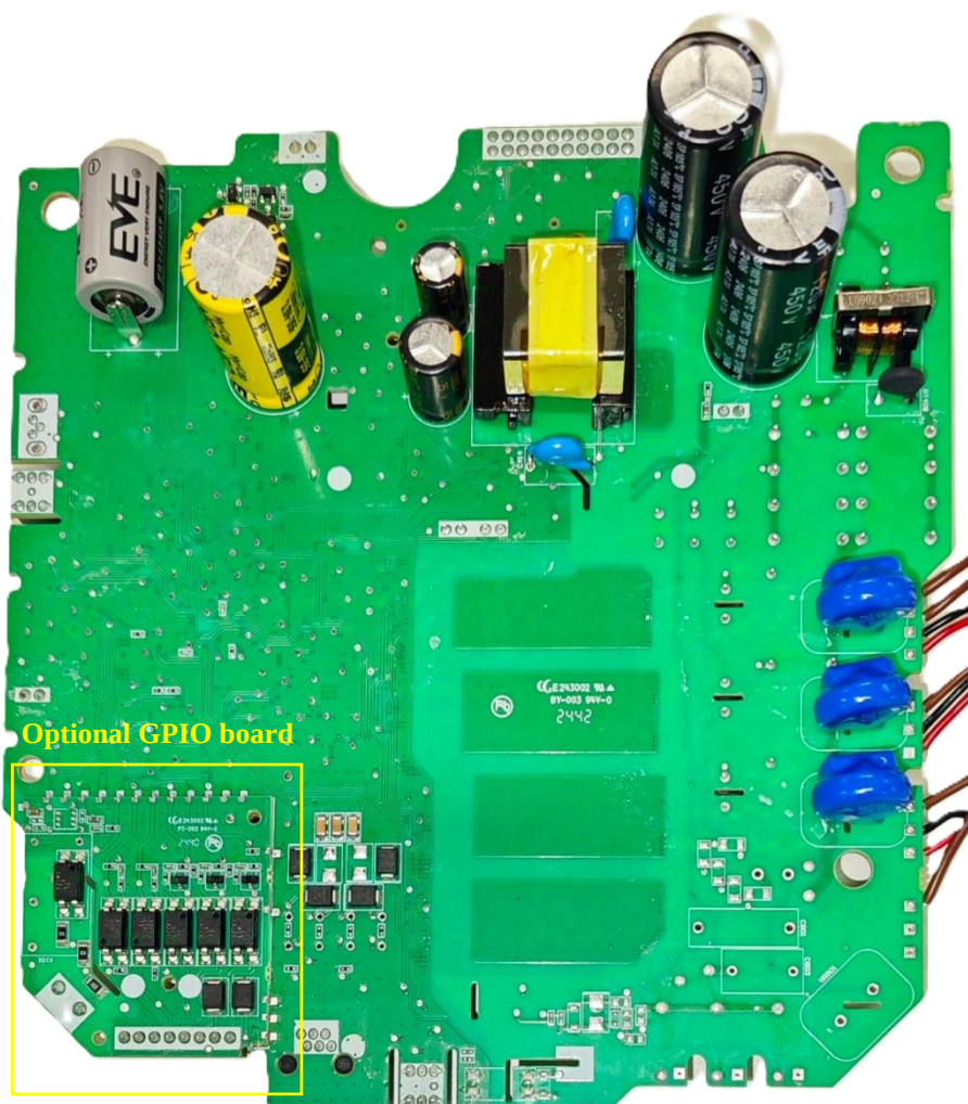
Figure 4 - GLOBYSGNG3 bottom PCB view
