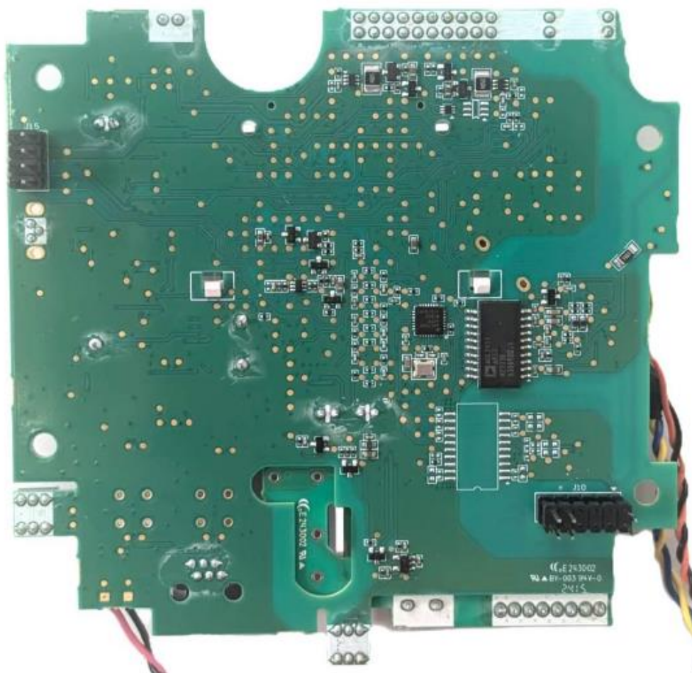
Figure 6 - GLOBYMGNG3 main PCB bottom view full version
