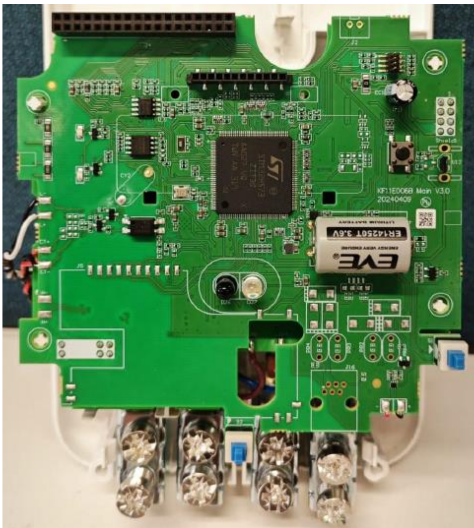
Figure 7 - GLOBYMGNG3 main PCB top view basic version
