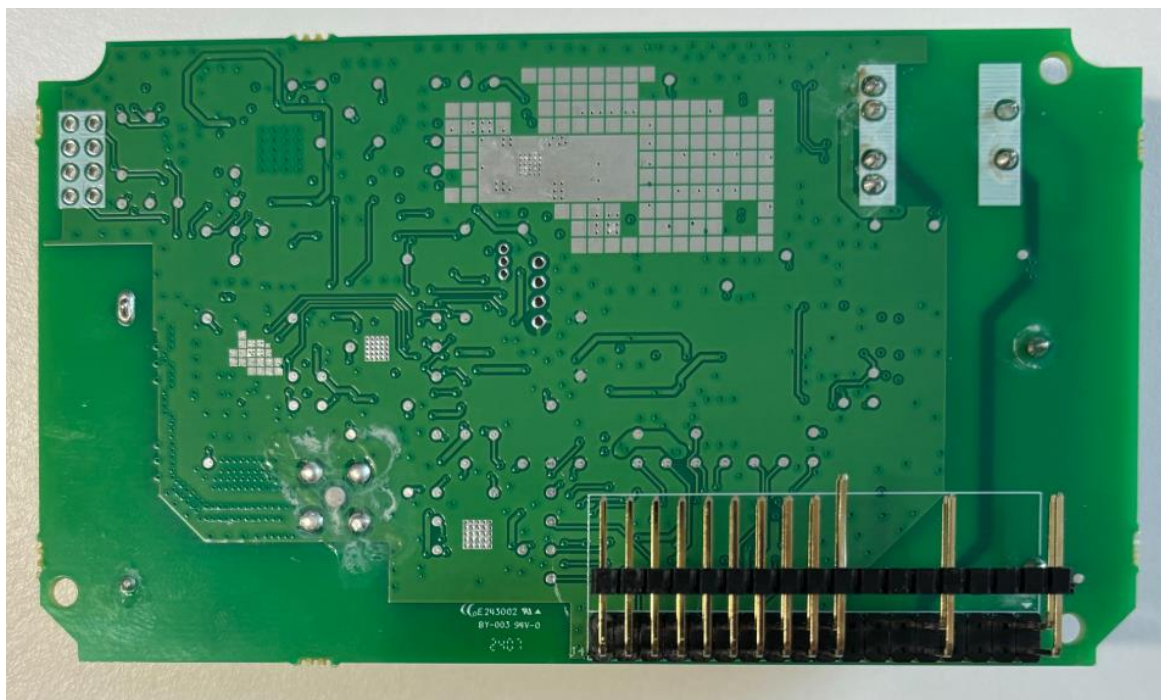
Figure 12 - GLOBYMGNG3 communication module bottom view
