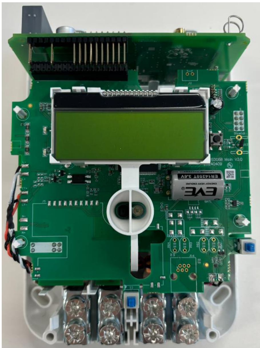
Figure 2 - GLOBYMGNG3 top open view basic version
