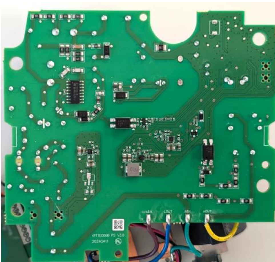
Figure 9 - Power Supply (PSU) PCB top view full and basic version
