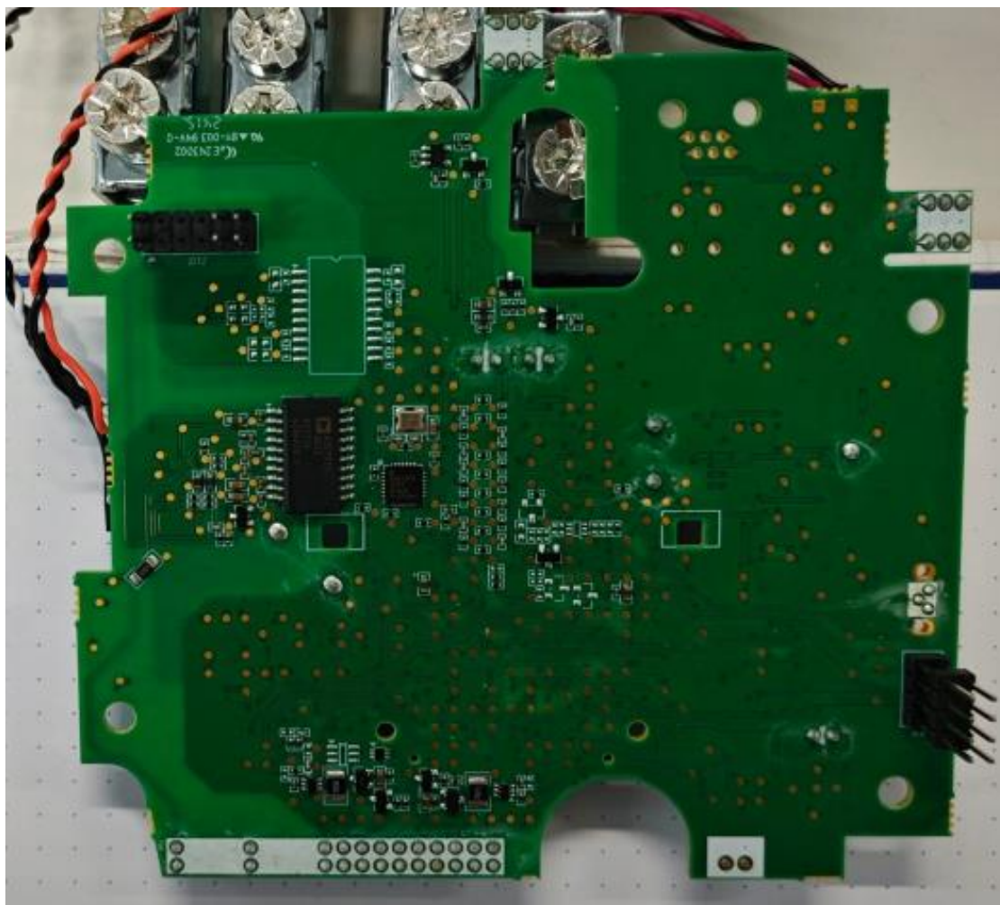
Figure 8 - GLOBYMGNG3 main PCB bottom view basic version
