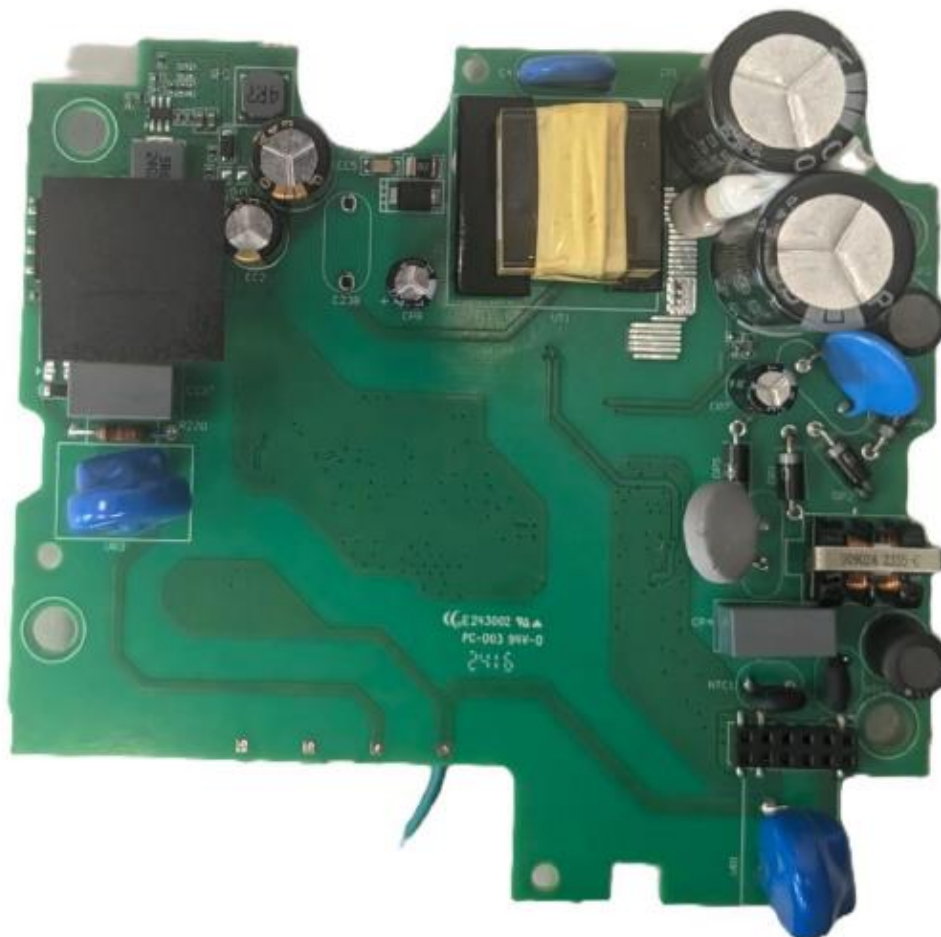
Figure 10 - Power Supply (PSU) PCB bottom view full and basic version
