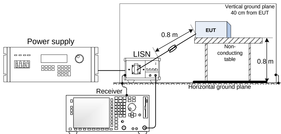
Figure 5.5-3: Conducted testing
