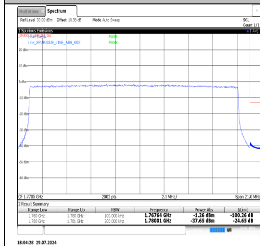
Band66-20MHz-16QAM-132572-100RB#0- PASS
