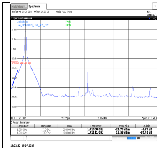
Band66-20MHz-16QAM-132072-1RB#99- PASS
