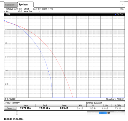
Band66-15MHz-16QAM-132322-75RB#0-PASS
