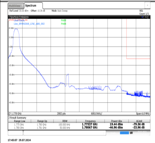
Band66-5MHz-QPSK-132647-1RB#24-PASS
