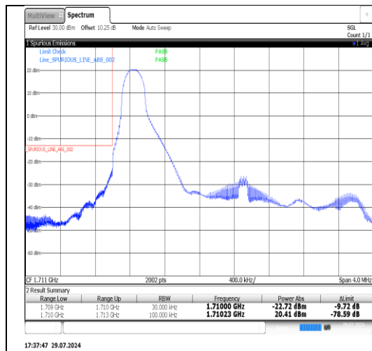
Band66-3MHz-QPSK-131987-1RB#14-PASS
