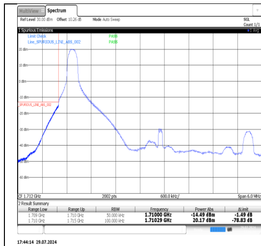
Band66-5MHz-QPSK-131997-1RB#24-PASS
