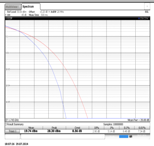
Band66-20MHz-16QAM-132322-100RB#0-PASS
