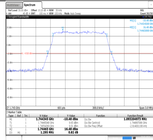
Band66-3MHz-QPSK-132322-15RB#0-PASS
