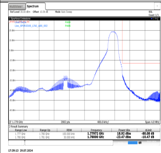
Band66-5MHz-QPSK-131997-25RB#0-PASS
