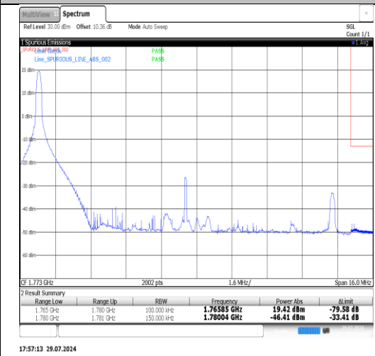
Band66-15MHz-QPSK-132597-1RB#74-PASS
