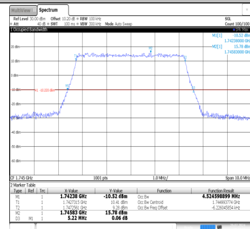
Band66-5MHz-QPSK-132322-25RB#0-PASS
