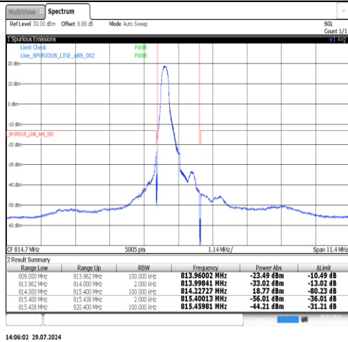
Band26(814-824)-1.4MHz-QPSK-26697- 1RB#5-PASS
