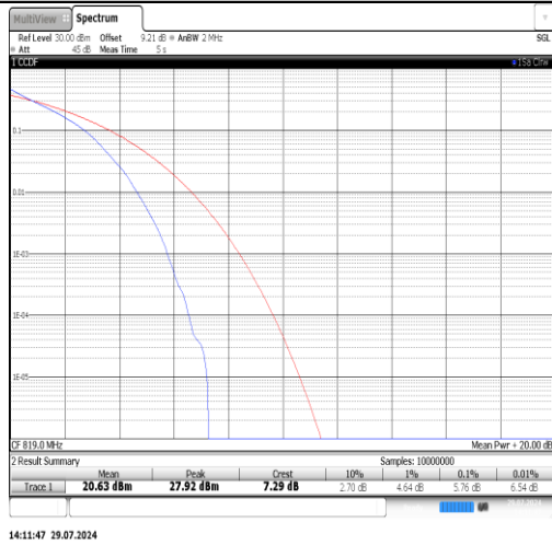
Band26(814-824)-5MHz-QPSK-26740-25RB#0-PASS
