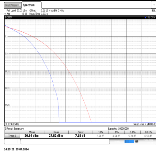
Band26(814-824)-10MHz-QPSK-26740-50RB#0-PASS
