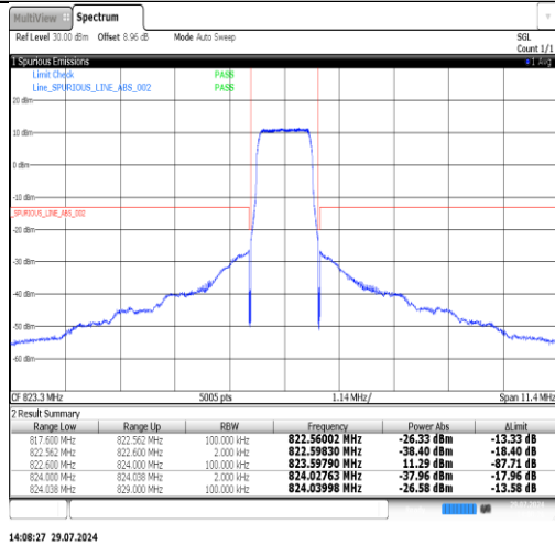
Band26(814-824)-1.4MHz-QPSK-26783- 6RB#0-PASS
