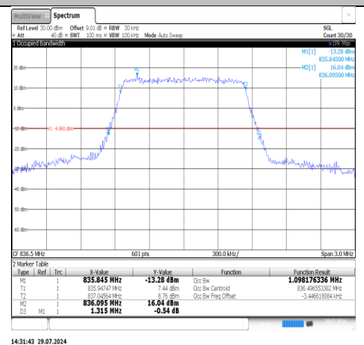
Band26(824-849)-3MHz-16QAM-26915-15RB#0-PASS
