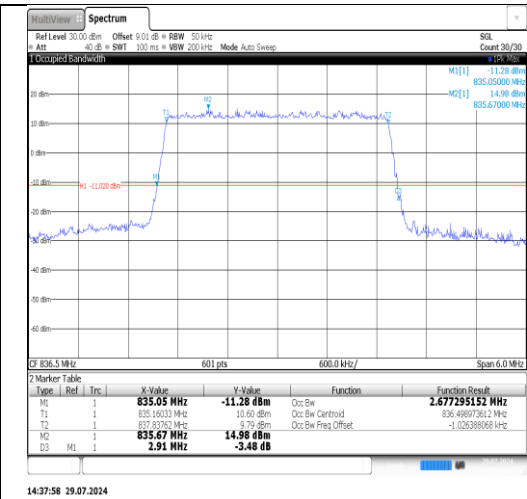
Band26(824-849)-5MHz-16QAM-26915-25RB#0-PASS
