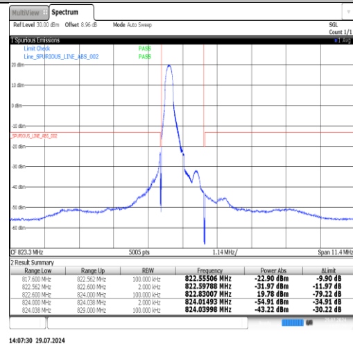
Band26(814-824)-1.4MHz-QPSK-26783- 1RB#5-PASS
