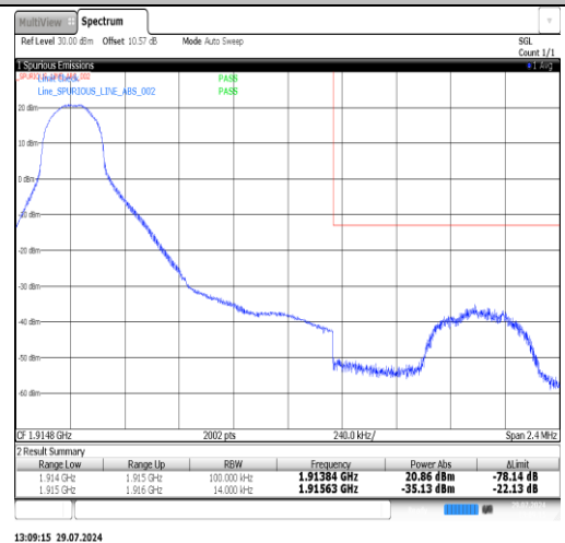
Band25-1.4MHz-QPSK-26683-1RB#5-PASS
