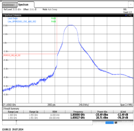
Band25-1.4MHz-QPSK-26047-1RB#5-PASS
