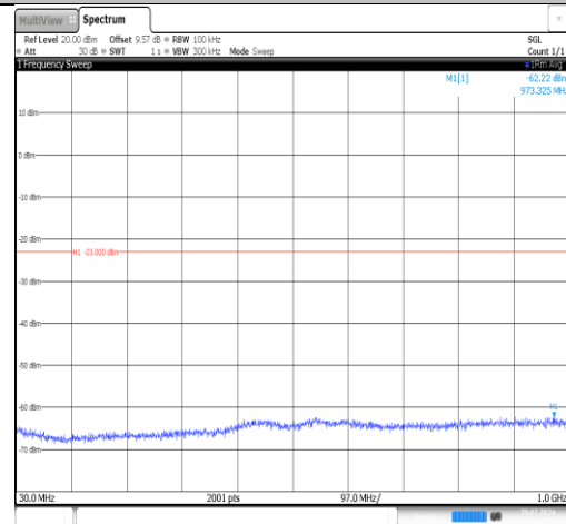
Band25-1.4MHz-16QAM-26047-1RB#0- 30~1000-PASS
