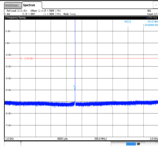
Band25-1.4MHz-QPSK-26683-1RB#0- 1000~3000-PASS
