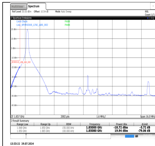
Band25-15MHz-QPSK-26115-1RB#74-PASS
