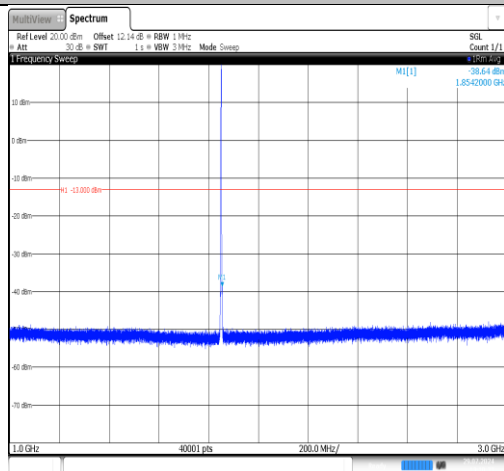
Band25-1.4MHz-16QAM-26047-1RB#0- 1000~3000-PASS
