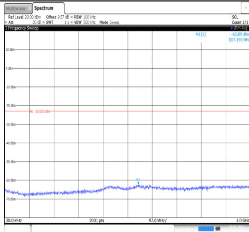
Band25-1.4MHz-QPSK-26683-1RB#0- 30~1000-PASS
