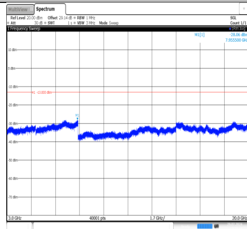
Band25-1.4MHz-16QAM-26047-1RB#0- 3000~20000-PASS
