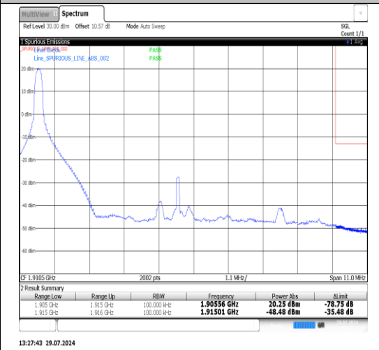
Band25-10MHz-QPSK-26640-1RB#49-PASS
