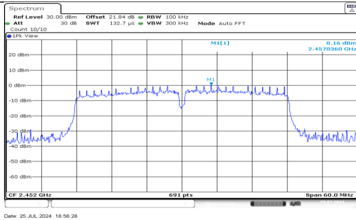
11N40SISO_Ant1_2452_0~Reference
