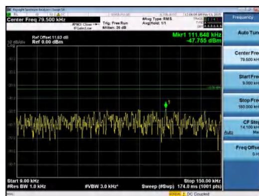
Band5-5MHz-16QAM-20625-25RB#0-0.009~0.1 5-PASS
