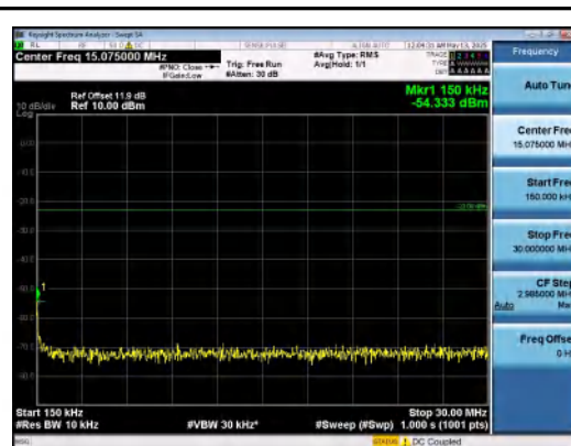
Band5-5MHz-16QAM-20625-1RB#24-0.15~30-P ASS
