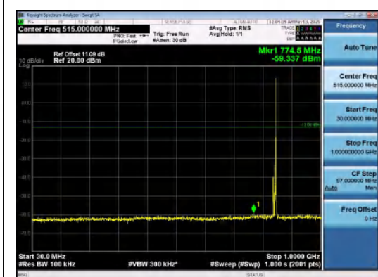
Band5-5MHz-16QAM-20625-1RB#24-30~1000-P ASS
