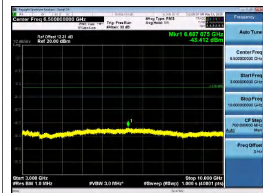
Band5-5MHz-16QAM-20625-1RB#24-3000~100 00-PASS
