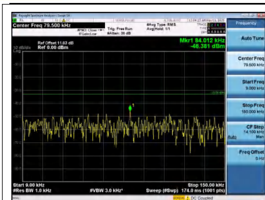
Band5-5MHz-16QAM-20625-1RB#24-0.009~0.1 5-PASS
