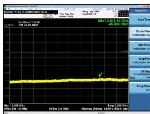
Band5-5MHz-16QAM-20625-1RB#24-1000~300 0-PASS
