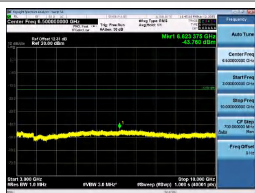
Band5-1.4MHz-QPSK-20407-1RB#0-3000~1000 0-PASS
