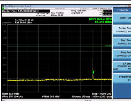
Band5-1.4MHz-QPSK-20407-1RB#5-30~1000-P ASS
