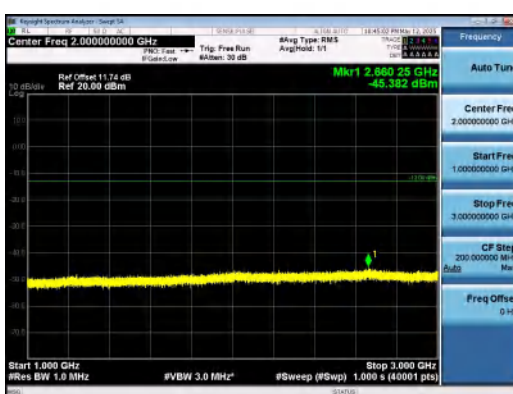
Band5-1.4MHz-QPSK-20407-1RB#0-1000~3000 -PASS
