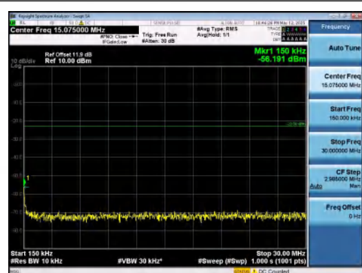
Band5-1.4MHz-QPSK-20407-1RB#5-0.15~30-P ASS
