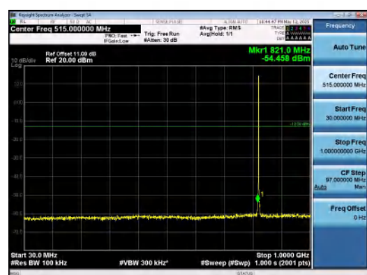
Band5-1.4MHz-QPSK-20407-1RB#0-30~1000-P ASS
