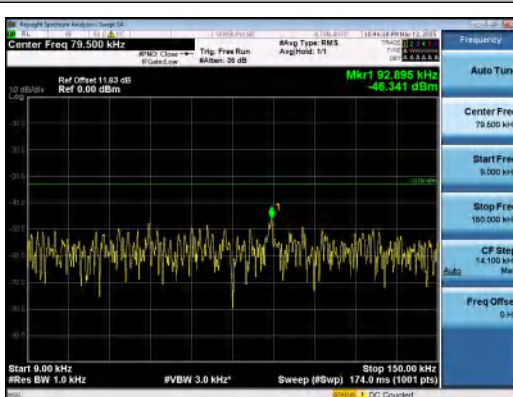
Band5-1.4MHz-QPSK-20407-1RB#5-0.009~0.15 -PASS
