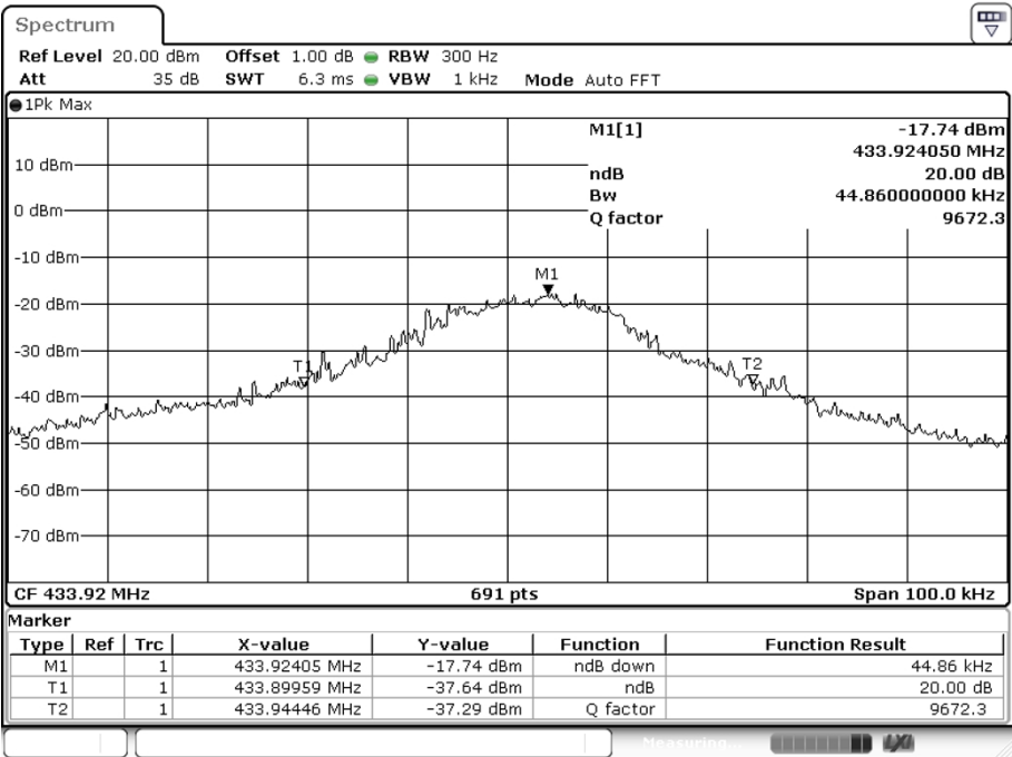
20dB Bandwidth
