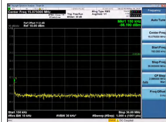
Band12-5MHz-QPSK-23095-1RB#24-0.15~30-P ASS
