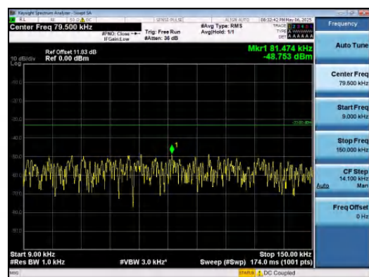
Band12-5MHz-QPSK-23095-1RB#24-0.009~0.1 5-PASS
