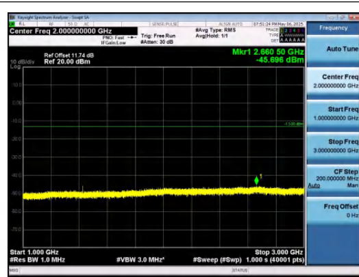
Band12-3MHz-QPSK-23165-1RB#0-1000~3000- PASS
