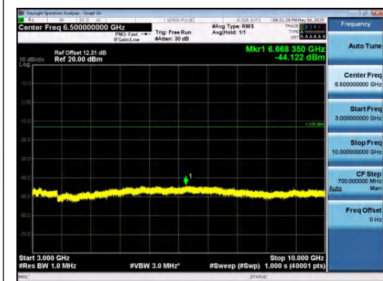
Band12-5MHz-QPSK-23095-1RB#0-3000~1000 0-PASS
