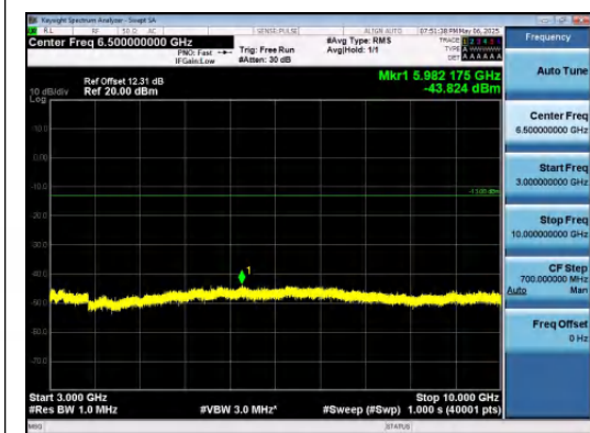
Band12-3MHz-QPSK-23165-1RB#0-3000~1000 0-PASS
