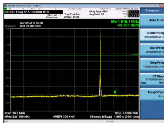
Band12-5MHz-QPSK-23095-1RB#24-30~1000-P ASS
