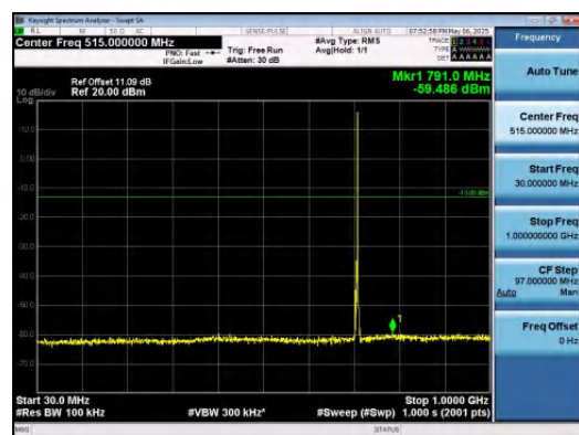
Band12-3MHz-QPSK-23165-1RB#14-30~1000-P ASS
