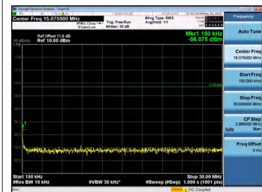
Band12-3MHz-QPSK-23165-1RB#14-0.15~30-P ASS
