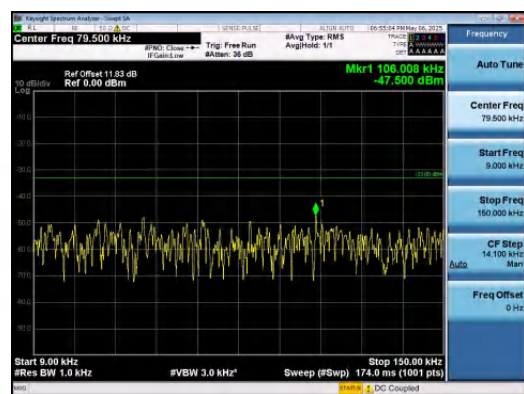
Band12-1.4MHz-QPSK-23017-1RB#5-0.009~0.1 5-PASS
