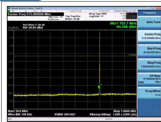
Band12-1.4MHz-QPSK-23095-1RB#0-30~1000-PASS
