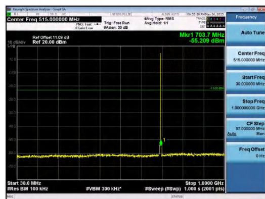
Band12-1.4MHz-QPSK-23017-1RB#5-30~1000- PASS
