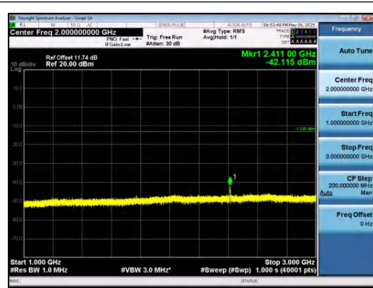
Band12-1.4MHz-QPSK-23017-1RB#0-1000~300 0-PASS
