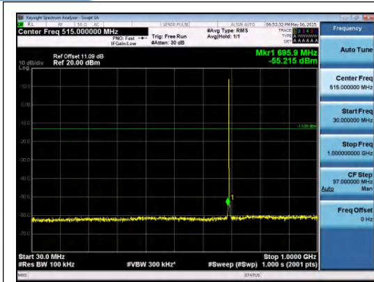
Band12-1.4MHz-QPSK-23017-1RB#0-30~1000-PASS
