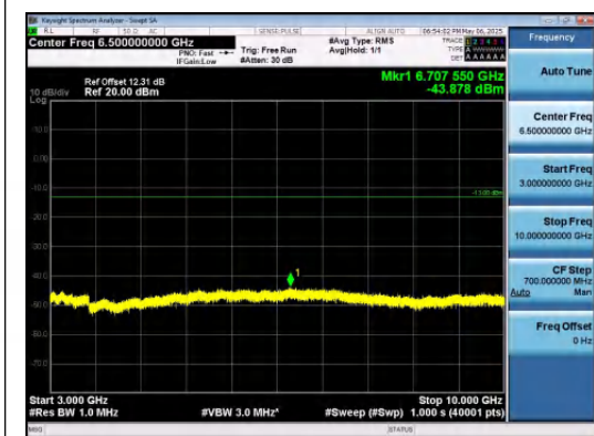
Band12-1.4MHz-QPSK-23017-1RB#0-3000~100 00-PASS
