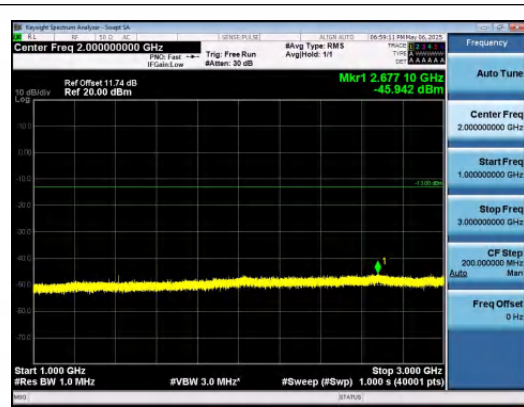
Band12-1.4MHz-QPSK-23095-1RB#0-1000~300 0-PASS
