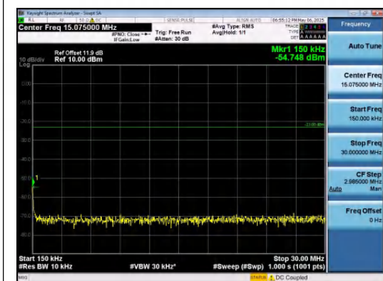
Band12-1.4MHz-QPSK-23017-1RB#5-0.15~30-P ASS
