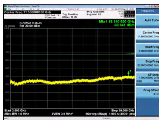
Band2-5MHz-QPSK-18900-1RB#24-3000~2000 0-PASS
