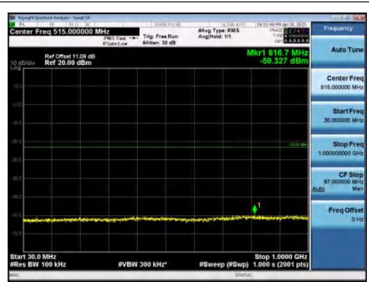
Band2-20MHz-16QAM-18900-1RB#0-30~1000-P ASS
