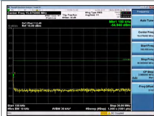
Band2-20MHz-16QAM-18900-1RB#0-0.15~30-P ASS
