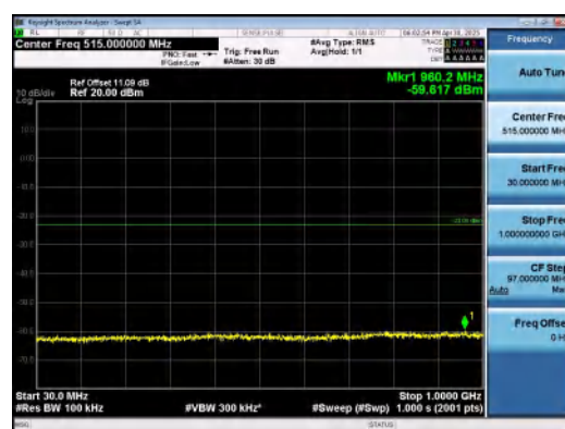
Band2-15MHz-QPSK-18675-1RB#74-30~1000-P ASS
