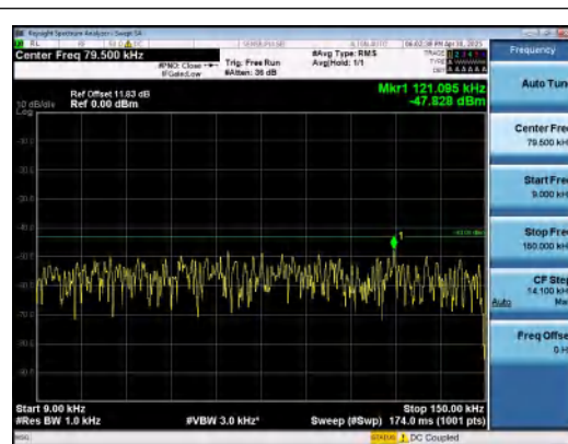
Band2-15MHz-QPSK-18675-1RB#74-0.009~0.1 5-PASS
