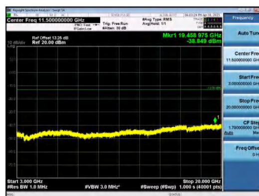
Band2-15MHz-QPSK-18675-1RB#74-3000~200 00-PASS
