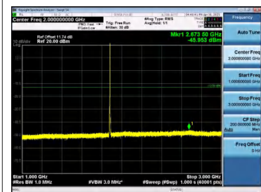
Band2-5MHz-QPSK-18900-1RB#24-1000~3000- PASS
