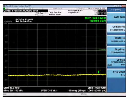
Band2-15MHz-16QAM-18675-1RB#0-30~1000-P ASS
