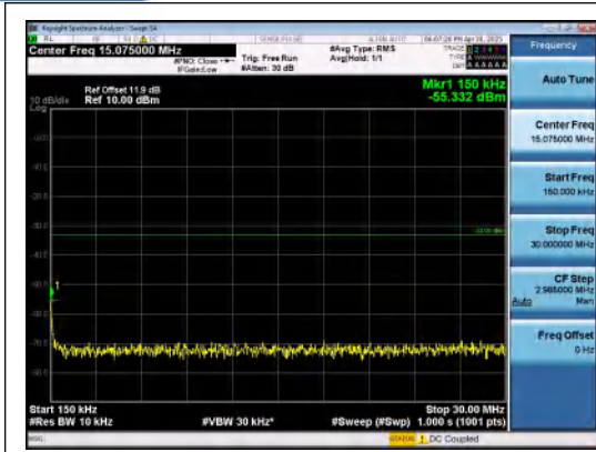
Band2-15MHz-16QAM-18900-1RB#0-0.15~30-P ASS
