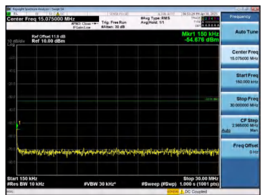
Band2-20MHz-16QAM-18900-1RB#99-0.15~30-PASS
