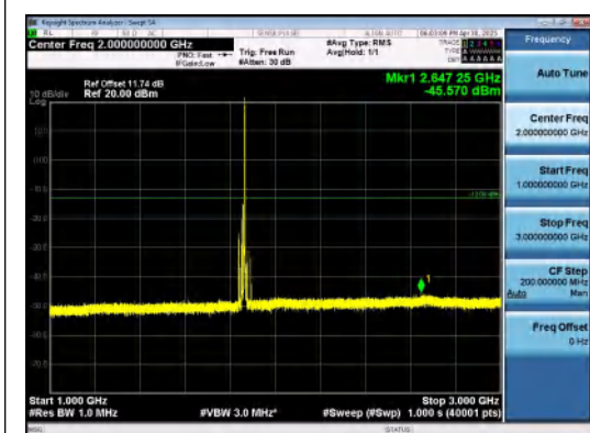
Band2-15MHz-QPSK-18675-1RB#74-1000~300 0-PASS
