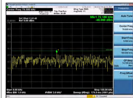
Band2-20MHz-16QAM-18900-1RB#99-0.009~0. 15-PASS
