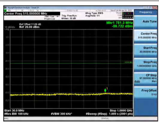
Band2-15MHz-16QAM-18900-1RB#0-30~1000-P ASS
