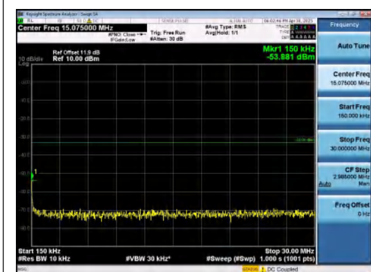
Band2-15MHz-QPSK-18675-1RB#74-0.15~30-P ASS
