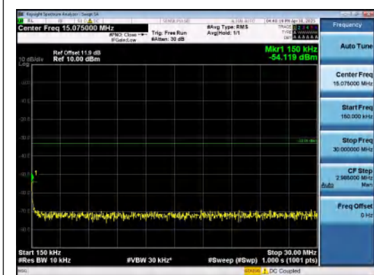
Band2-5MHz-QPSK-18900-1RB#24-0.15~30-PA- SS
