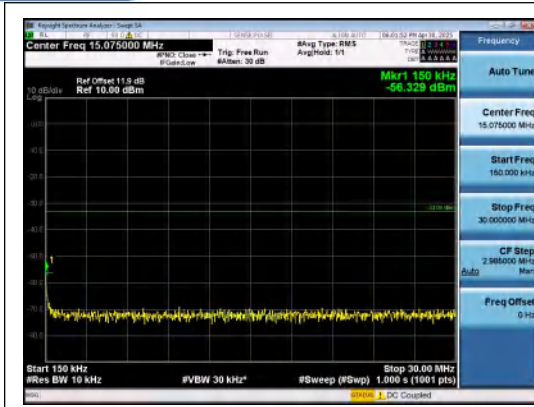
Band2-15MHz-16QAM-18675-1RB#0-0.15~30-P ASS
