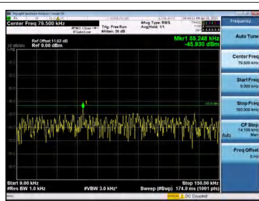
Band2-5MHz-QPSK-18900-1RB#24-0.009~0.15- PASS
