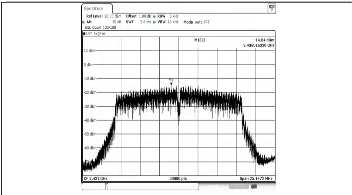
11G-Ant1-2437-PASS
