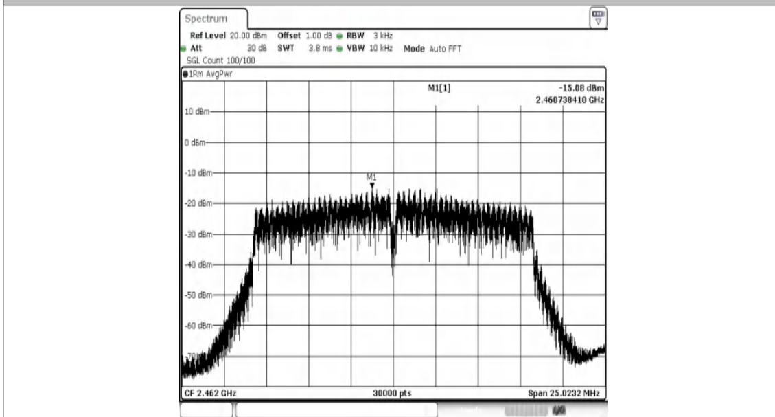
11G-Ant1-2462-PASS
