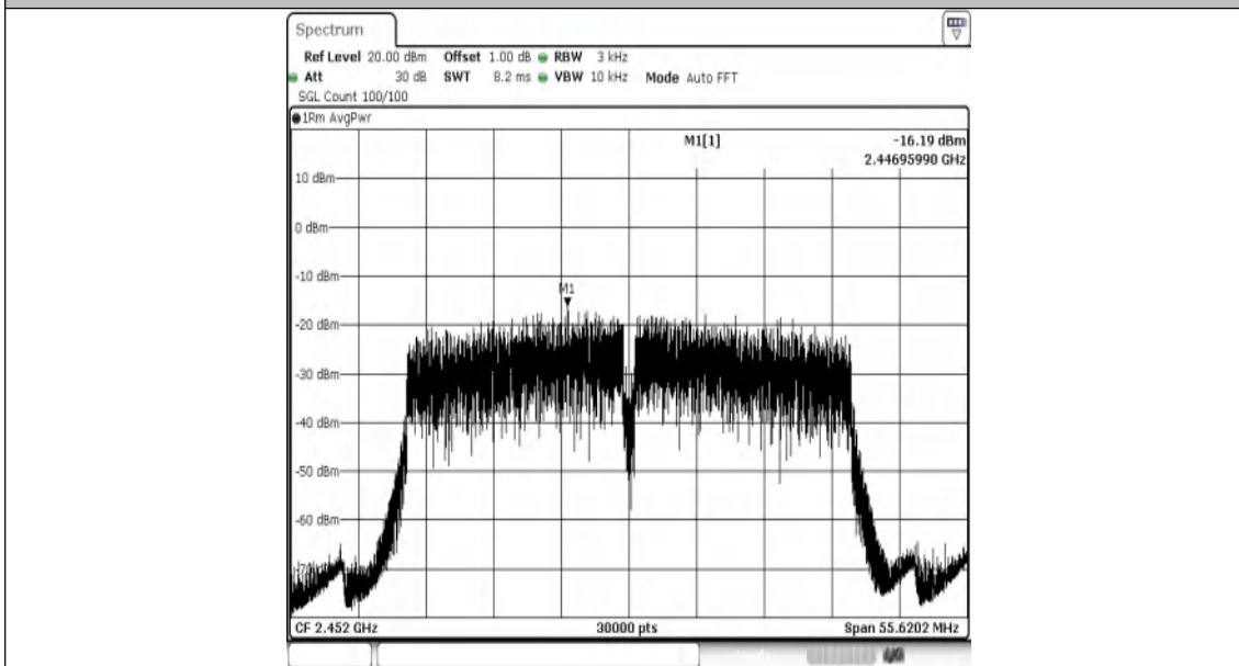
11N40SISO-Ant1-2452-PASS
