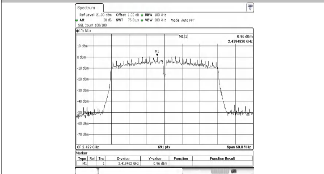
11N40SISO-Ant1-2422-0~Reference-PASS
