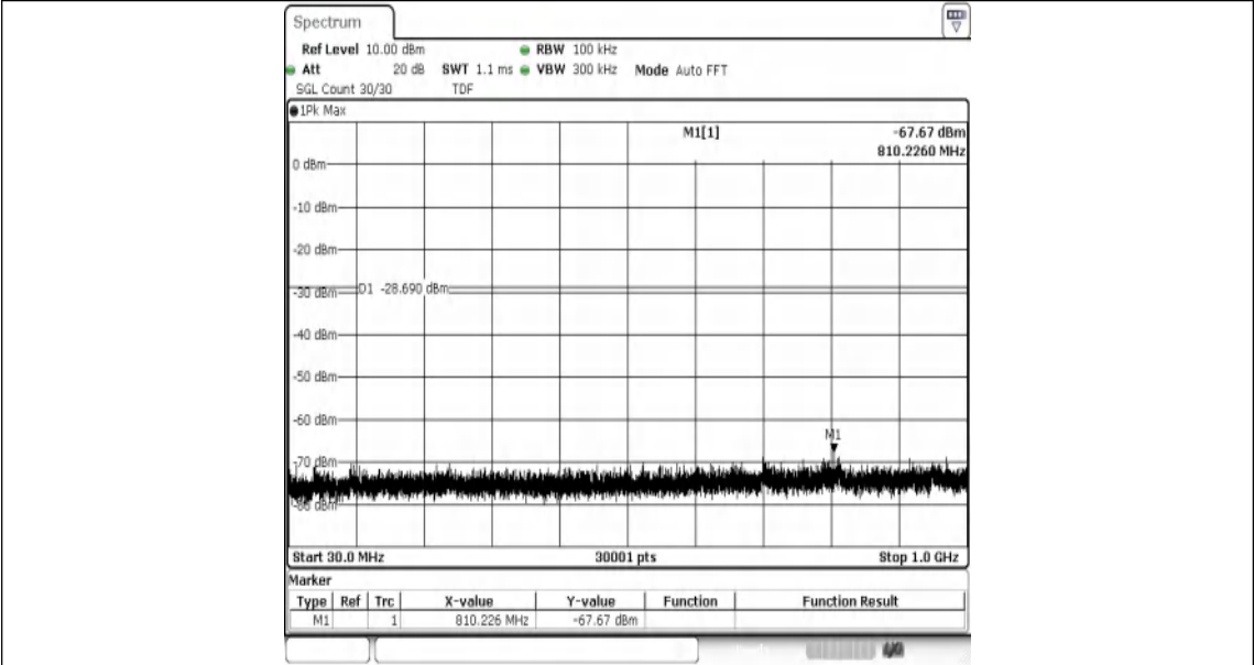
11N40SISO-Ant1-2437-30~1000-PASS
