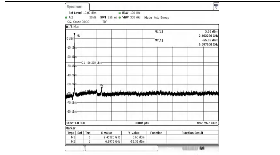
11N20SISO-Ant1-2462-1000~26500-PASS
