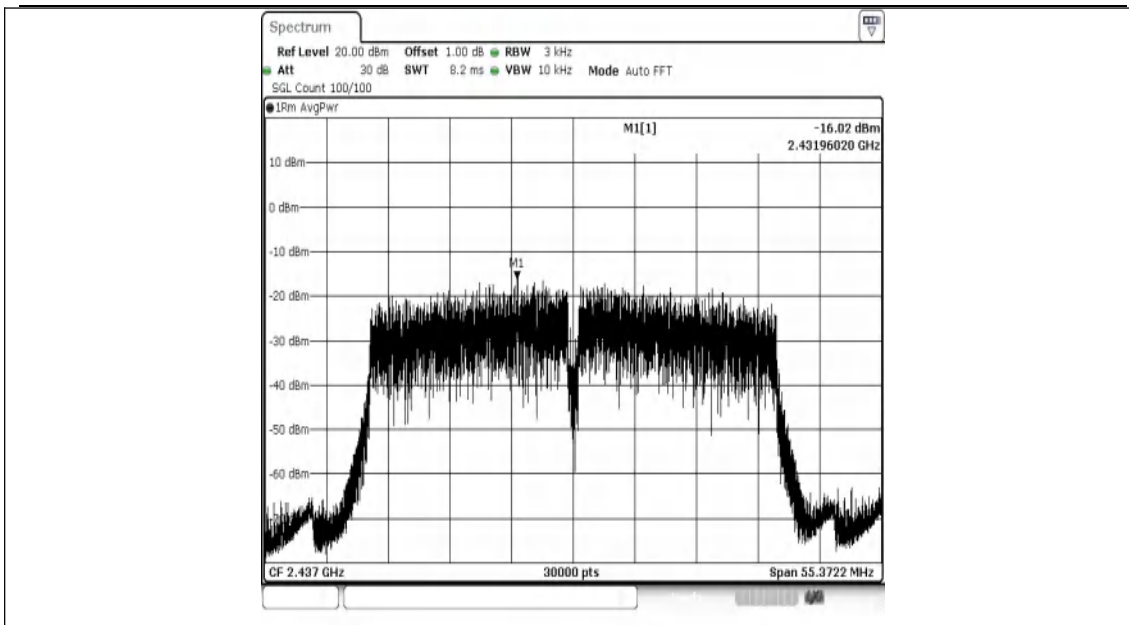
11N40SISO-Ant1-2437-PASS
