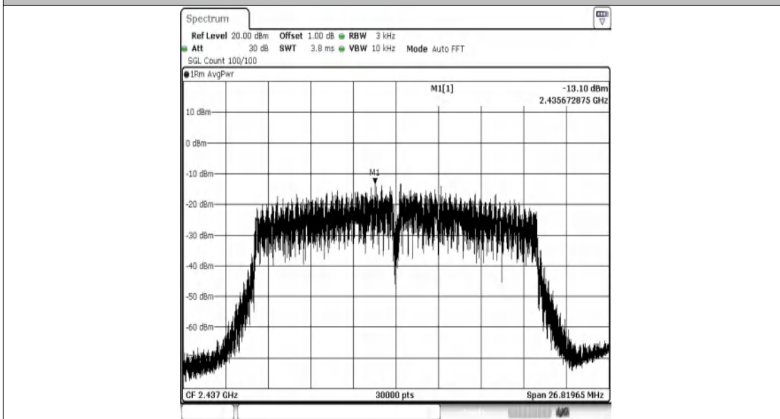
11N20SISO-Ant1-2437-PASS
