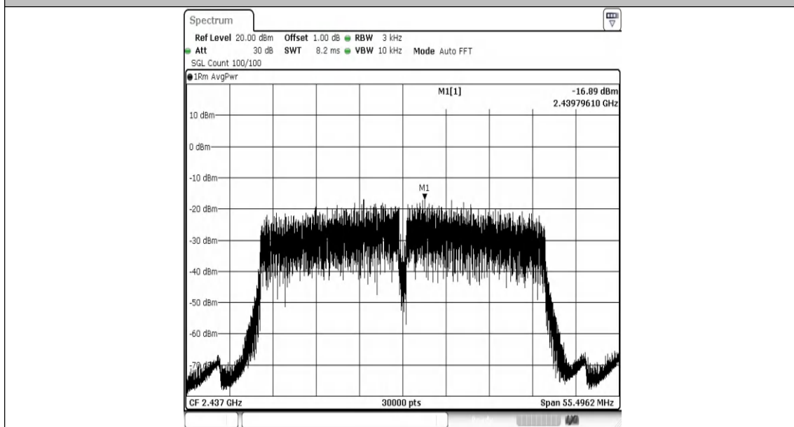
11N40SISO-Ant1-2437-PASS
