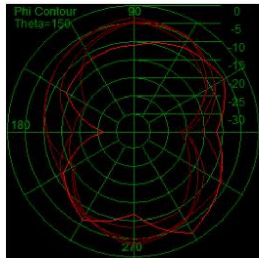
Passive -Freq2480.00MHz
