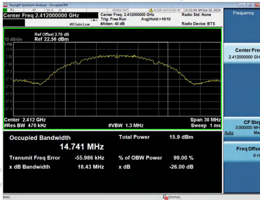
99%_Occupied_Bandwidth_NVNT_ANT1_802_11b_2412
