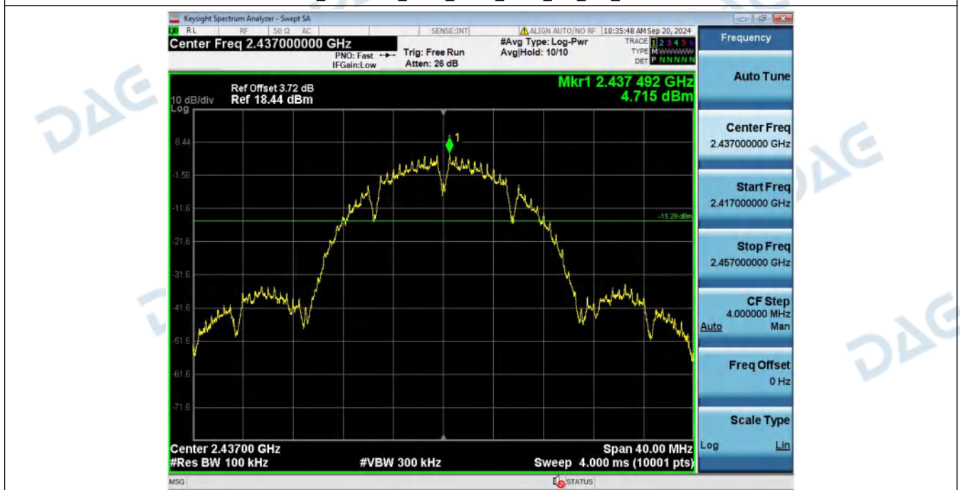
2_Spurious_Emission_NVNT_ANT1_802_11b_2437
