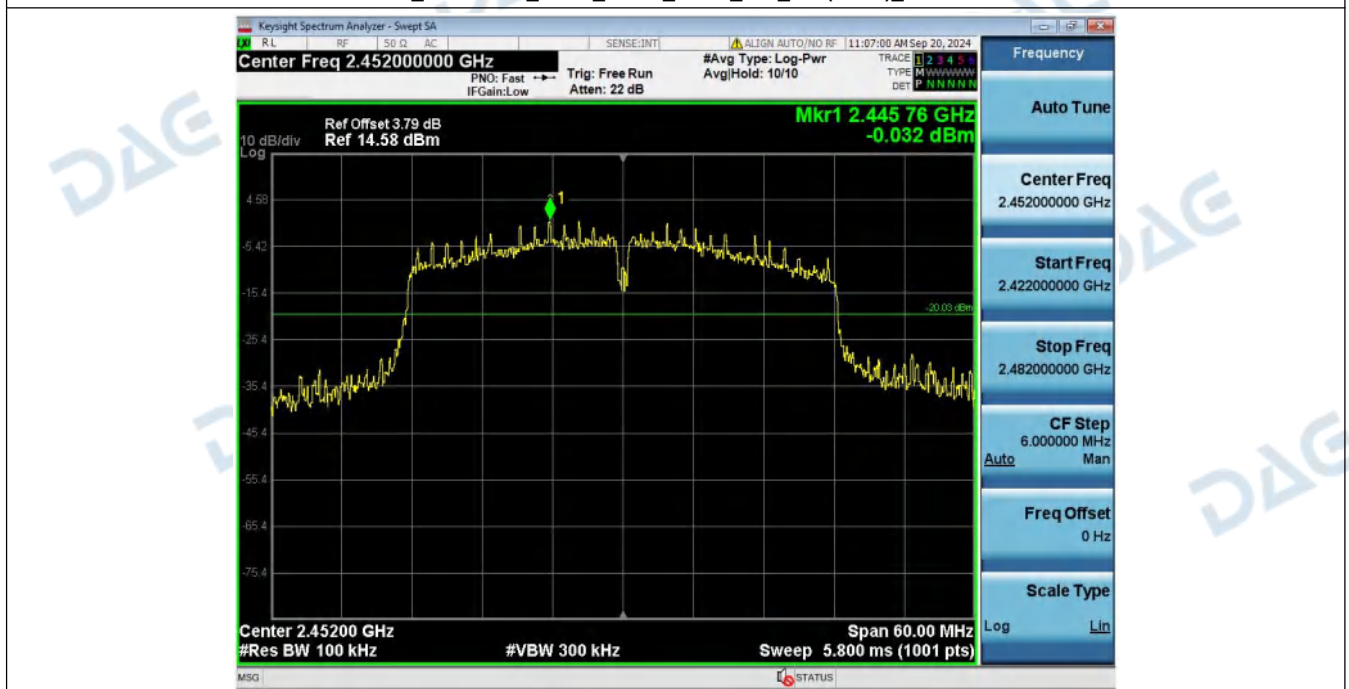
2_Spurious_Emission_NVNT_ANT1_802_11n(HT40)_2452
