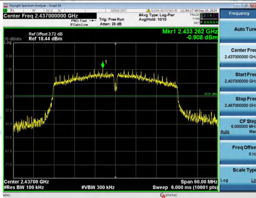
2_Spurious_Emission_NVNT_ANT1_802_11n(HT40)_2437
