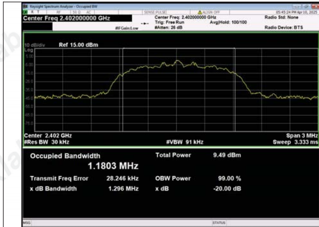
8DPSK_3-DH5_Channel 0
