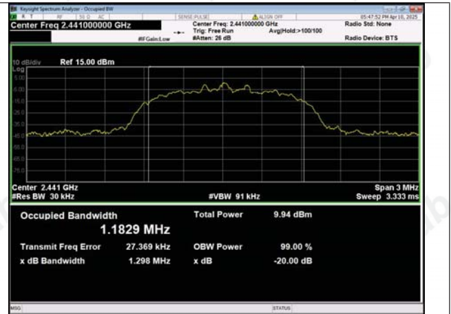
8DPSK_3-DH5_Channel 39
