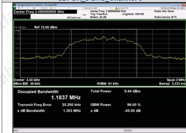
8DPSK_3-DH5_Channel 78
