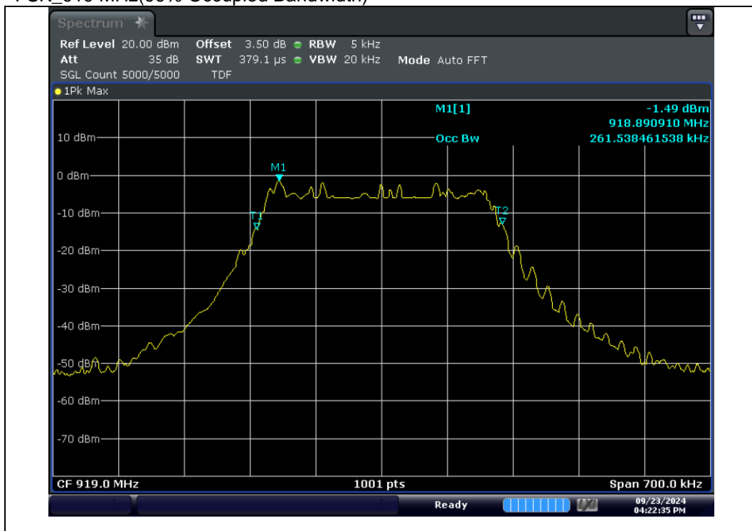
FSK_919 MHz(99% Occupied Bandwidth)
