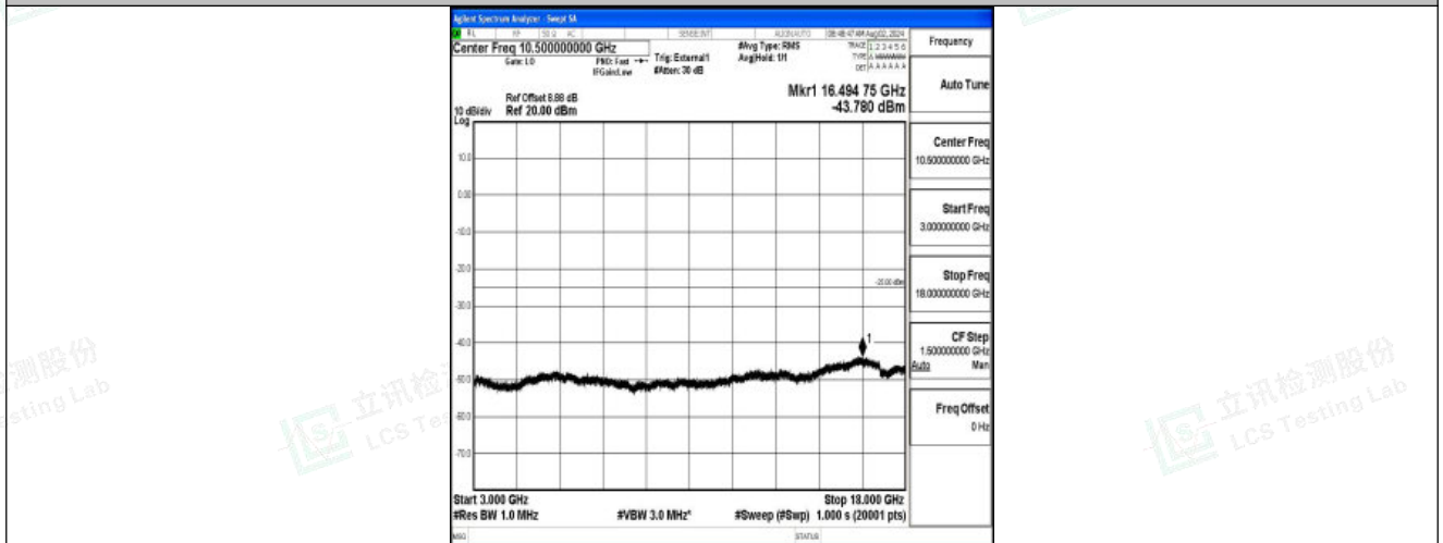
Band41-20MHz-16QAM-39750-1RB#0-3000~18000-PASS
