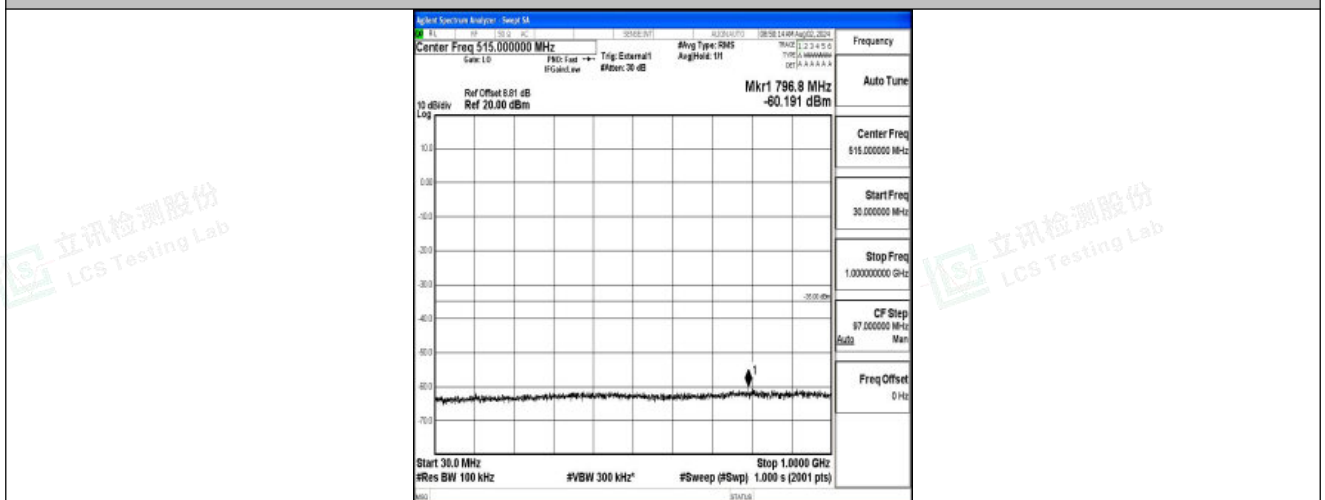
Band41-20MHz-QPSK-40620-1RB#0-30~1000-PASS
