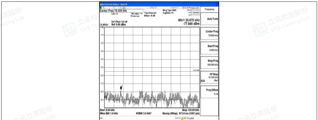
Band41-5MHz-16QAM-41565-1RB#0-0.009~0.15-PASS
