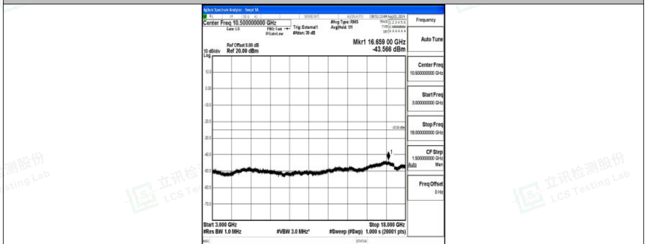
Band41-20MHz-QPSK-40620-1RB#0-3000~18000-PASS
