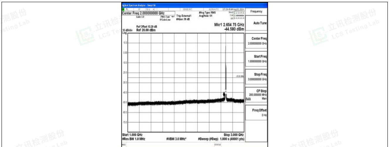
Band41-10MHz-QPSK-41540-1RB#0-1000~3000-PASS
