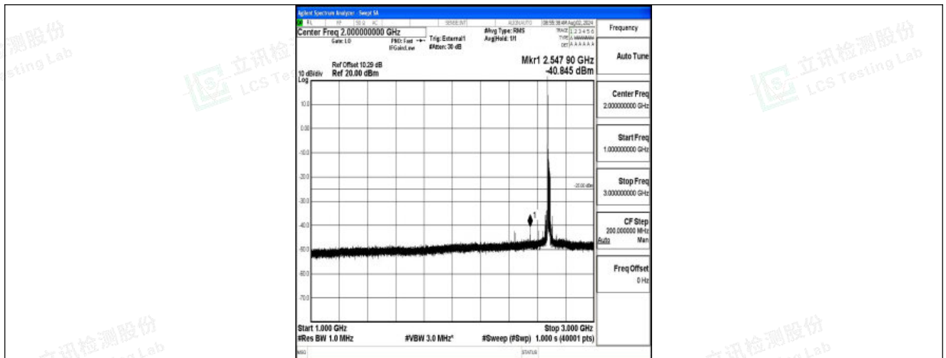
Band41-20MHz-QPSK-41490-1RB#0-1000~3000-PASS
