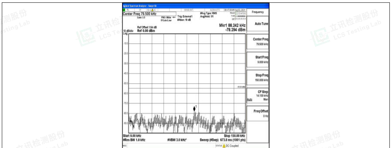
Band41-20MHz-16QAM-39750-1RB#0-0.009~0.15-PASS
