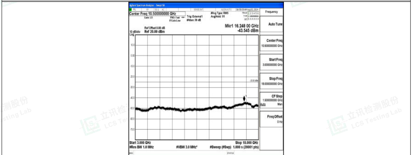
Band41-5MHz-16QAM-41565-1RB#0-3000~18000-PASS
