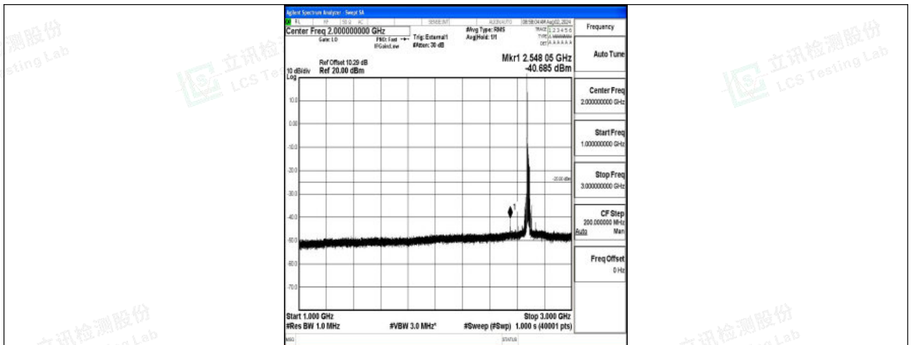
Band41-20MHz-16QAM-41490-1RB#0-1000~3000-PASS
