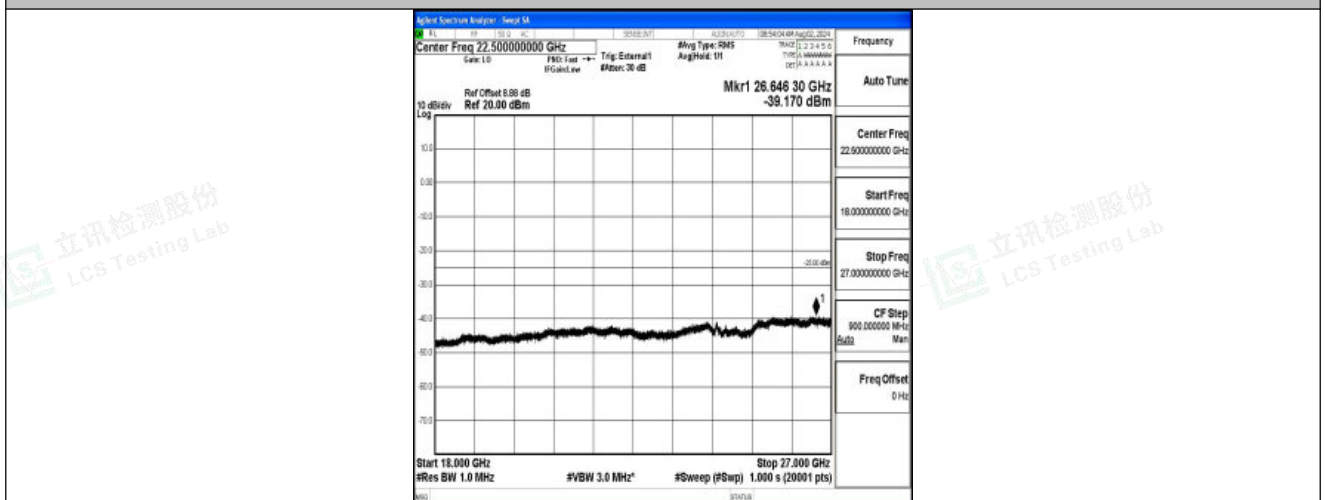
Band41-20MHz-16QAM-40620-1RB#0-18000~27000-PASS
