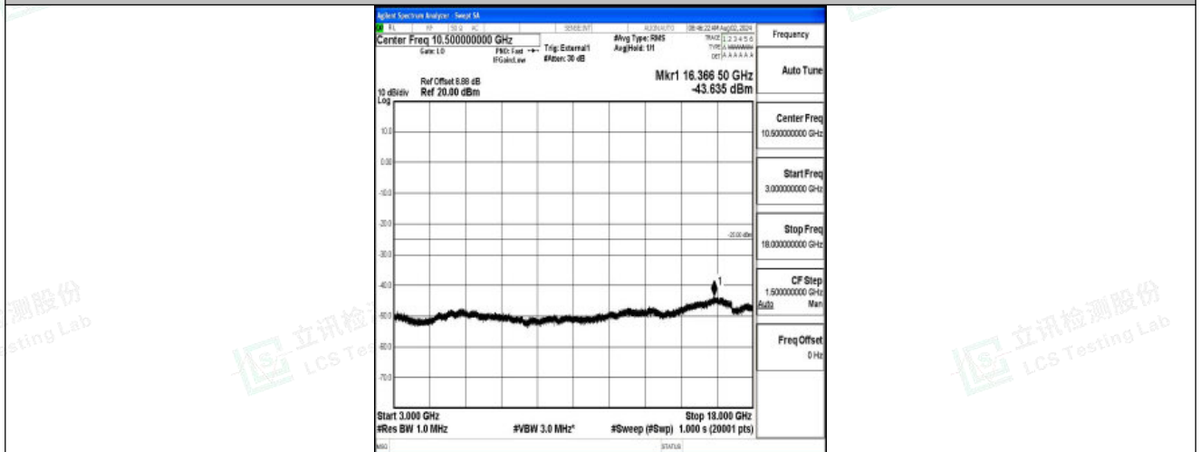
Band41-20MHz-QPSK-39750-1RB#0-3000~18000-PASS
