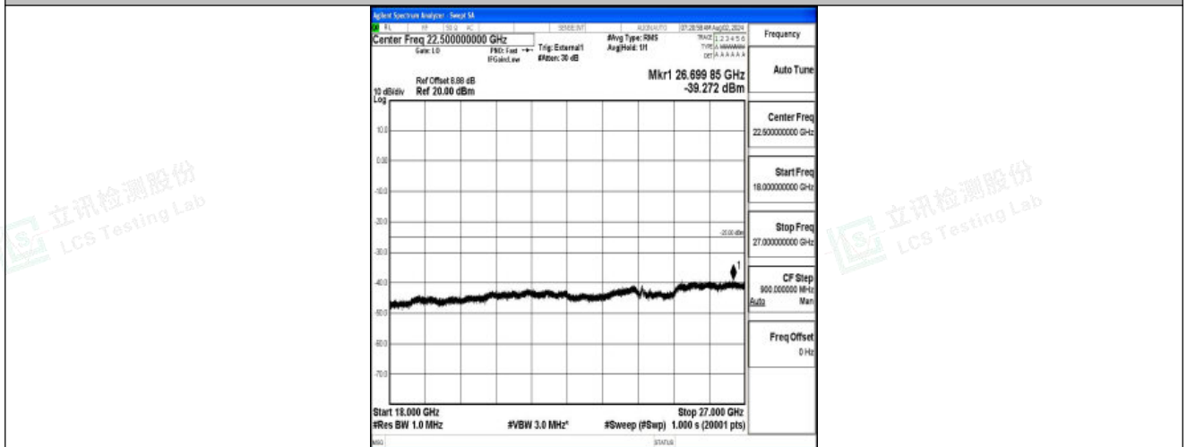
Band41-10MHz-QPSK-39700-1RB#0-18000~27000-PASS
