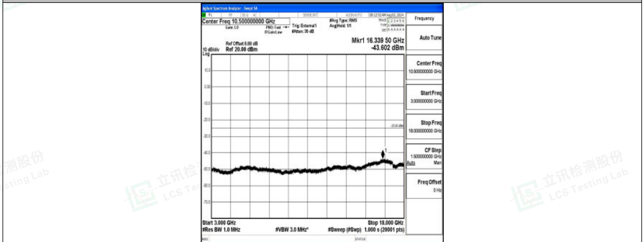
Band41-15MHz-16QAM-41515-1RB#0-3000~18000-PASS
