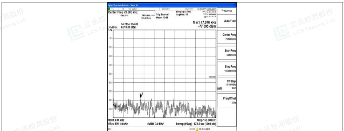
Band41-10MHz-16QAM-40620-1RB#0-0.009~0.15-PASS
