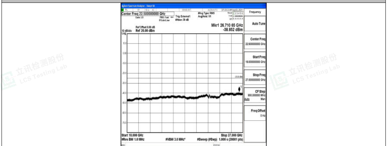
Band41-10MHz-16QAM-39700-1RB#0-18000~27000-PASS
