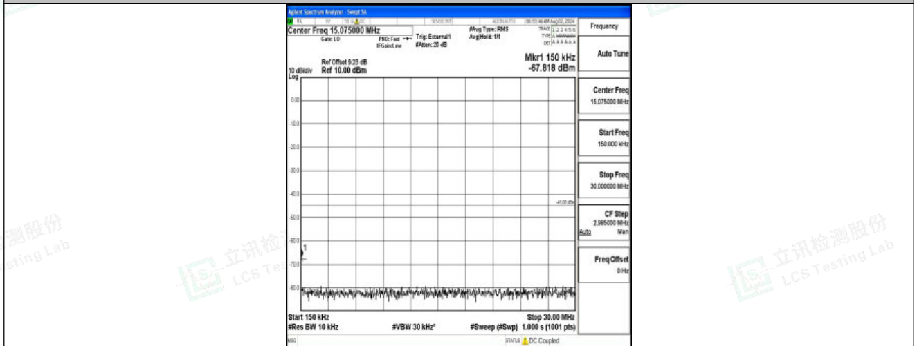
Band41-5MHz-16QAM-41565-1RB#0-0.15~30-PASS
