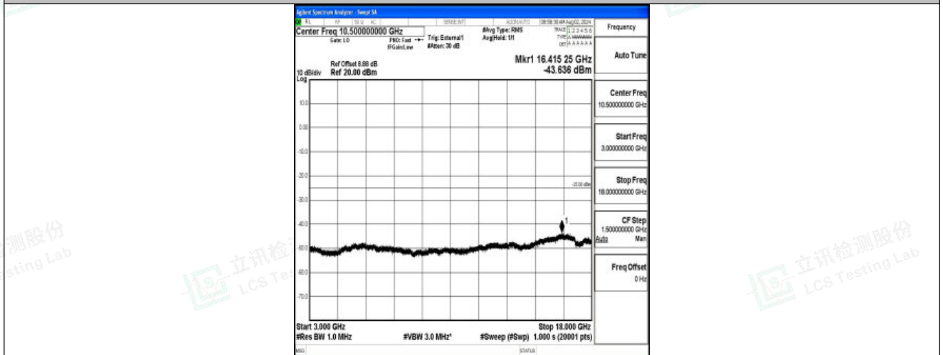
Band41-20MHz-16QAM-41490-1RB#0-3000~18000-PASS
