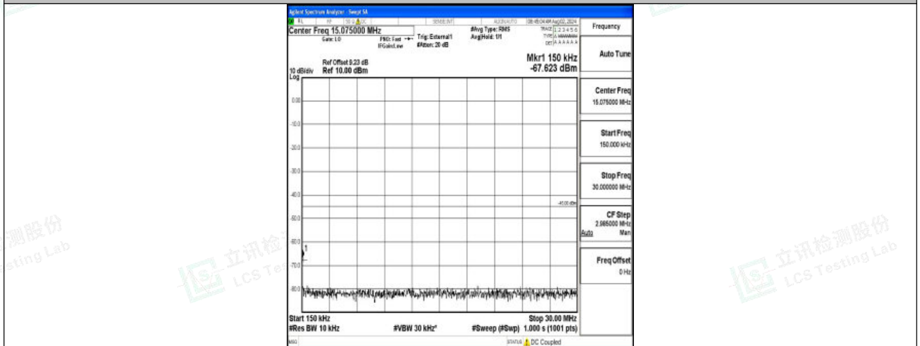
Band41-20MHz-QPSK-39750-1RB#0-0.15~30-PASS
