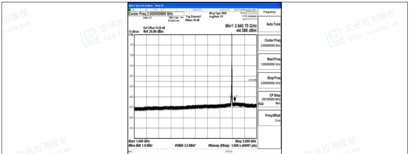
Band41-10MHz-16QAM-40620-1RB#0-1000~3000-PASS
