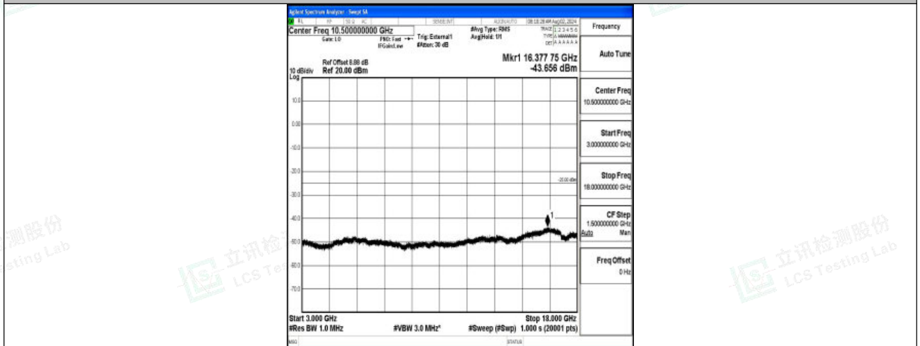
Band41-15MHz-QPSK-41515-1RB#0-3000~18000-PASS
