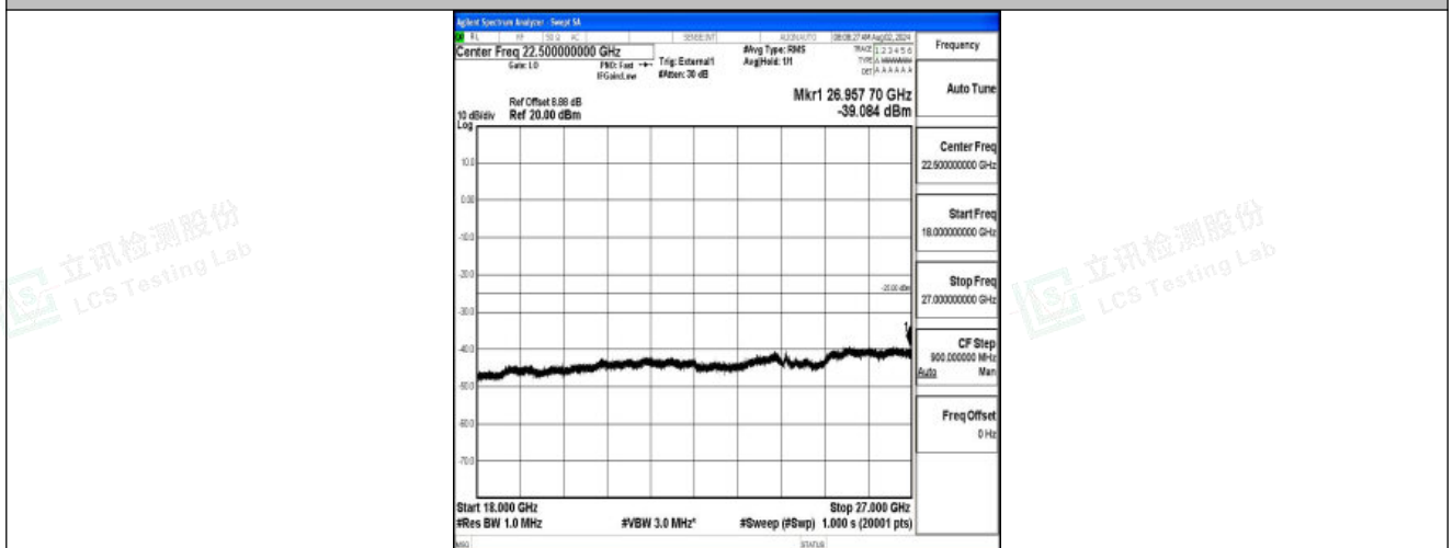
Band41-15MHz-16QAM-40620-1RB#0-18000~27000-PASS
