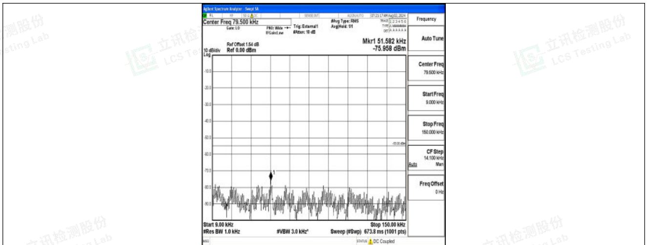
Band41-10MHz-16QAM-39700-1RB#0-0.009~0.15-PASS
