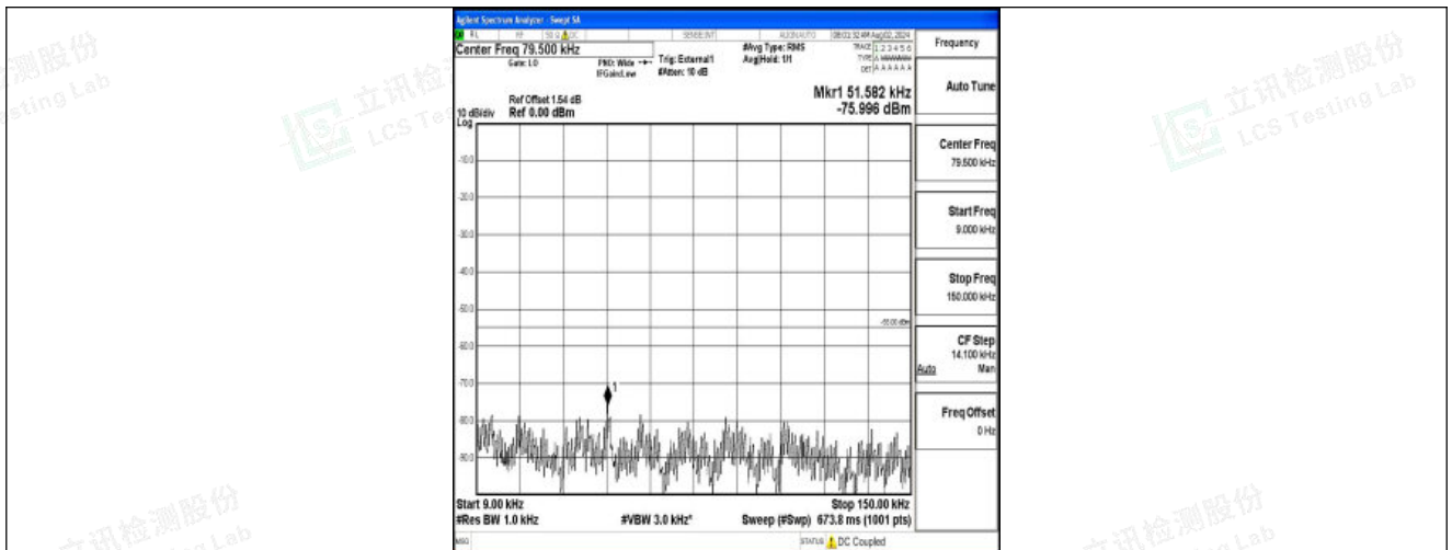
Band41-15MHz-16QAM-39725-1RB#0-0.009~0.15-PASS
