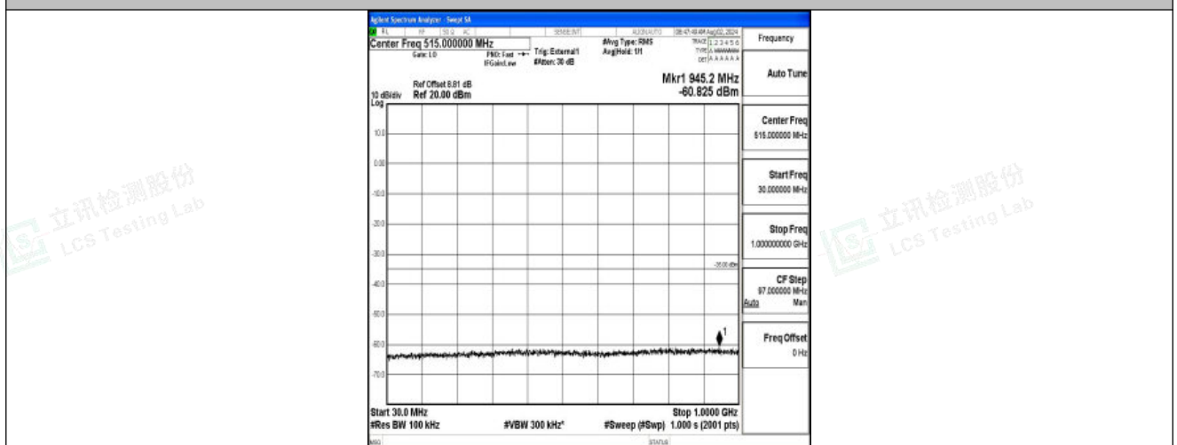
Band41-20MHz-16QAM-39750-1RB#0-30~1000-PASS
