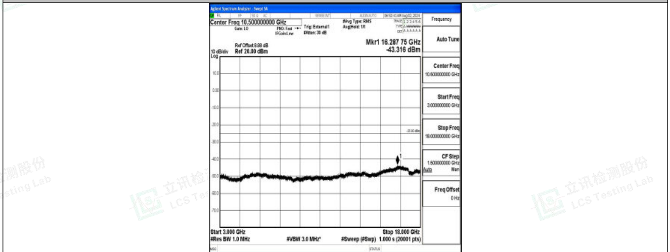
Band41-5MHz-QPSK-41565-1RB#0-3000~18000-PASS
