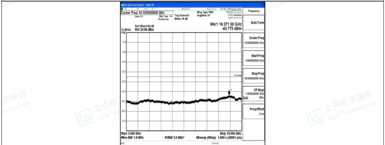
Band41-10MHz-QPSK-41540-1RB#0-3000~18000-PASS
