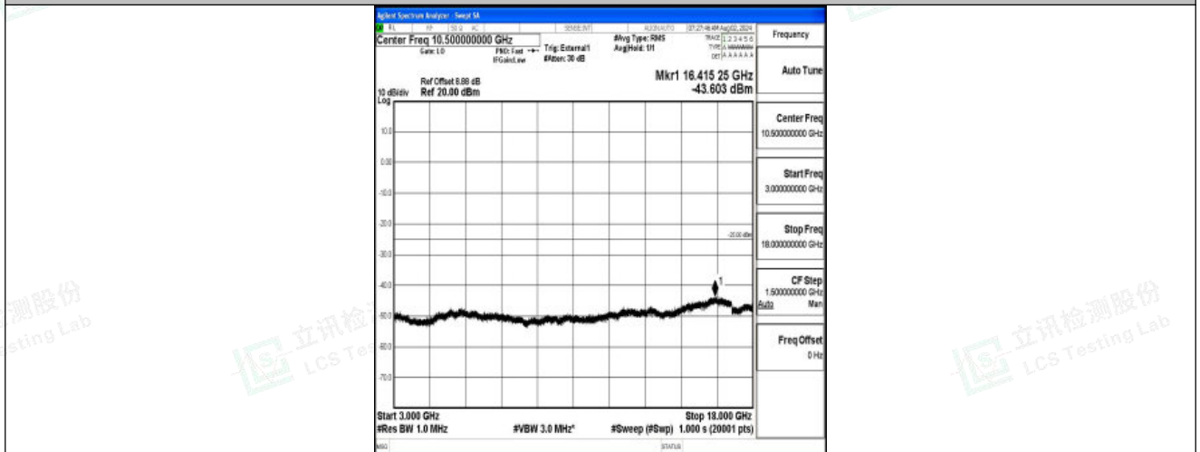
Band41-10MHz-16QAM-40620-1RB#0-3000~18000-PASS
