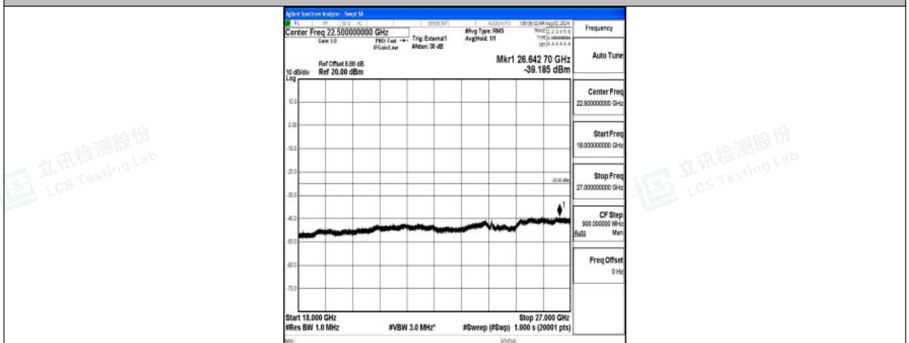
Band41-15MHz-QPSK-40620-1RB#0-18000~27000-PASS
