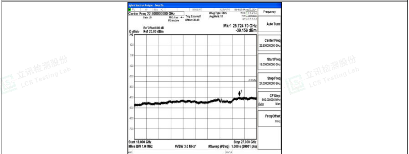
Band41-5MHz-QPSK-40620-1RB#0-18000~27000-PASS
