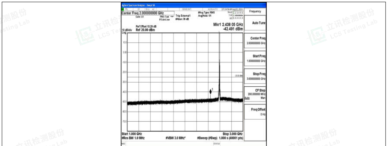
Band41-10MHz-QPSK-40620-1RB#0-1000~3000-PASS
