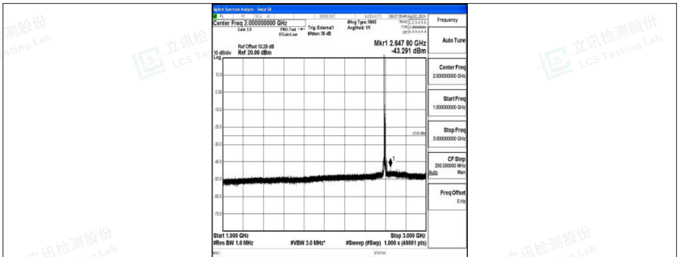
Band41-15MHz-16QAM-40620-1RB#0-1000~3000-PASS
