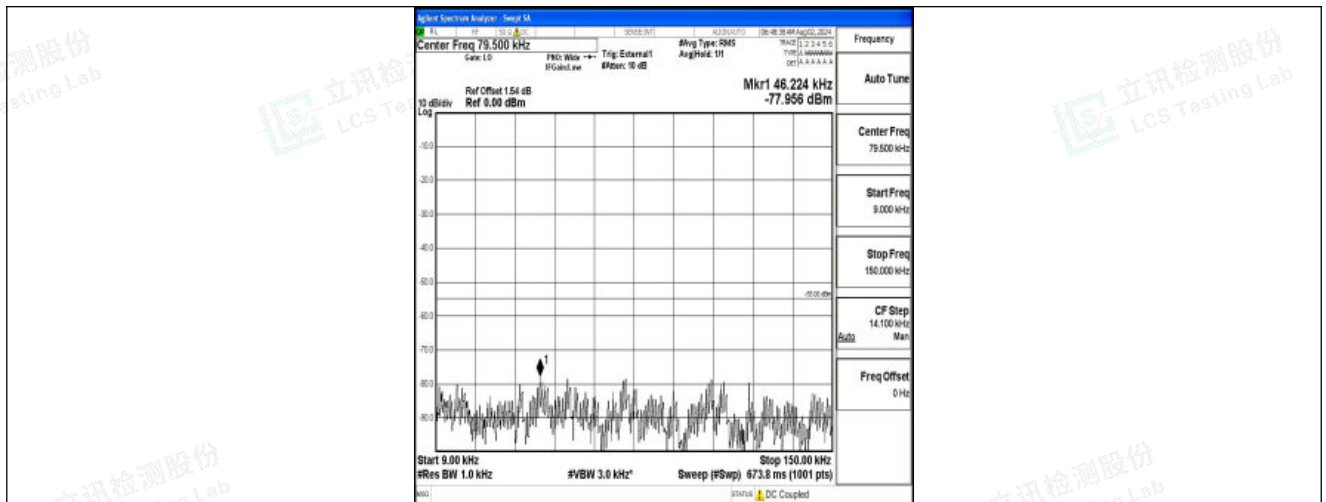
Band41-5MHz-16QAM-40620-1RB#0-0.009~0.15-PASS
