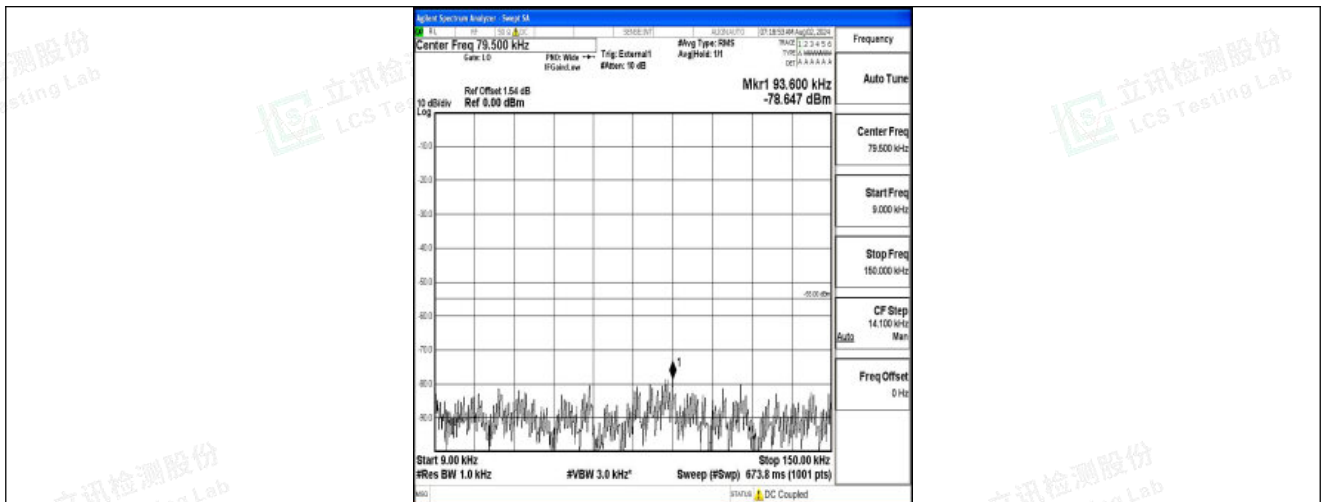
Band41-10MHz-QPSK-39700-1RB#0-0.009~0.15-PASS
