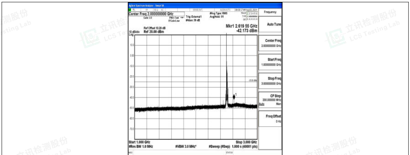
Band41-15MHz-QPSK-39725-1RB#0-1000~3000-PASS
