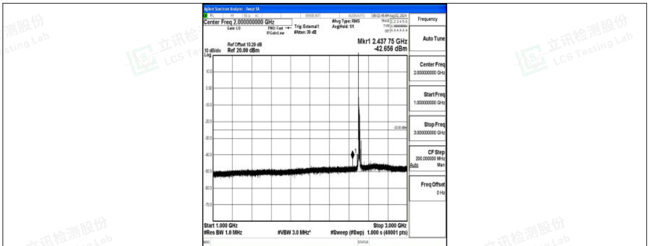
Band41-15MHz-16QAM-39725-1RB#0-1000~3000-PASS
