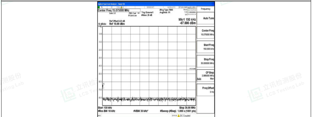
Band41-10MHz-QPSK-39700-1RB#0-0.15~30-PASS
