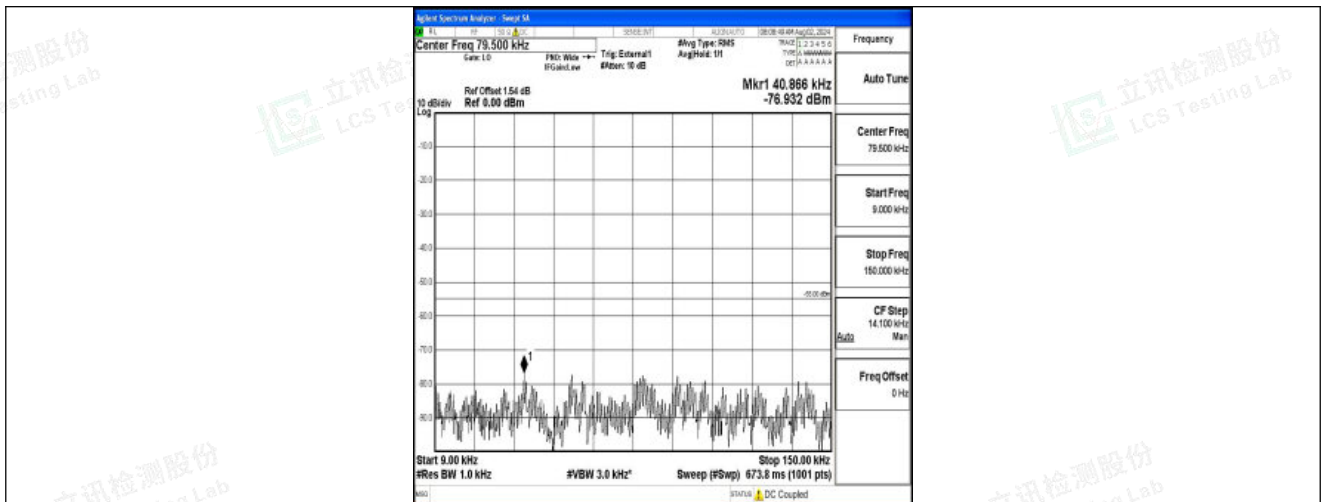
Band41-15MHz-QPSK-41515-1RB#0-0.009~0.15-PASS
