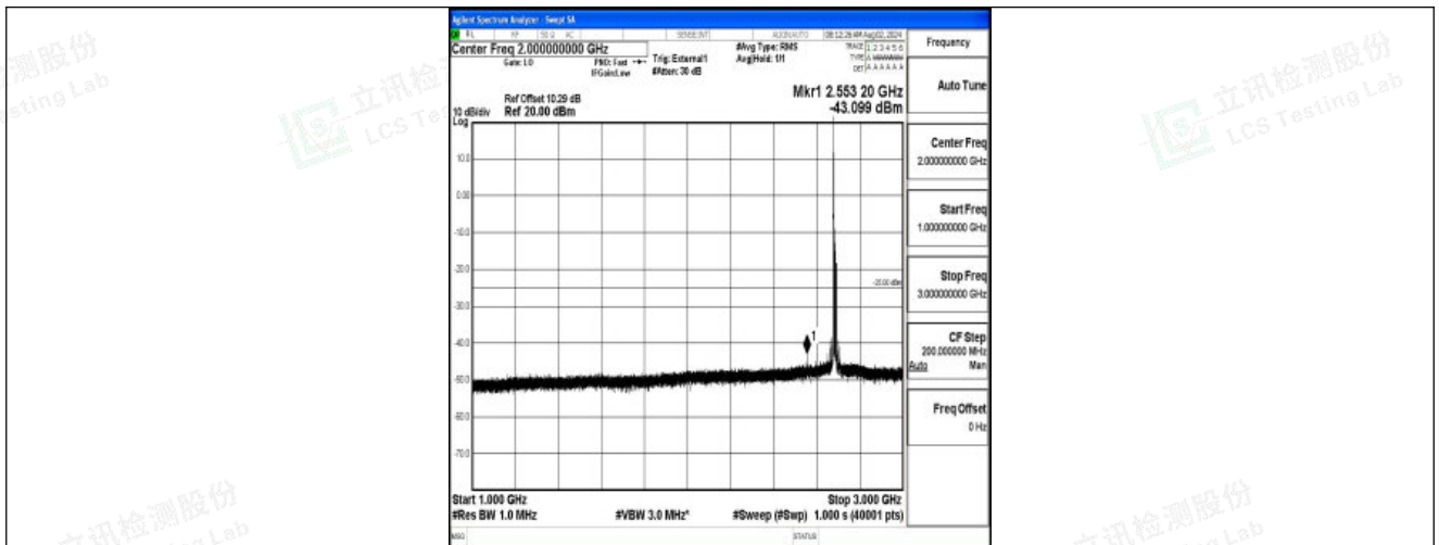
Band41-15MHz-16QAM-41515-1RB#0-1000~3000-PASS
