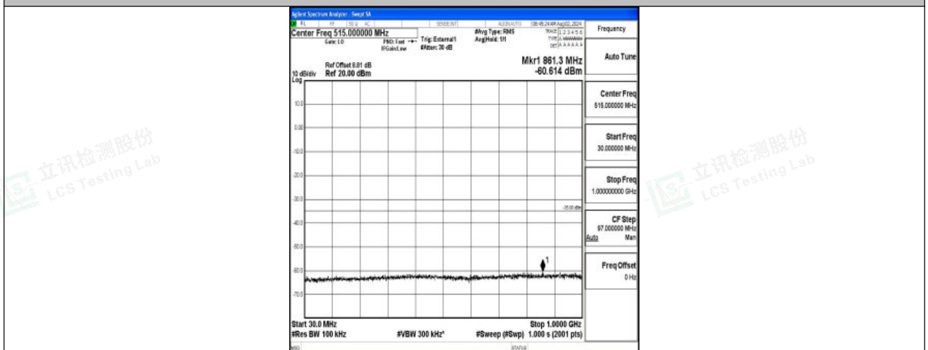
Band41-20MHz-QPSK-39750-1RB#0-30~1000-PASS
