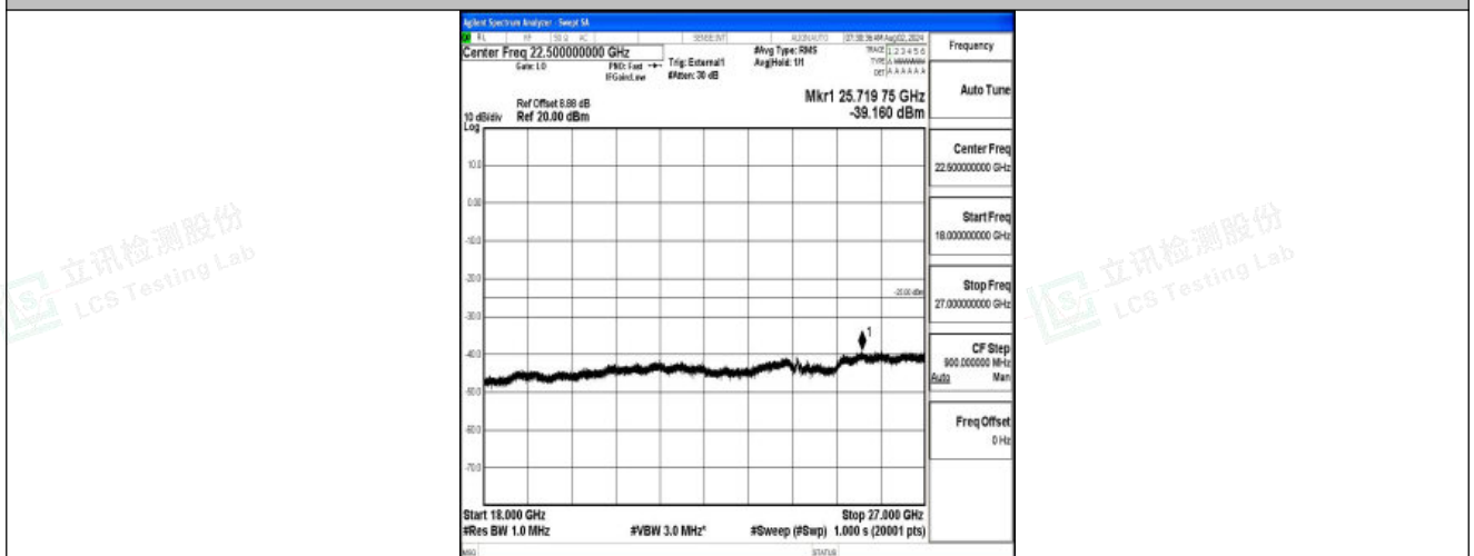
Band41-10MHz-QPSK-41540-1RB#0-18000~27000-PASS
