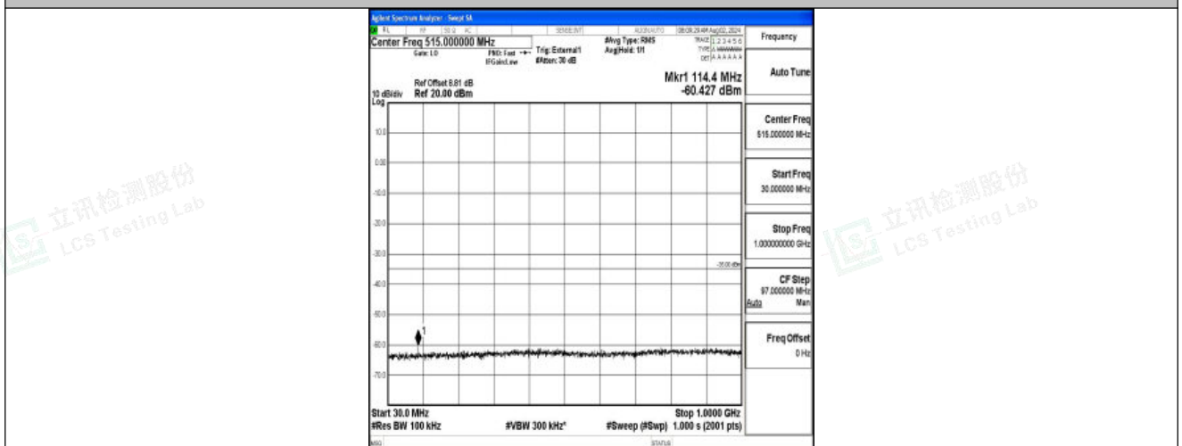
Band41-15MHz-QPSK-41515-1RB#0-30~1000-PASS
