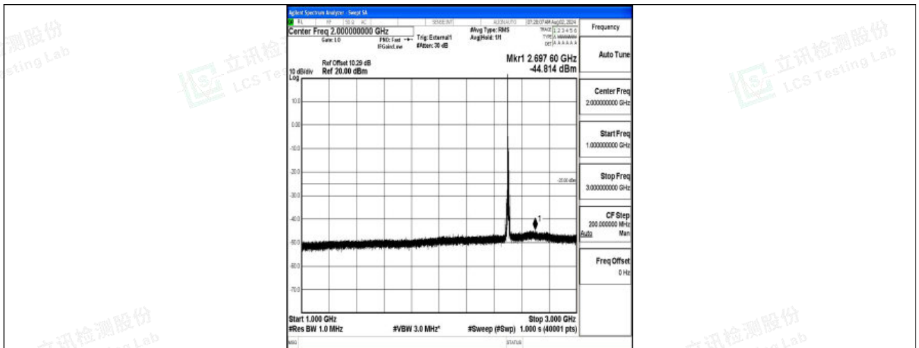
Band41-10MHz-QPSK-39700-1RB#0-1000~3000-PASS
