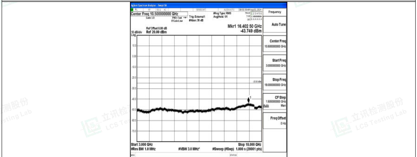
Band41-20MHz-16QAM-40620-1RB#0-3000~18000-PASS
