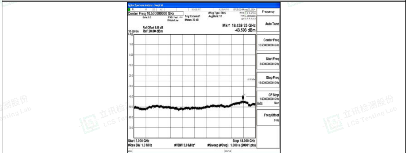
Band41-10MHz-QPSK-40620-1RB#0-3000~18000-PASS
