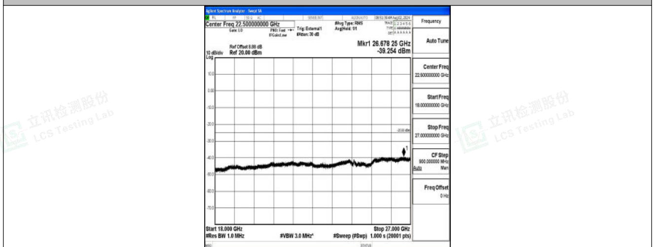
Band41-20MHz-QPSK-40620-1RB#0-18000~27000-PASS
