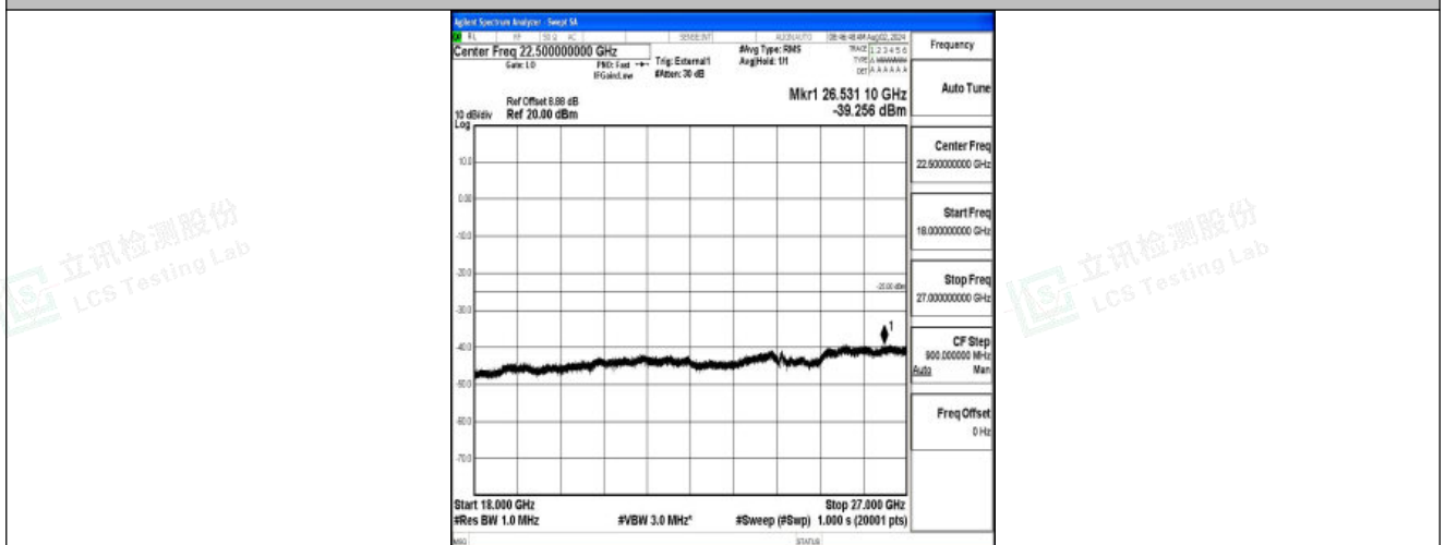
Band41-20MHz-QPSK-39750-1RB#0-18000~27000-PASS
