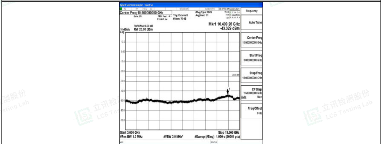
Band41-5MHz-QPSK-40620-1RB#0-3000~18000-PASS
