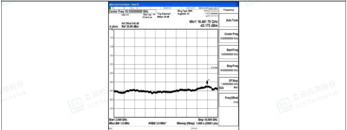
Band41-15MHz-QPSK-39725-1RB#0-3000~18000-PASS
