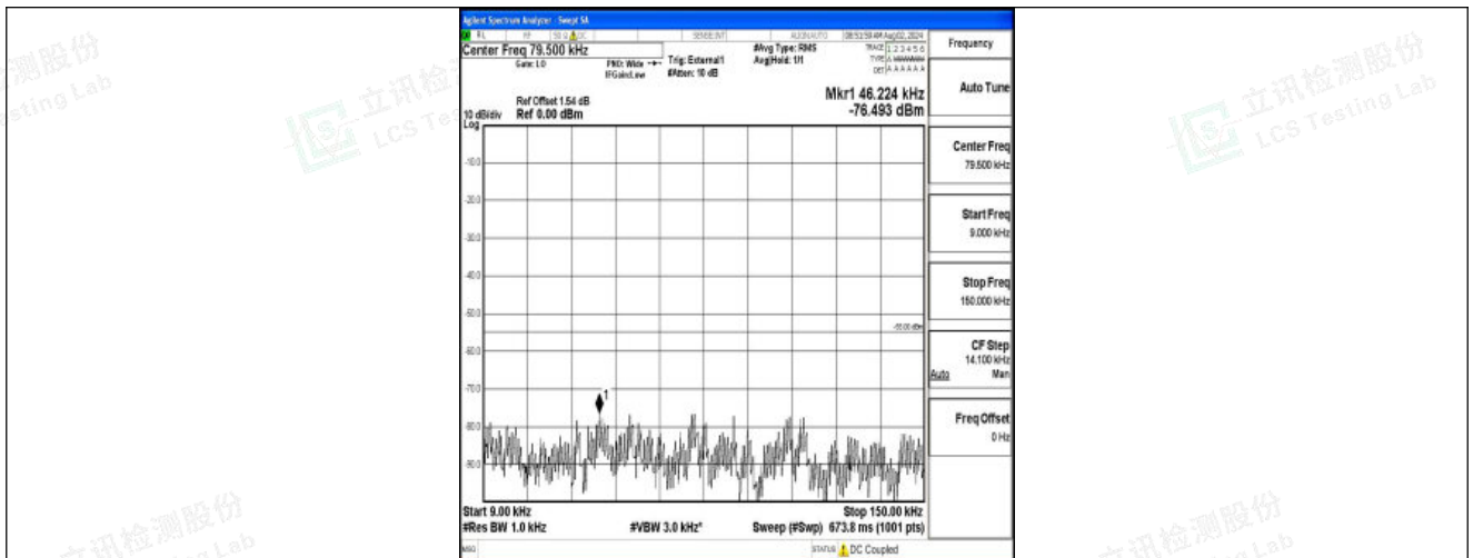
Band41-20MHz-16QAM-40620-1RB#0-0.009~0.15-PASS
