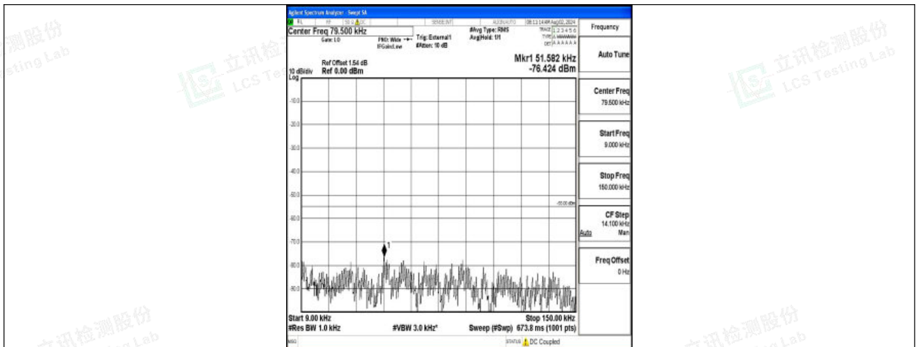
Band41-15MHz-16QAM-41515-1RB#0-0.009~0.15-PASS
