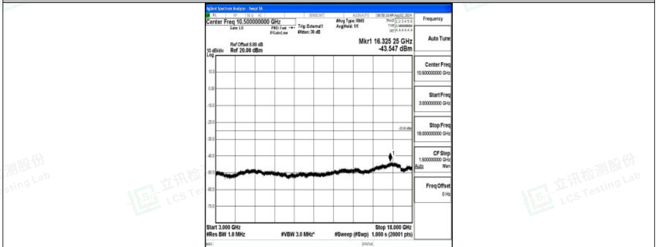
Band41-5MHz-16QAM-40620-1RB#0-3000~18000-PASS
