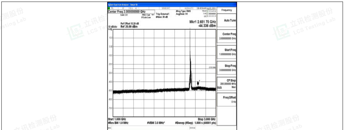
Band41-20MHz-QPSK-39750-1RB#0-1000~3000-PASS
