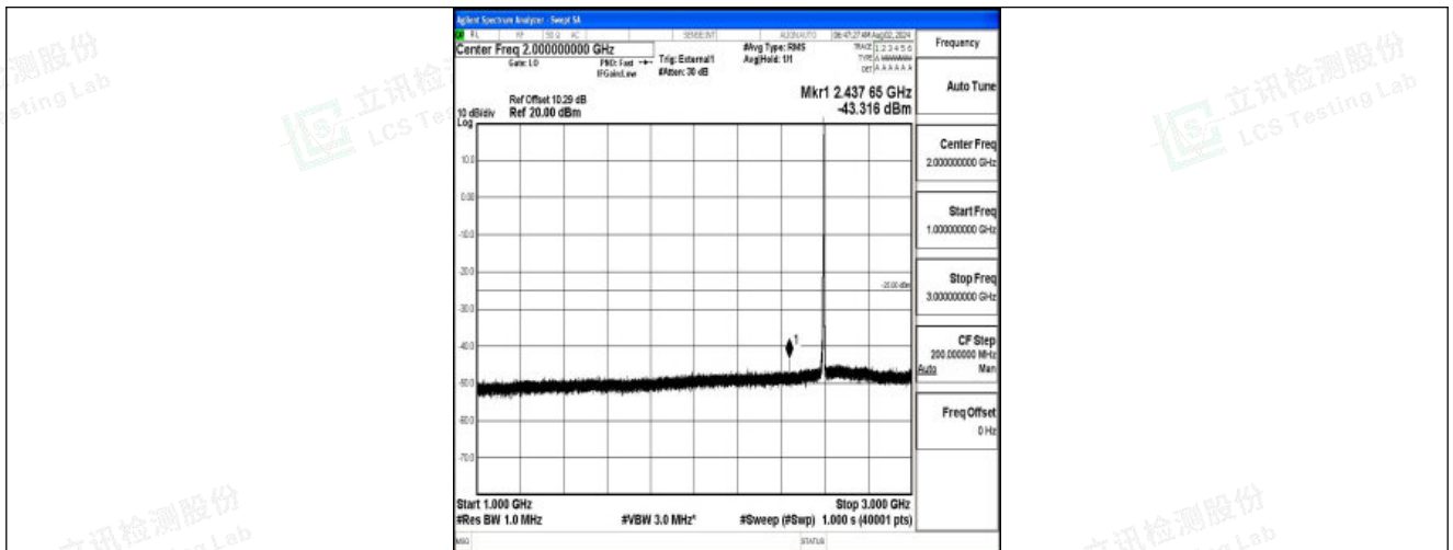
Band41-5MHz-QPSK-40620-1RB#0-1000~3000-PASS
