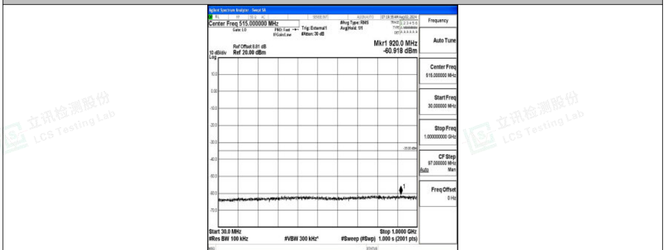
Band41-10MHz-QPSK-39700-1RB#0-30~1000-PASS
