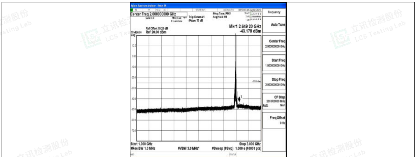
Band41-20MHz-16QAM-40620-1RB#0-1000~3000-PASS
