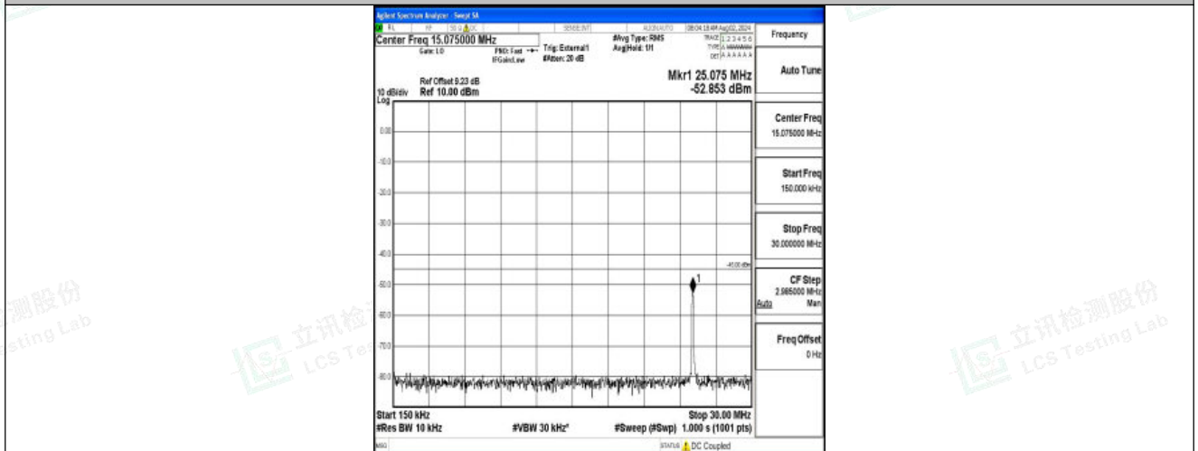
Band41-15MHz-QPSK-40620-1RB#0-0.15~30-PASS
