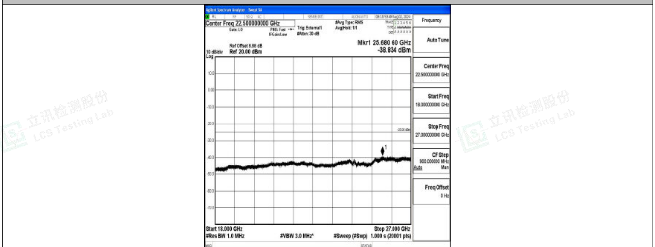
Band41-15MHz-QPSK-41515-1RB#0-18000~27000-PASS
