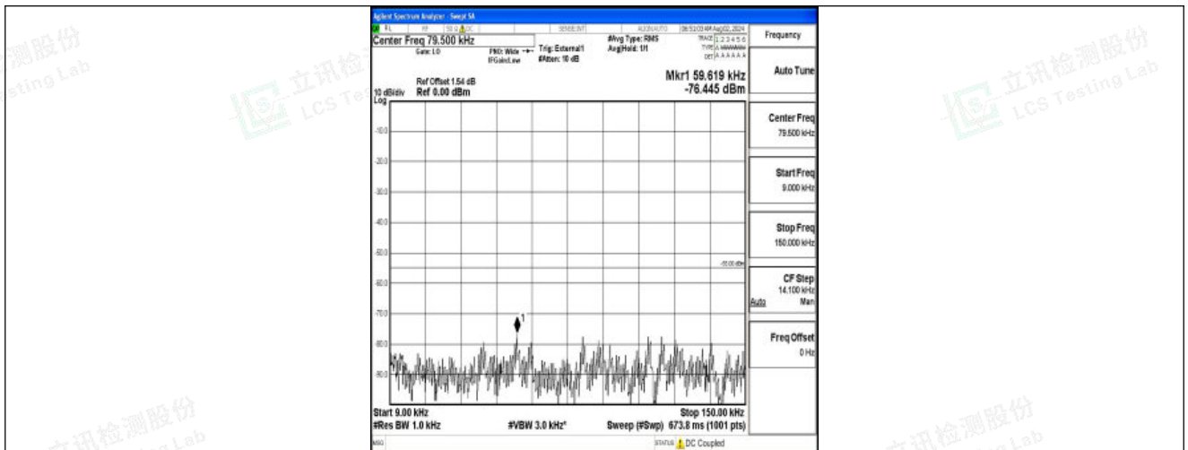
Band41-5MHz-QPSK-41565-1RB#0-0.009~0.15-PASS
