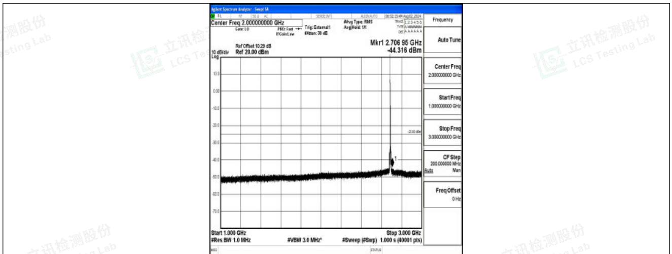
Band41-5MHz-QPSK-41565-1RB#0-1000~3000-PASS
