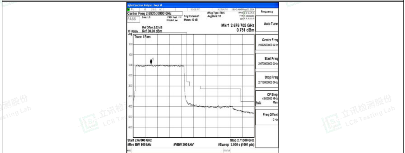
Band41-20MHz-QPSK-41490-100RB#0-PASS
