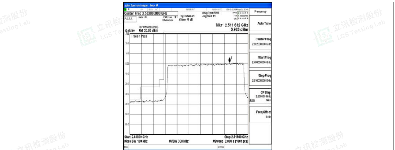
Band41-20MHz-16QAM-39750-100RB#0-PASS
