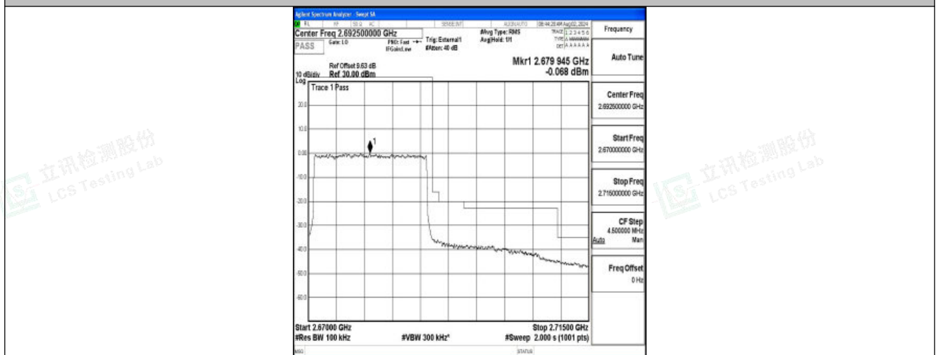
Band41-20MHz-16QAM-41490-100RB#0-PASS
