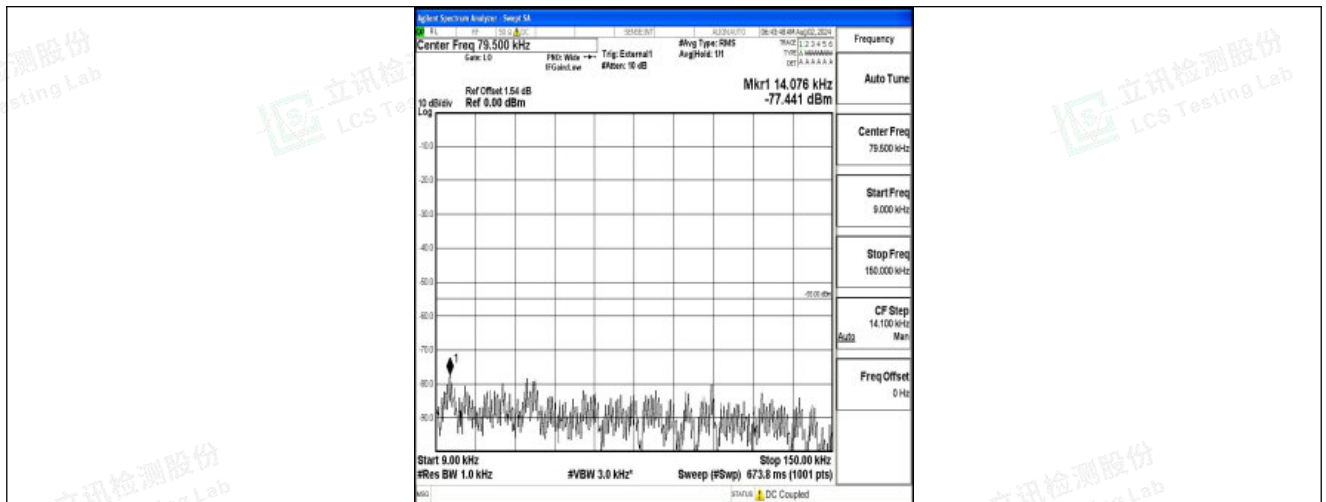
Band41-5MHz-16QAM-39675-1RB#0-0.009~0.15-PASS
