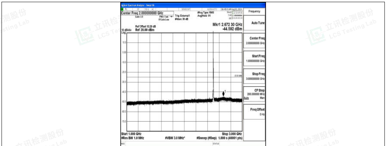
Band41-5MHz-16QAM-39675-1RB#0-1000~3000-PASS
