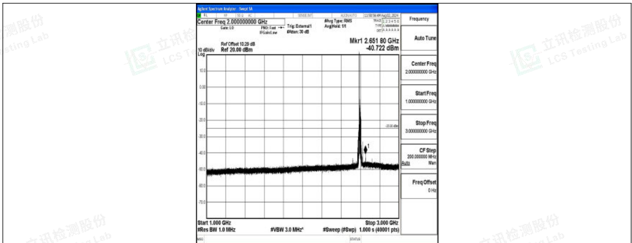
Band38-20MHz-16QAM-38000-1RB#0-1000~3000-PASS
