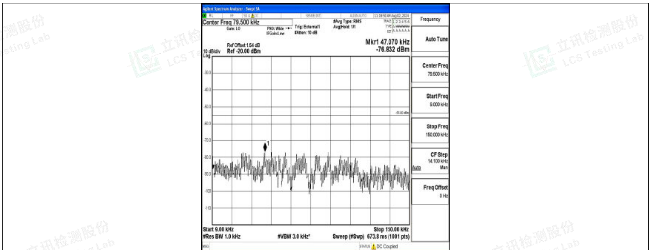
Band38-15MHz-16QAM-38000-1RB#0-0.009~0.15-PASS
