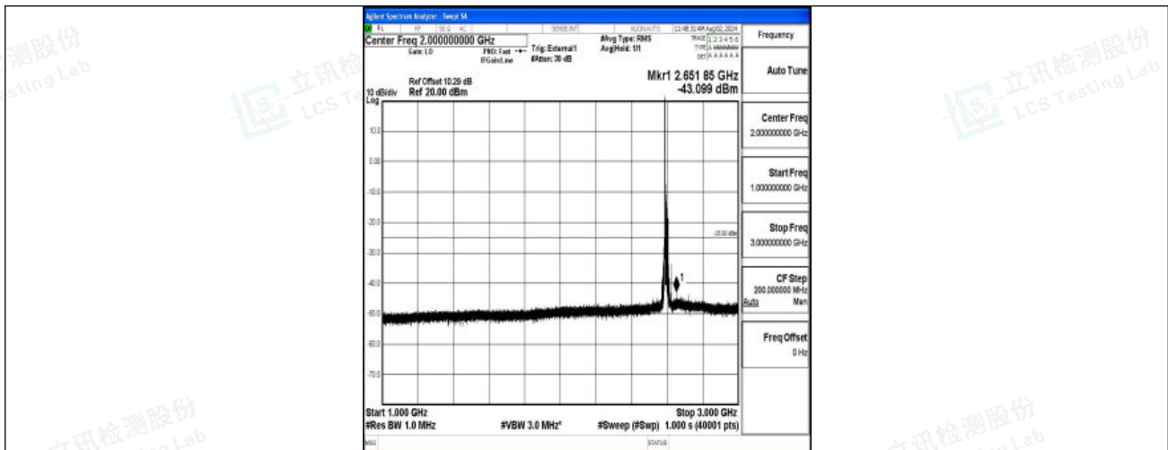
Band38-20MHz-QPSK-38000-1RB#0-1000~3000-PASS
