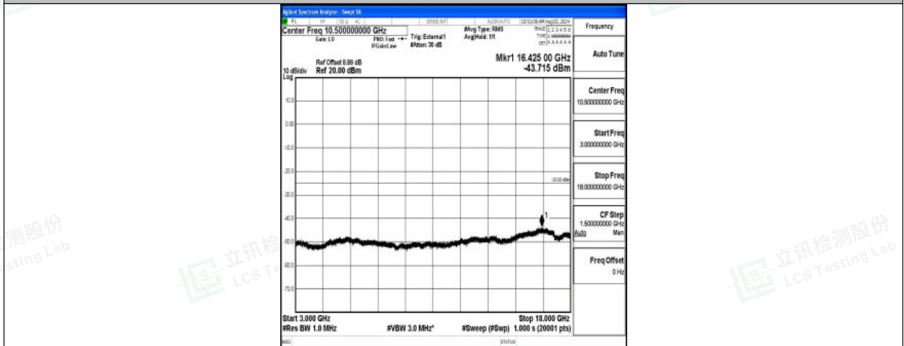
Band38-10MHz-QPSK-38200-1RB#0-3000~18000-PASS
