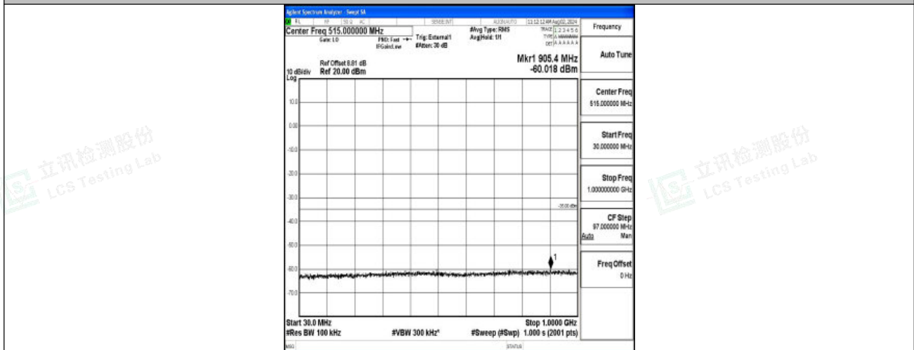
Band38-15MHz-QPSK-37825-1RB#0-30~1000-PASS
