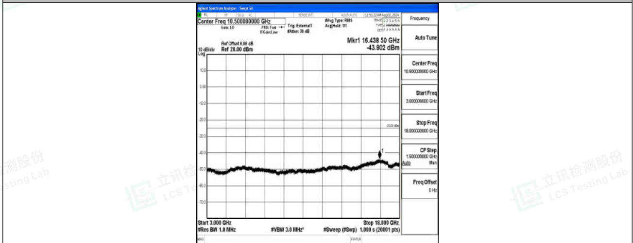
Band38-20MHz-16QAM-38000-1RB#0-3000~18000-PASS
