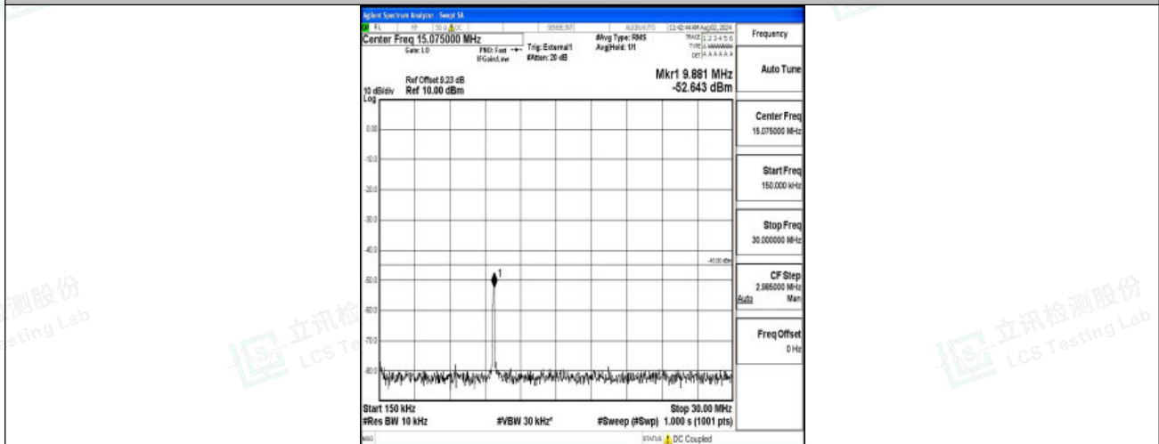
Band38-20MHz-QPSK-37850-1RB#0-0.15~30-PASS
