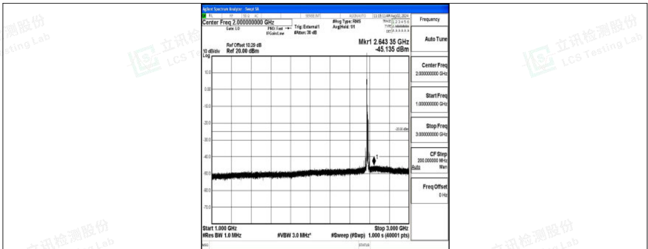
Band38-15MHz-16QAM-37825-1RB#0-1000~3000-PASS
