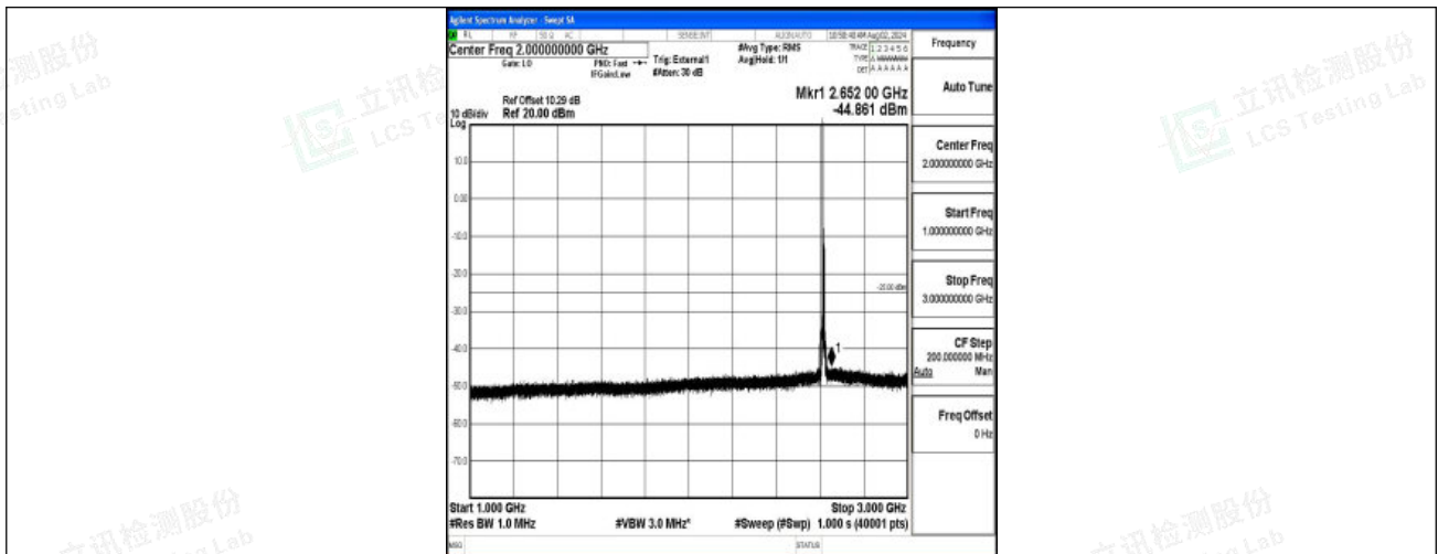
Band38-10MHz-QPSK-38200-1RB#0-1000~3000-PASS
