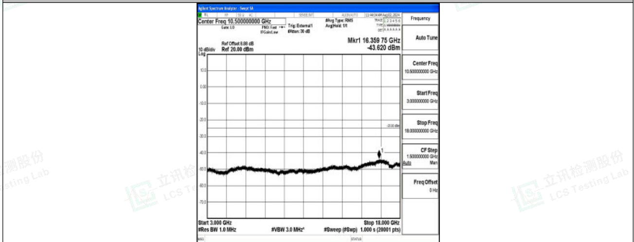
Band38-20MHz-QPSK-37850-1RB#0-3000~18000-PASS
