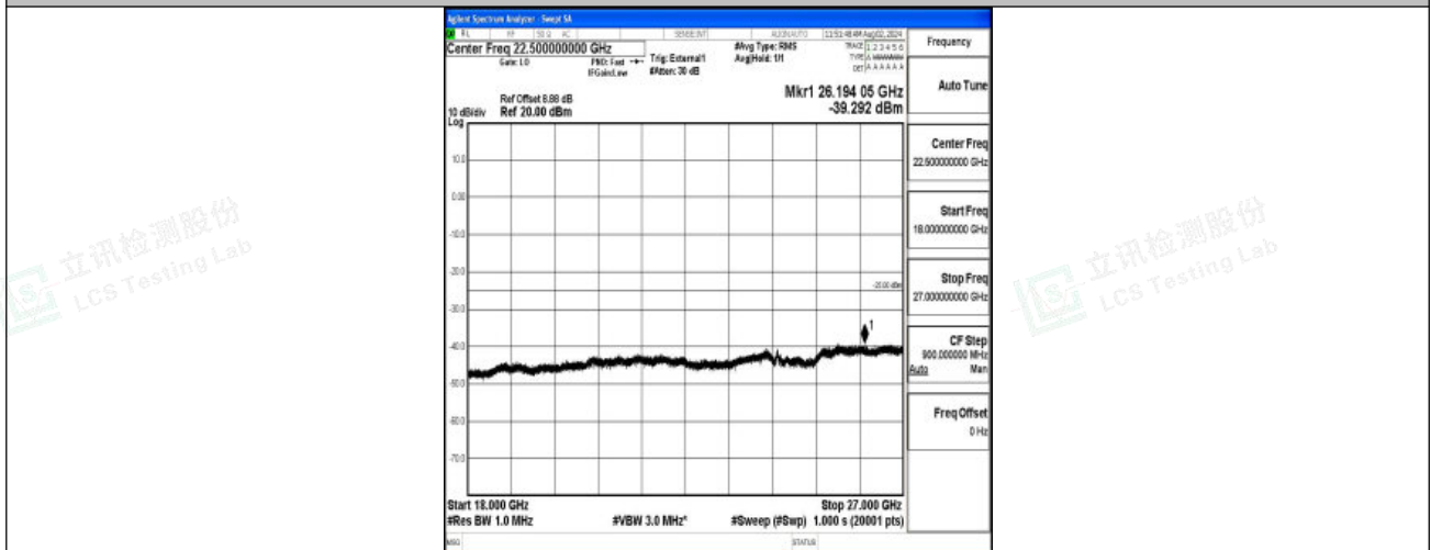
Band38-20MHz-16QAM-38000-1RB#0-18000~27000-PASS
