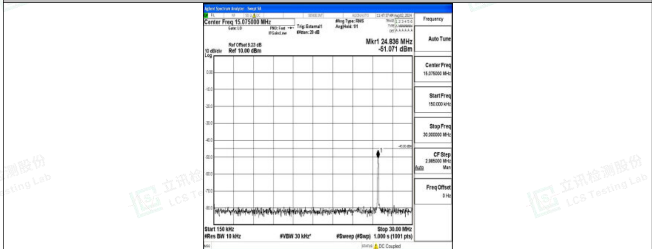
Band38-20MHz-QPSK-38000-1RB#0-0.15~30-PASS
