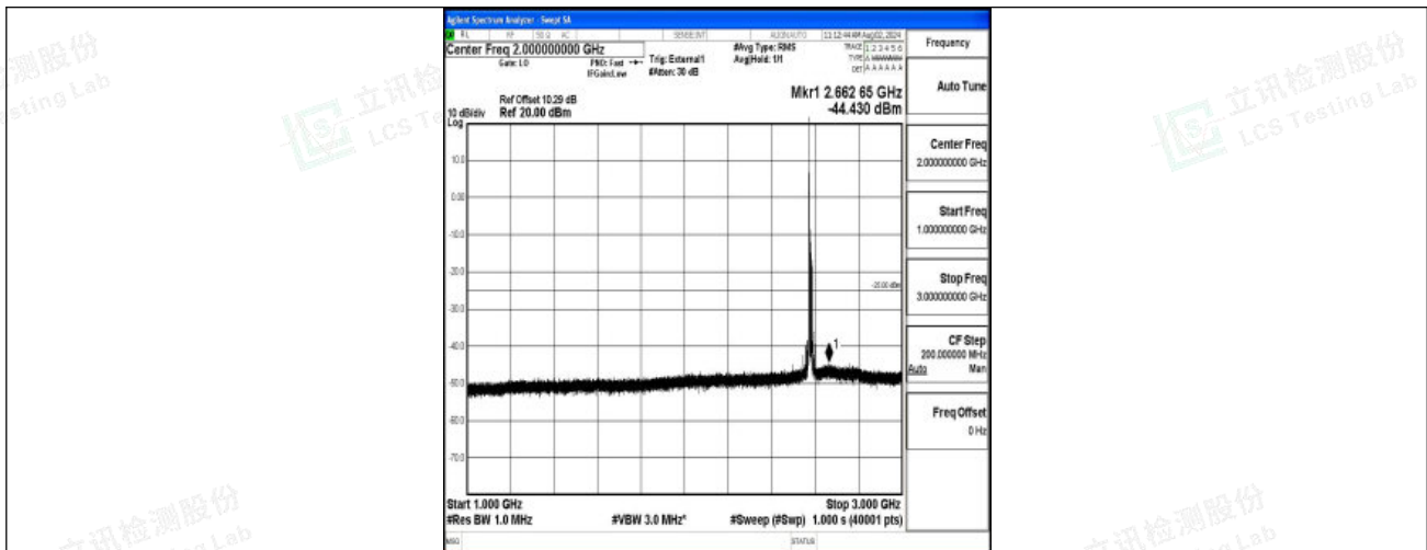
Band38-15MHz-QPSK-37825-1RB#0-1000~3000-PASS
