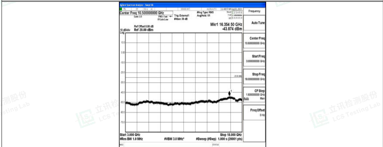
Band38-20MHz-QPSK-38000-1RB#0-3000~18000-PASS
