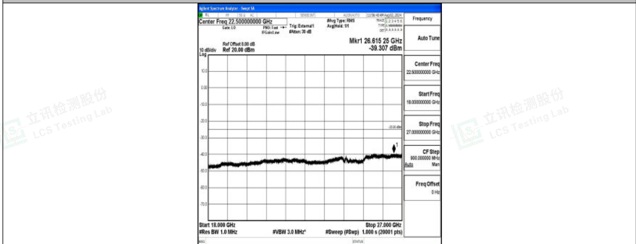
Band38-20MHz-16QAM-38150-1RB#0-18000~27000-PASS
