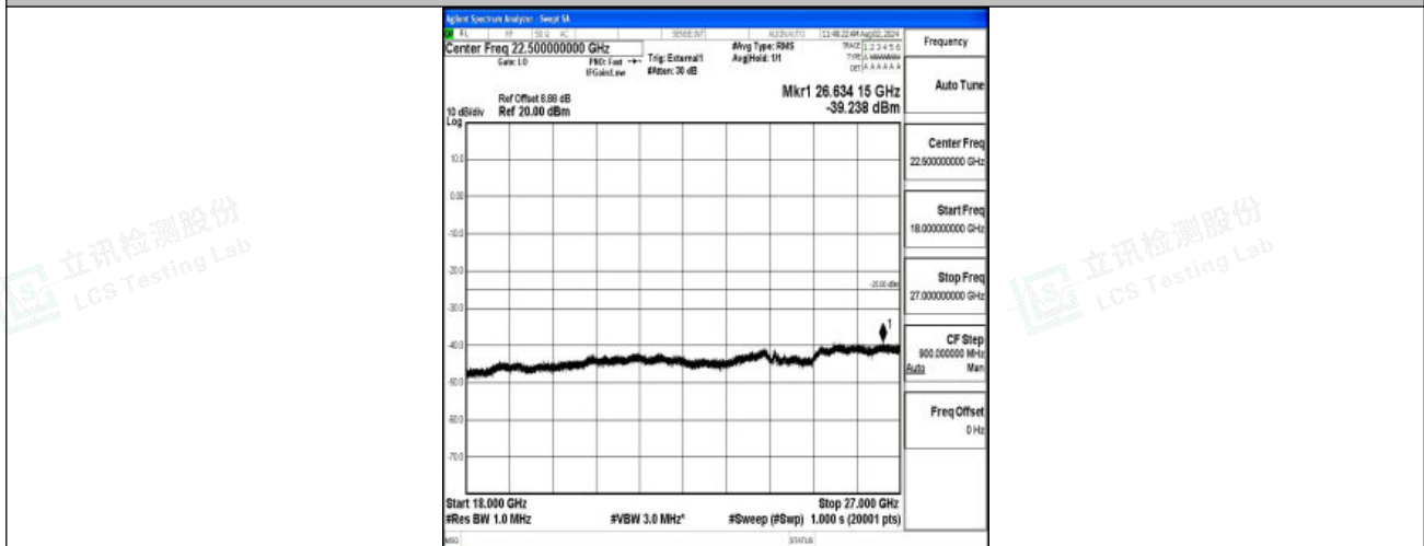
Band38-20MHz-QPSK-38000-1RB#0-18000~27000-PASS
