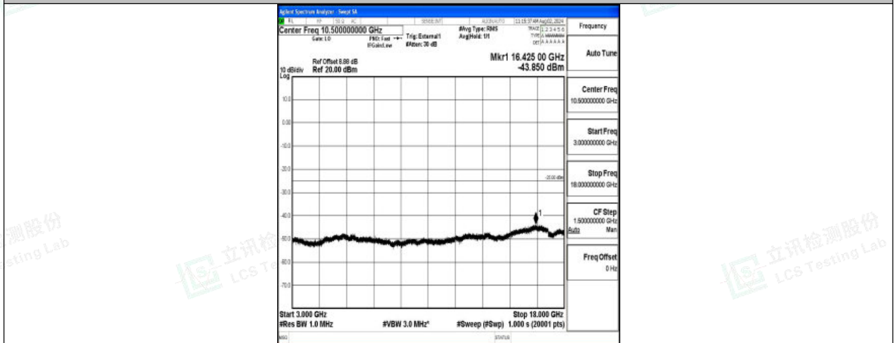
Band38-15MHz-16QAM-37825-1RB#0-3000~18000-PASS
