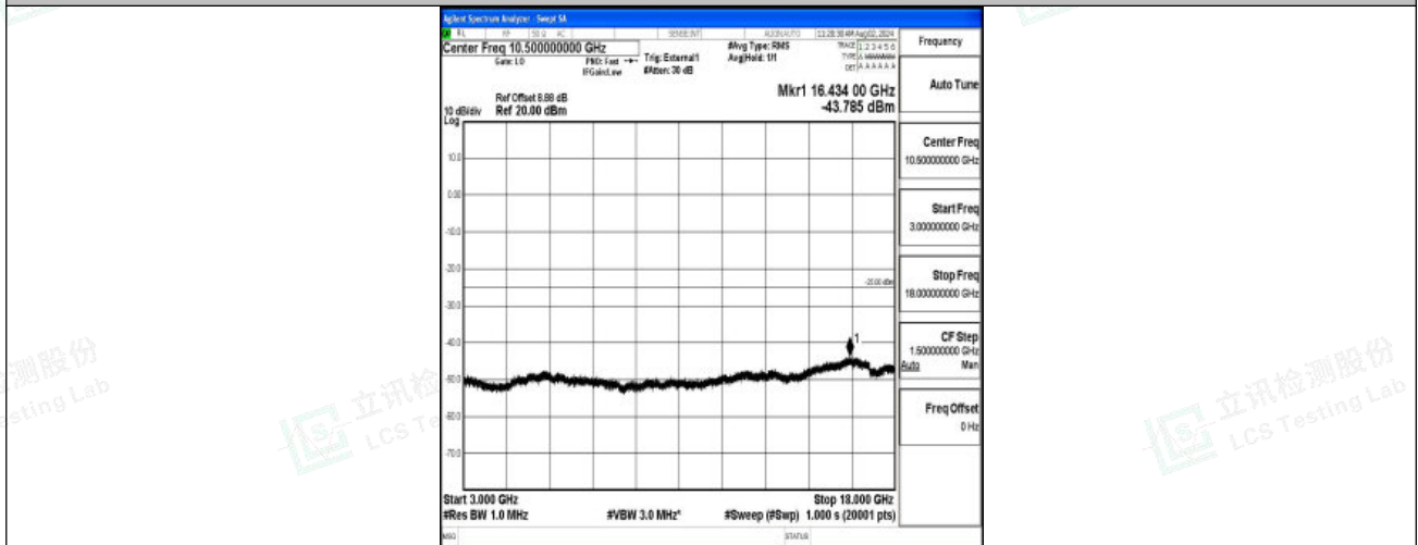
Band38-15MHz-16QAM-38000-1RB#0-3000~18000-PASS
