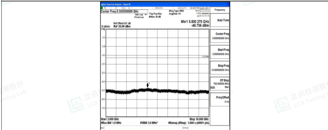
Band12-3MHz-QPSK-23165-1RB#0-3000~10000-PASS
