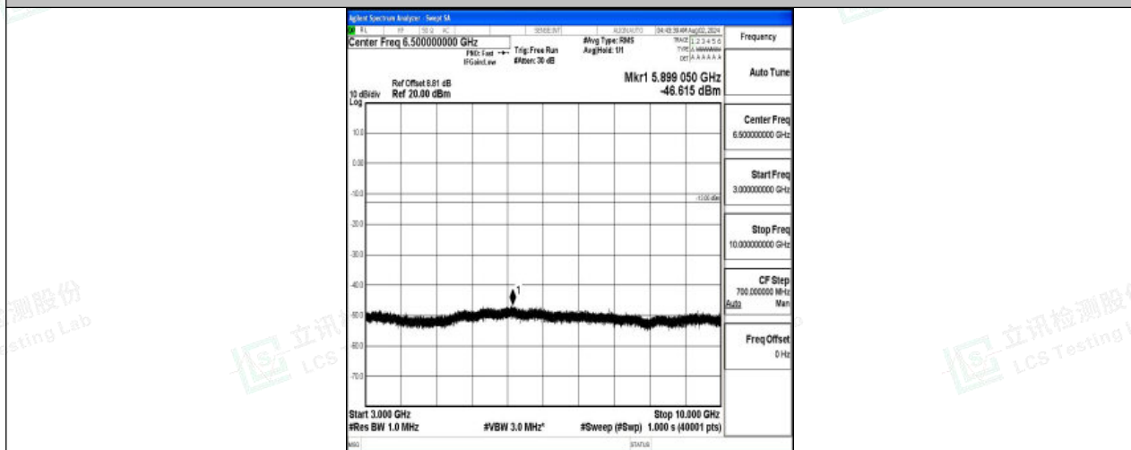
Band12-3MHz-16QAM-23025-1RB#0-3000~10000-PASS
