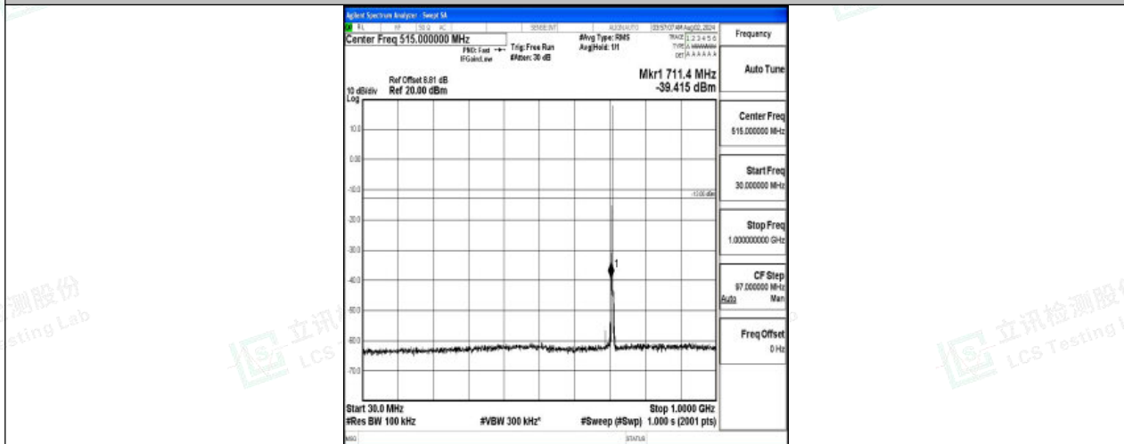
Band12-1.4MHz-16QAM-23173-1RB#0-30~1000-PASS
