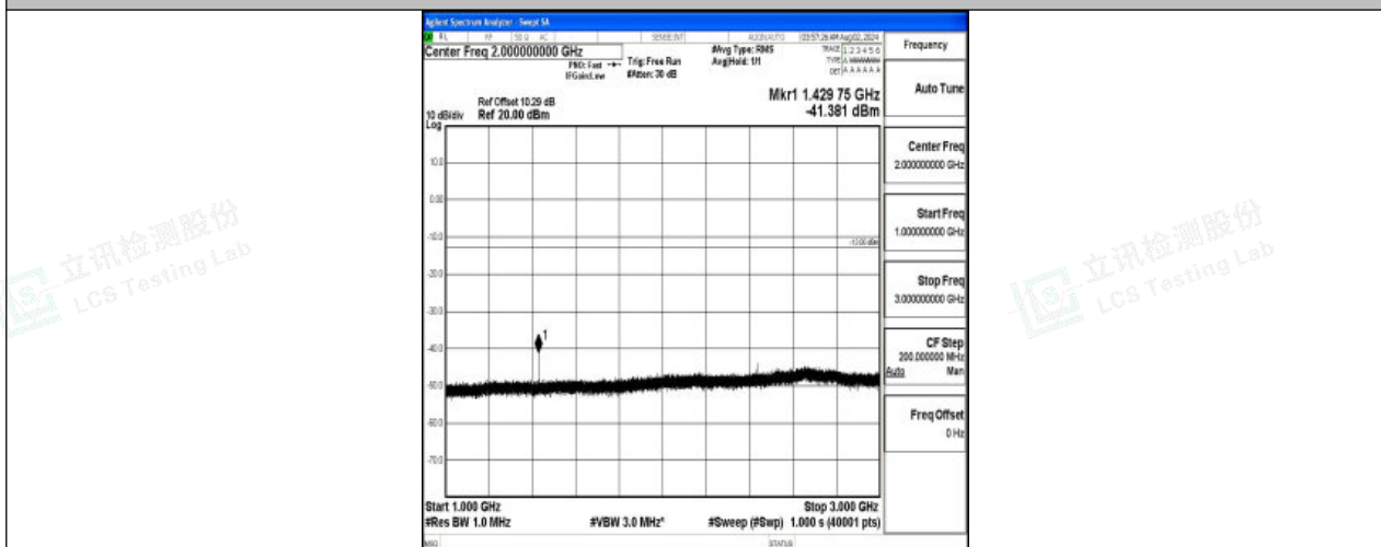
Band12-1.4MHz-16QAM-23173-1RB#0-1000~3000-PASS
