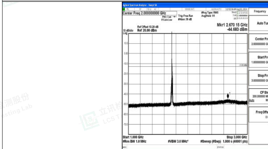
Band4-10MHz-QPSK-20175-1RB#0-1000~3000-PASS
