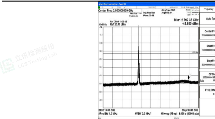
Band4-15MHz-QPSK-20325-1RB#0-1000~3000-PASS
