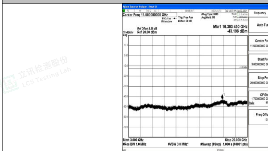
Band4-3MHz-16QAM-20385-1RB#0-3000~20000-PASS
