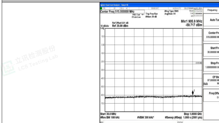
Band4-15MHz-16QAM-20175-1RB#0-30~1000-PASS
