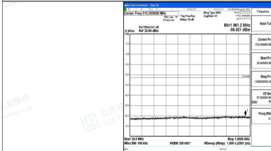
Band4-20MHz-16QAM-20050-1RB#0-30~1000-PASS
