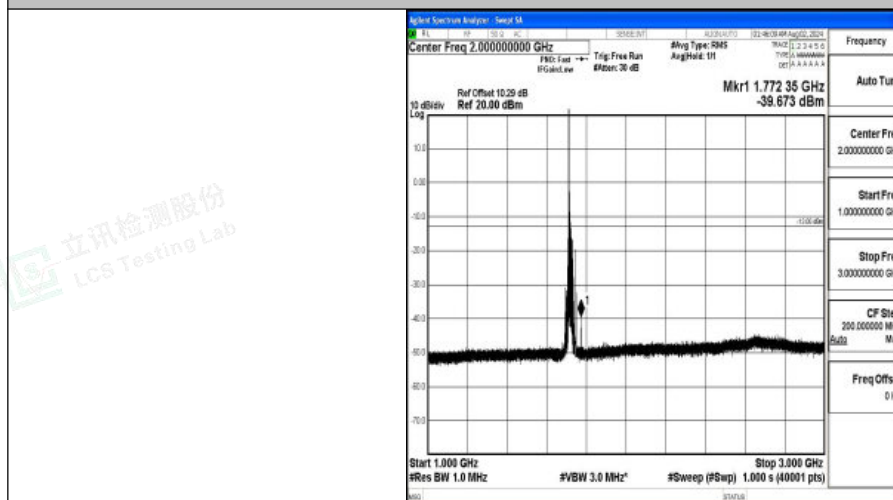
Band4-20MHz-16QAM-20050-1RB#0-1000~3000-PASS
