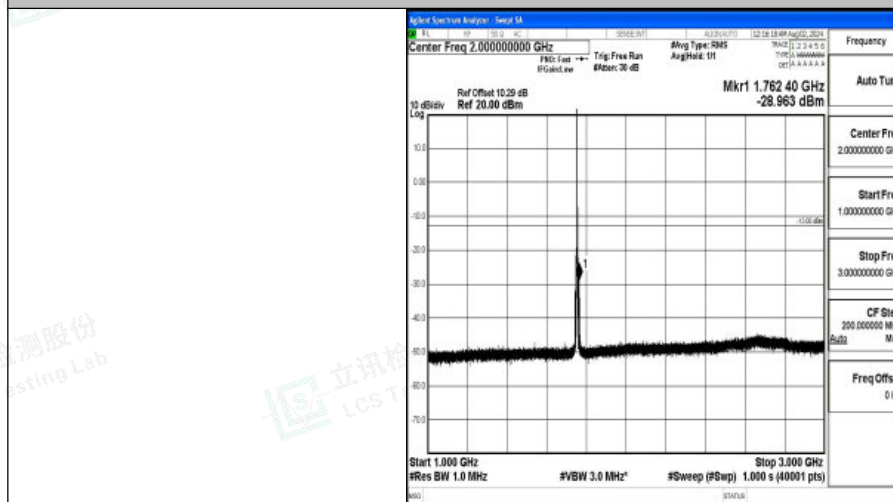
Band4-3MHz-16QAM-20385-1RB#0-1000~3000-PASS
