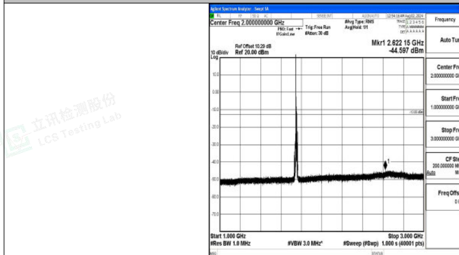
Band4-10MHz-QPSK-20350-1RB#0-1000~3000-PASS
