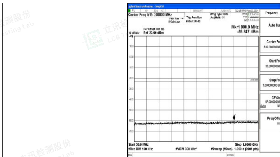
Band4-3MHz-16QAM-20385-1RB#0-30~1000-PASS
