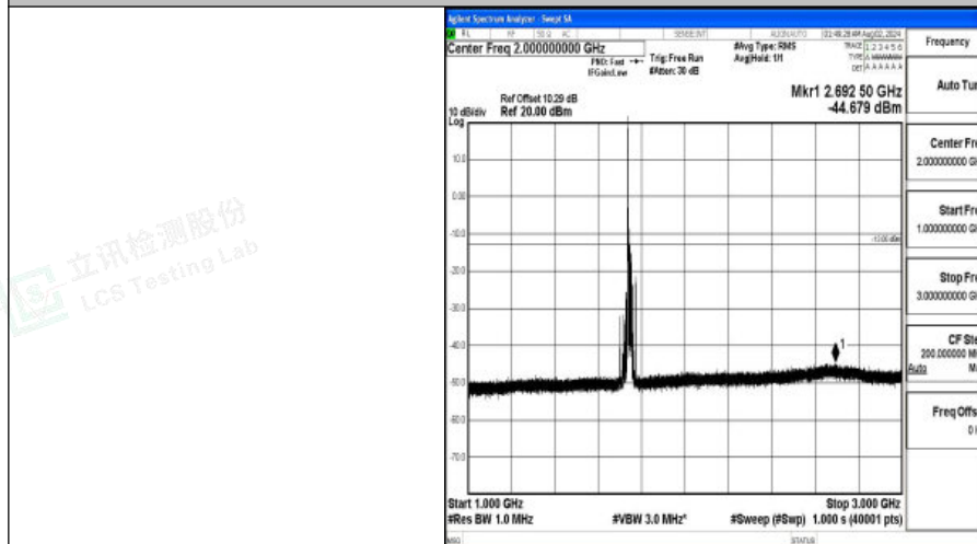
Band4-20MHz-QPSK-20300-1RB#0-1000~3000-PASS
