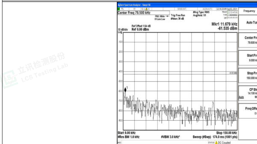
Band4-5MHz-QPSK-20375-1RB#0-0.009~0.15-PASS
