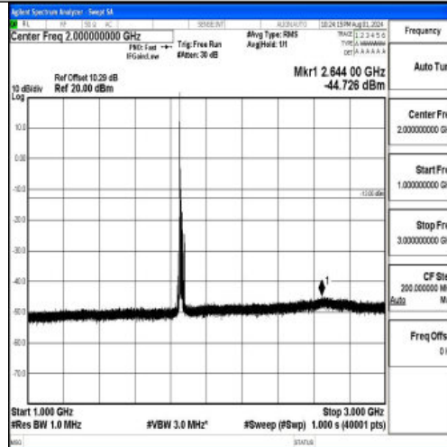
Band2-15MHz-16QAM-18675-1RB#0-1000~3000-PASS
