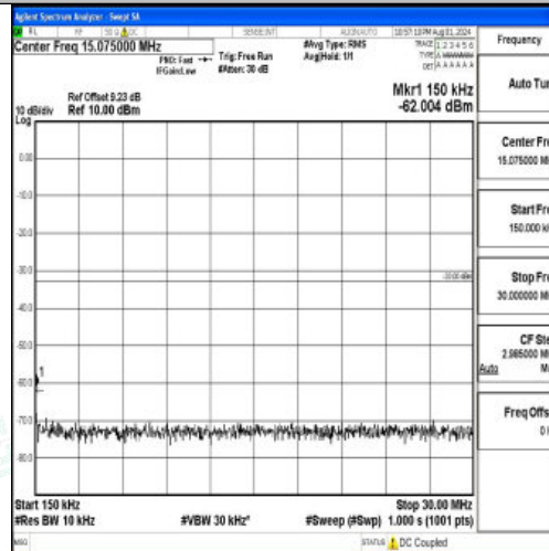
Band2-20MHz-QPSK-18700-1RB#0-0.15~30-PASS
