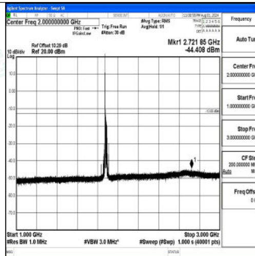
Band2-20MHz-16QAM-18900-1RB#0-1000~3000-PASS
