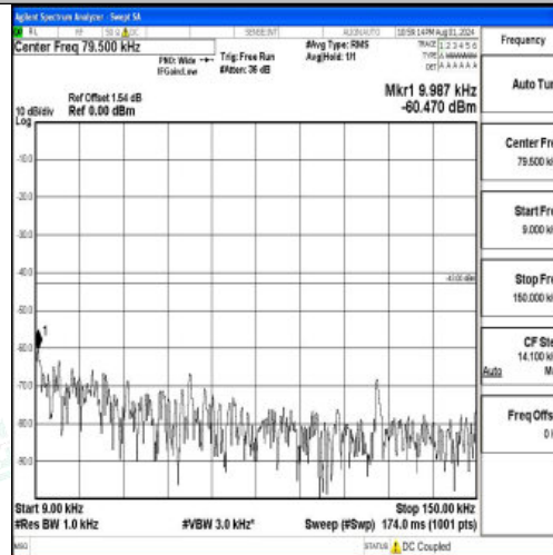
Band2-20MHz-QPSK-18900-1RB#0-0.009~0.15-PASS
