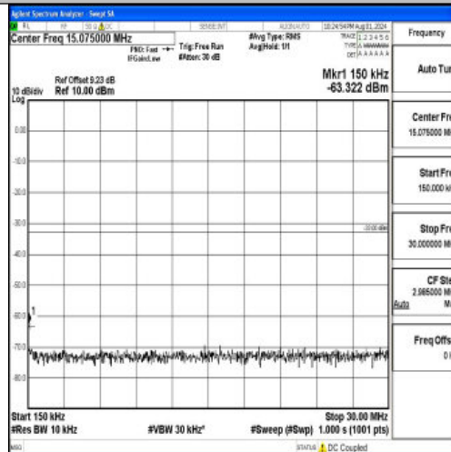
Band2-15MHz-QPSK-18900-1RB#0-0.15~30-PASS
