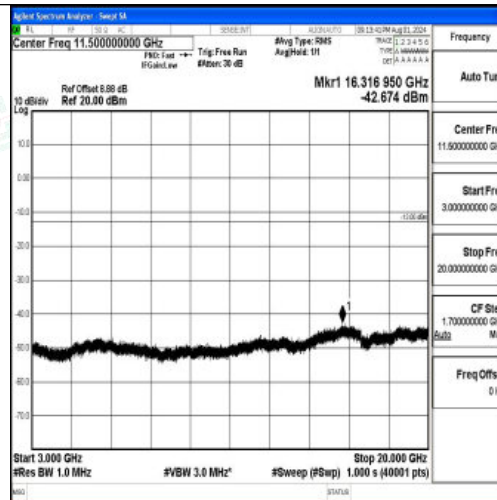
Band2-3MHz-QPSK-19185-1RB#0-3000~20000-PASS
