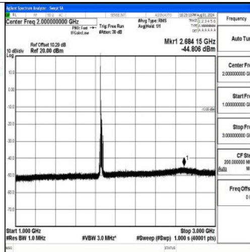
Band2-15MHz-QPSK-18675-1RB#0-1000~3000-PASS
