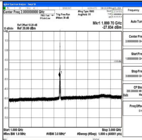
Band2-3MHz-QPSK-19185-1RB#0-1000~3000-PASS
