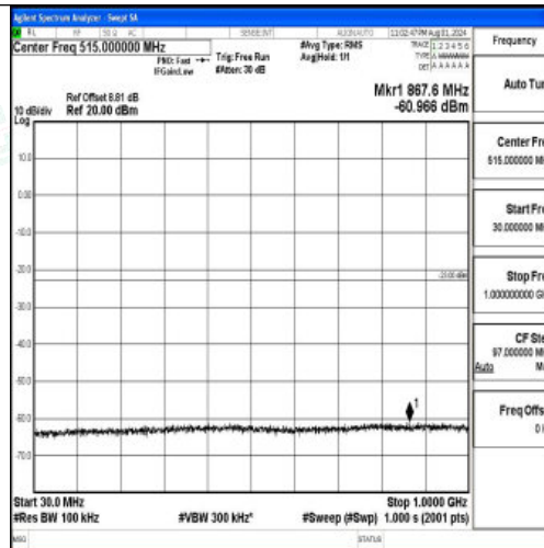
Band2-20MHz-16QAM-19100-1RB#0-30~1000-PASS
