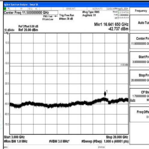
Band2-20MHz-16QAM-18900-1RB#0-3000~20000-PASS
