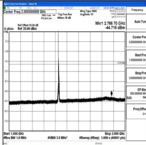
Band2-10MHz-16QAM-18650-1RB#0-1000~3000-PASS
