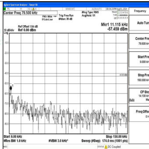
Band2-5MHz-16QAM-18900-1RB#0-0.009~0.15-PASS
