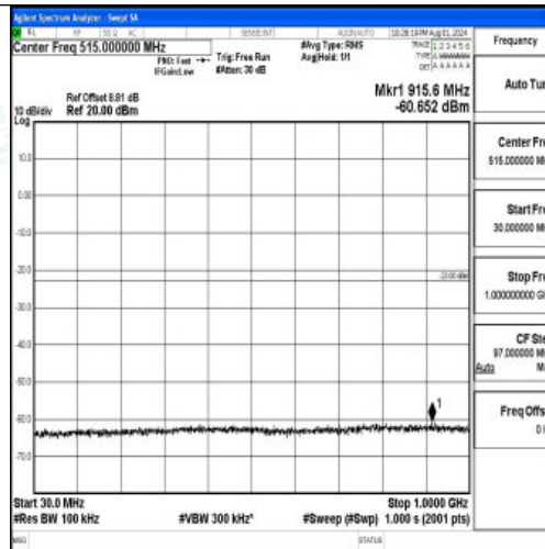
Band2-15MHz-16QAM-19125-1RB#0-30~1000-PASS
