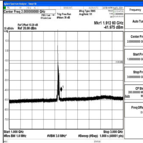
Band2-20MHz-16QAM-18700-1RB#0-1000~3000-PASS
