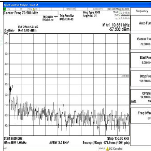
Band2-3MHz-16QAM-18900-1RB#0-0.009~0.15-PASS
