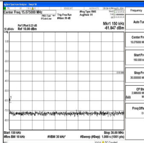
Band2-5MHz-16QAM-19175-1RB#0-0.15~30-PASS
