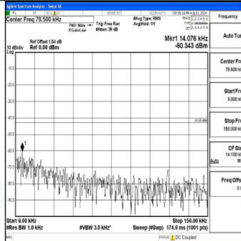
Band2-10MHz-QPSK-18900-1RB#0-0.009~0.15-PASS
