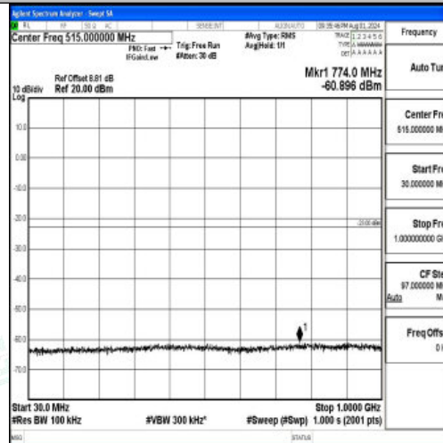
Band2-5MHz-QPSK-19175-1RB#0-30~1000-PASS
