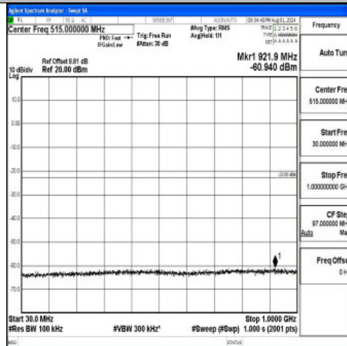
Band2-5MHz-16QAM-18900-1RB#0-30~1000-PASS
