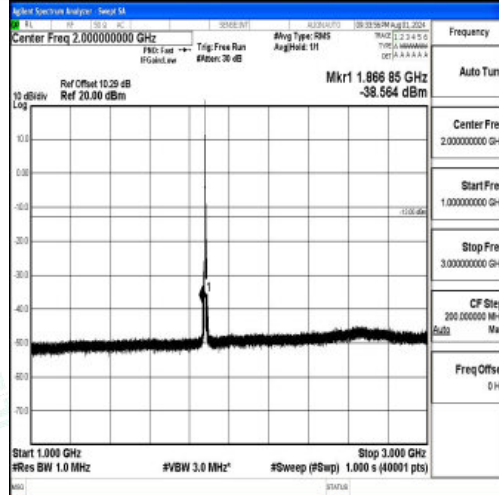
Band2-5MHz-QPSK-18900-1RB#0-1000~3000-PASS
