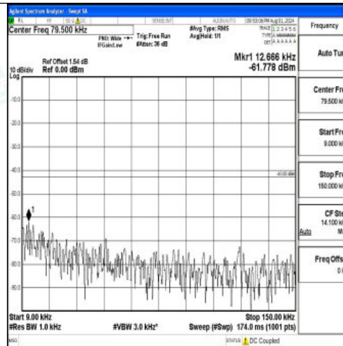
Band2-10MHz-QPSK-18650-1RB#0-0.009~0.15-PASS
