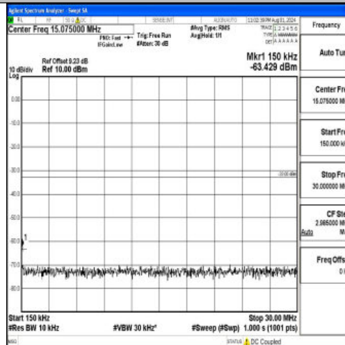
Band2-20MHz-16QAM-19100-1RB#0-0.15~30-PASS
