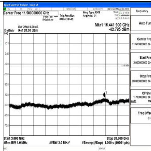
Band2-3MHz-16QAM-18615-1RB#0-3000~20000-PASS
