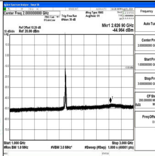
Band2-15MHz-16QAM-19125-1RB#0-1000~3000-PASS
