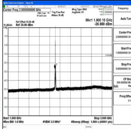
Band2-3MHz-16QAM-19185-1RB#0-1000~3000-PASS
