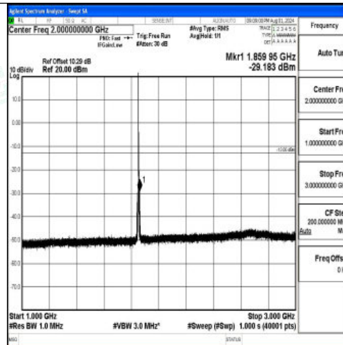
Band2-3MHz-QPSK-18615-1RB#0-1000~3000-PASS
