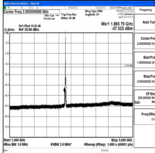
Band2-5MHz-16QAM-19175-1RB#0-1000~3000-PASS
