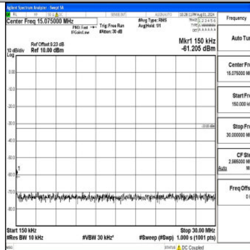
Band2-15MHz-16QAM-19125-1RB#0-0.15~30-PASS
