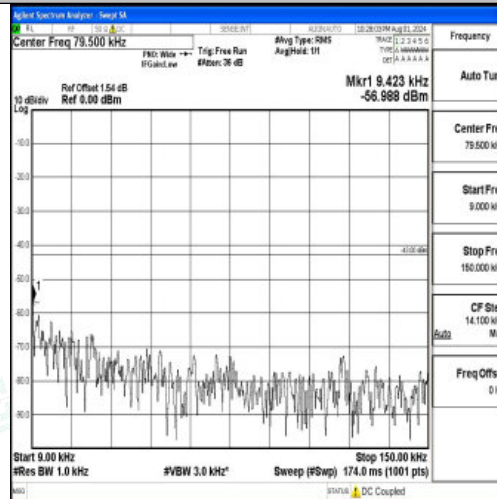
Band2-15MHz-16QAM-19125-1RB#0-0.009~0.15-PASS
