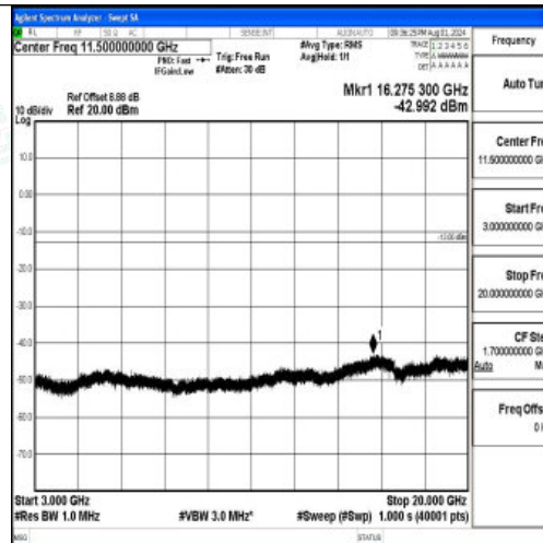
Band2-5MHz-QPSK-19175-1RB#0-3000~20000-PASS
