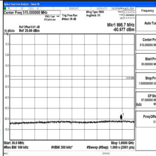
Band2-15MHz-16QAM-18675-1RB#0-30~1000-PASS
