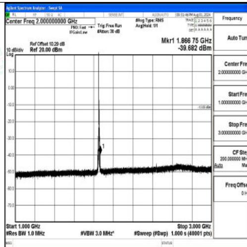
Band2-5MHz-QPSK-18625-1RB#0-1000~3000-PASS
