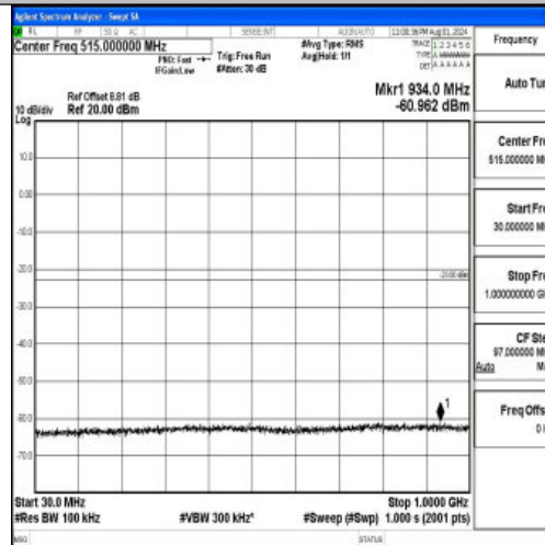
Band2-20MHz-16QAM-18900-1RB#0-30~1000-PASS
