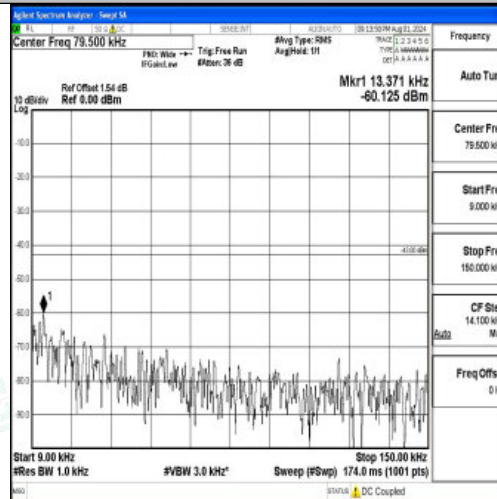
Band2-3MHz-16QAM-19185-1RB#0-0.009~0.15-PASS
