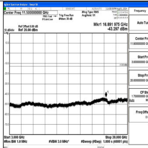
Band2-20MHz-QPSK-18900-1RB#0-3000~20000-PASS
