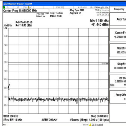
Band2-3MHz-16QAM-19185-1RB#0-0.15~30-PASS
