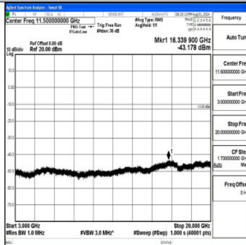
Band2-1.4MHz-16QAM-19193-1RB#0-3000~20000-PASS
