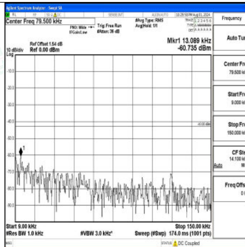
Band2-15MHz-16QAM-18900-1RB#0-0.009~0.15-PASS
