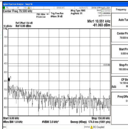
Band2-10MHz-16QAM-18900-1RB#0-0.009~0.15-PASS
