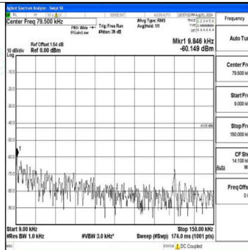
Band2-20MHz-QPSK-18700-1RB#0-0.009~0.15-PASS
