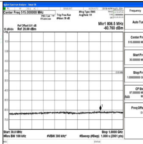
Band2-10MHz-16QAM-19150-1RB#0-30~1000-PASS
