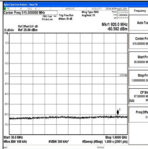
Band2-10MHz-16QAM-18900-1RB#0-30~1000-PASS
