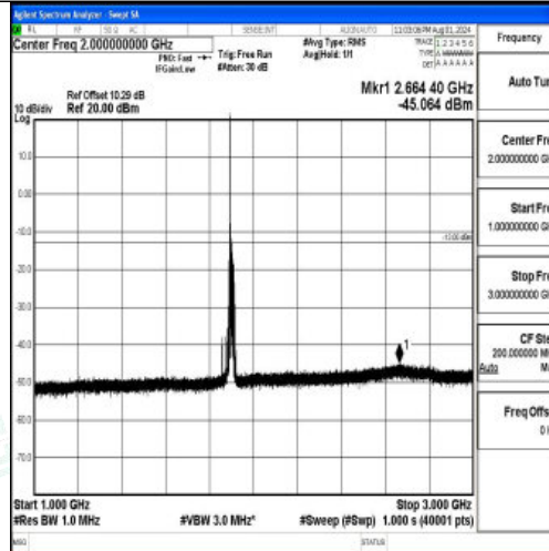
Band2-20MHz-16QAM-19100-1RB#0-1000~3000-PASS
