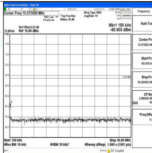
Band2-20MHz-16QAM-18700-1RB#0-0.15~30-PASS
