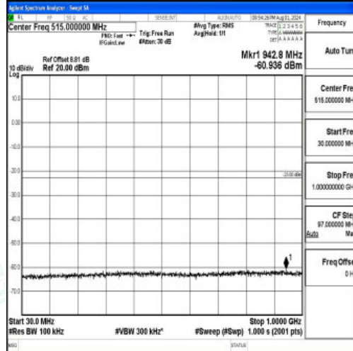
Band2-10MHz-16QAM-18650-1RB#0-30~1000-PASS
