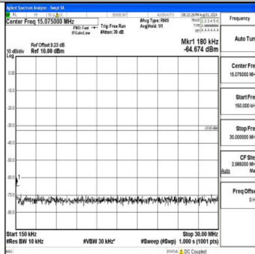
Band2-1.4MHz-16QAM-19193-1RB#0-0.15~30-PASS
