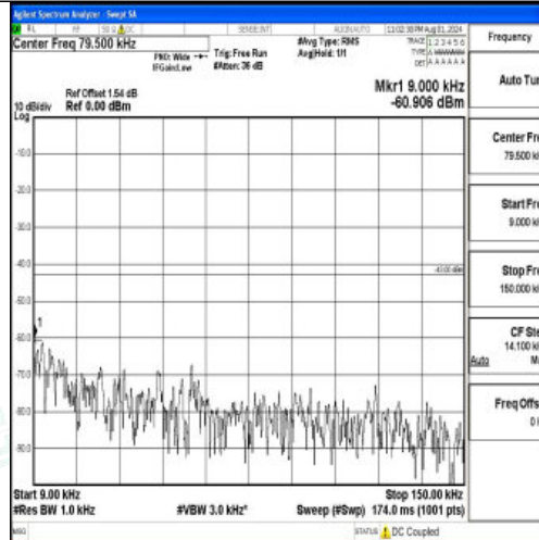
Band2-20MHz-16QAM-19100-1RB#0-0.009~0.15-PASS
