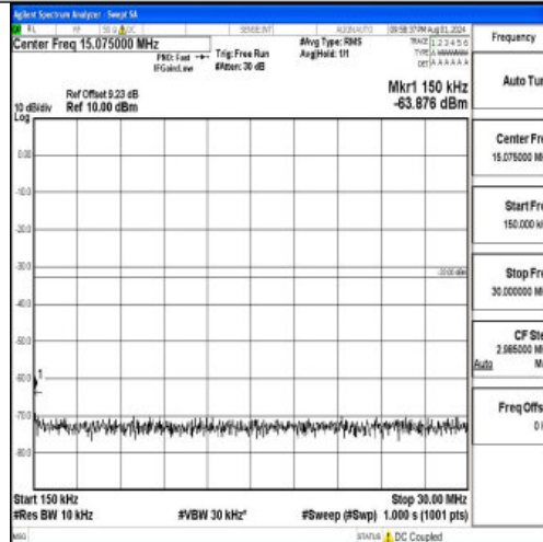
Band2-10MHz-16QAM-19150-1RB#0-0.15~30-PASS
