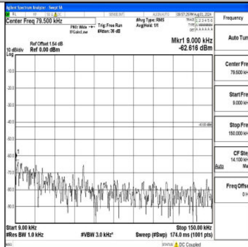
Band2-10MHz-QPSK-19150-1RB#0-0.009~0.15-PASS
