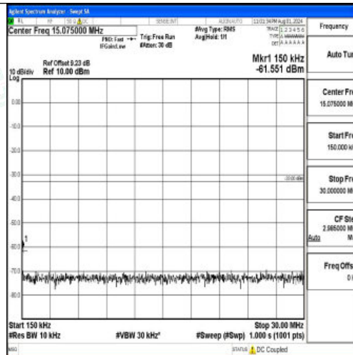
Band2-20MHz-QPSK-19100-1RB#0-0.15~30-PASS
