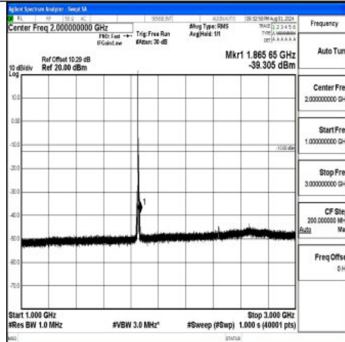
Band2-5MHz-16QAM-18625-1RB#0-1000~3000-PASS
