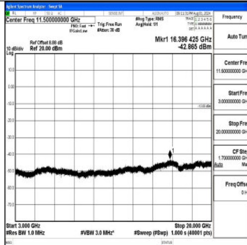
Band2-3MHz-QPSK-18900-1RB#0-3000~20000-PASS
