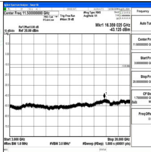
Band2-20MHz-16QAM-18700-1RB#0-3000~20000-PASS
