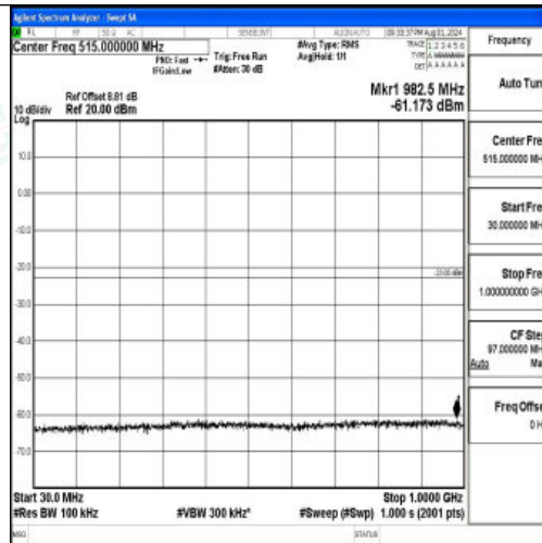
Band2-5MHz-QPSK-18900-1RB#0-30~1000-PASS
