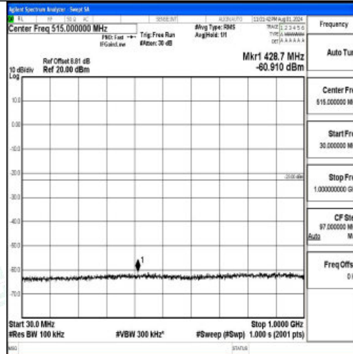
Band2-20MHz-QPSK-19100-1RB#0-30~1000-PASS
