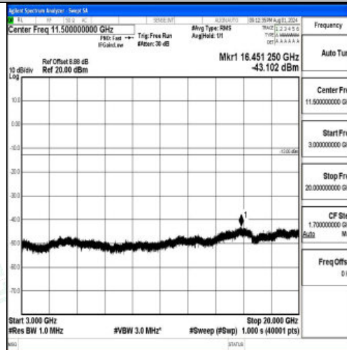
Band2-3MHz-16QAM-18900-1RB#0-3000~20000-PASS
