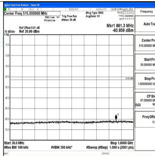
Band2-20MHz-QPSK-18900-1RB#0-30~1000-PASS
