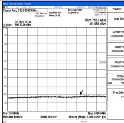
Band2-5MHz-QPSK-18625-1RB#0-30~1000-PASS
