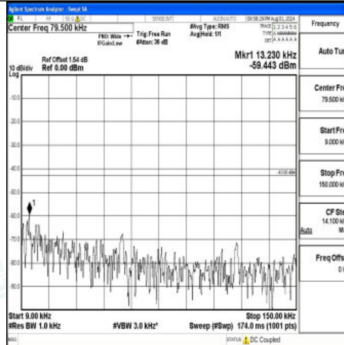
Band2-10MHz-16QAM-19150-1RB#0-0.009~0.15-PASS
