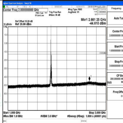
Band2-10MHz-QPSK-18900-1RB#0-1000~3000-PASS
