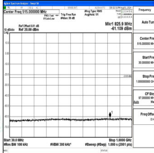
Band2-5MHz-16QAM-18625-1RB#0-30~1000-PASS
