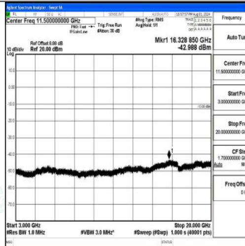
Band2-20MHz-QPSK-18700-1RB#0-3000~20000-PASS
