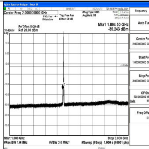
Band2-5MHz-QPSK-19175-1RB#0-1000~3000-PASS
