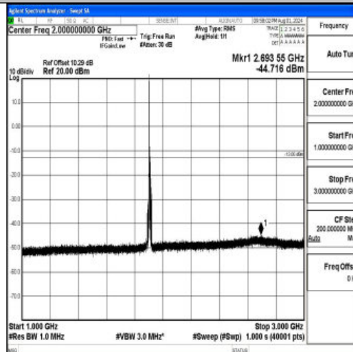
Band2-10MHz-QPSK-19150-1RB#0-1000~3000-PASS
