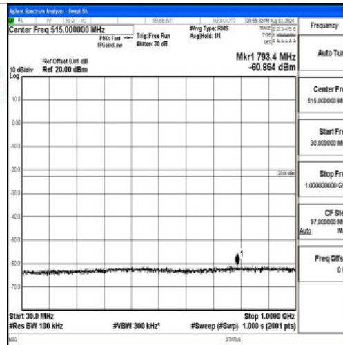
Band2-10MHz-QPSK-18900-1RB#0-30~1000-PASS
