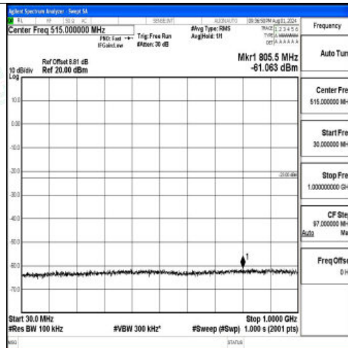
Band2-5MHz-16QAM-19175-1RB#0-30~1000-PASS
