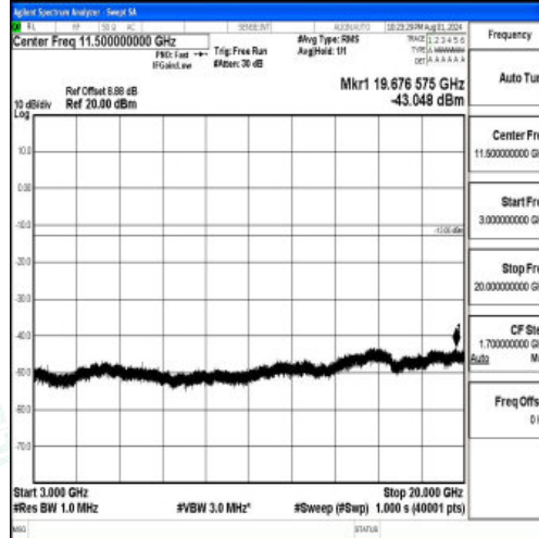
Band2-15MHz-QPSK-18675-1RB#0-3000~20000-PASS
