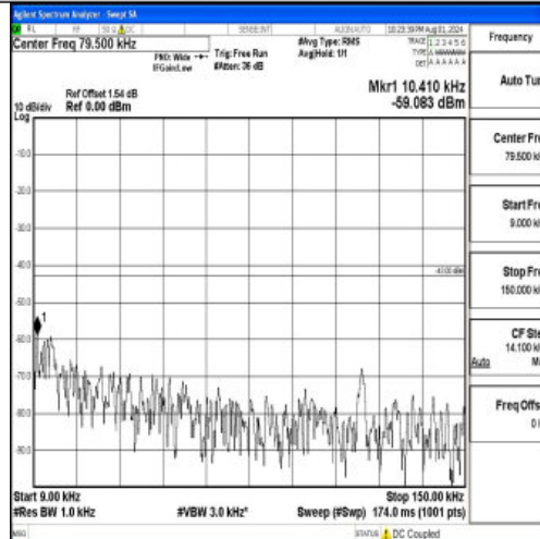
Band2-15MHz-16QAM-18675-1RB#0-0.009~0.15-PASS
