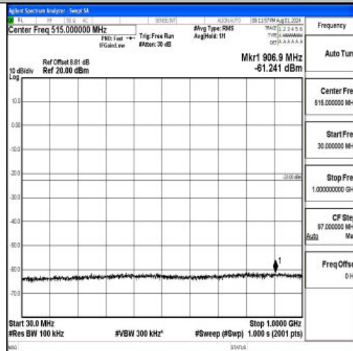
Band2-3MHz-16QAM-18900-1RB#0-30~1000-PASS
