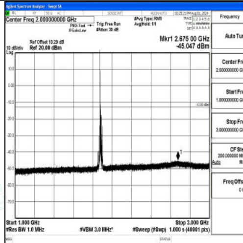
Band2-15MHz-QPSK-18900-1RB#0-1000~3000-PASS
