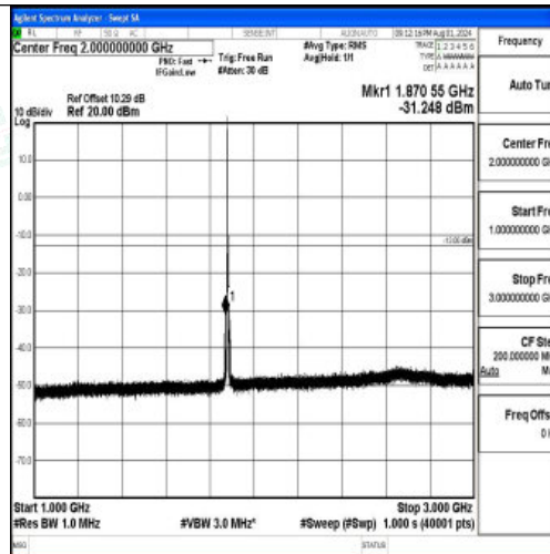
Band2-3MHz-16QAM-18900-1RB#0-1000~3000-PASS
