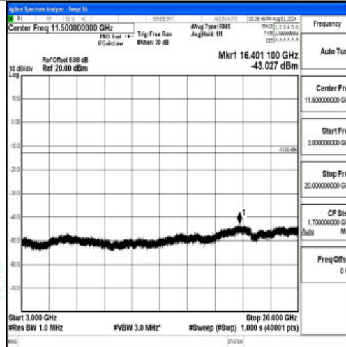
Band2-15MHz-16QAM-18900-1RB#0-3000~20000-PASS
