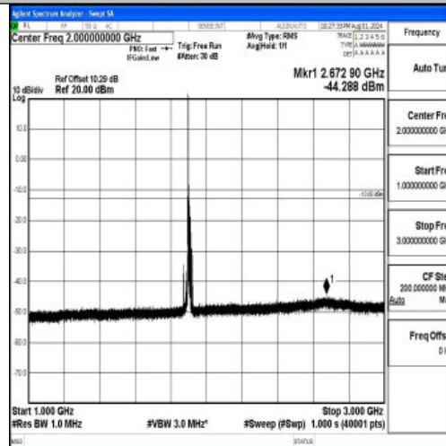
Band2-15MHz-QPSK-19125-1RB#0-1000~3000-PASS
