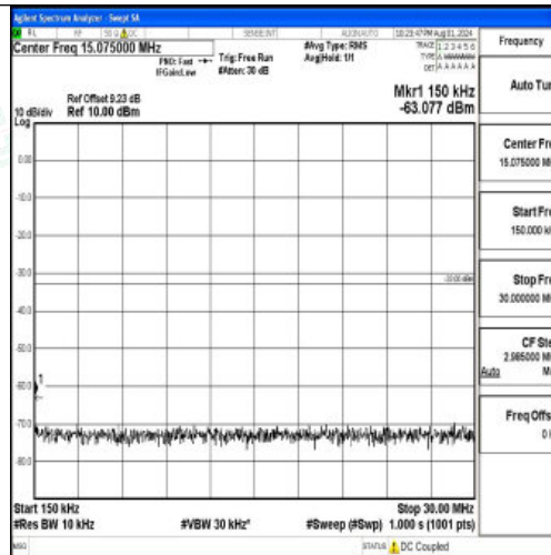
Band2-15MHz-16QAM-18675-1RB#0-0.15~30-PASS
