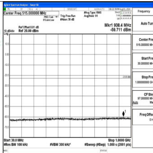
Band2-1.4MHz-16QAM-19193-1RB#0-30~1000-PASS
