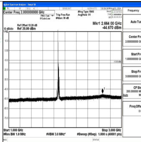
Band2-15MHz-16QAM-18900-1RB#0-1000~3000-PASS
