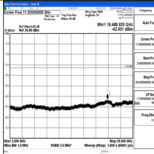
Band2-3MHz-QPSK-18615-1RB#0-3000~20000-PASS
