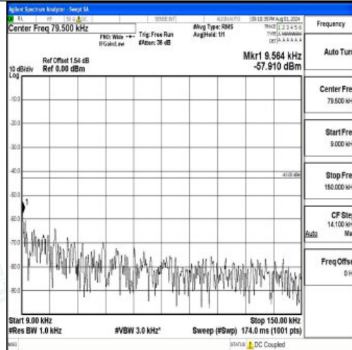
Band2-3MHz-QPSK-18900-1RB#0-0.009~0.15-PASS
