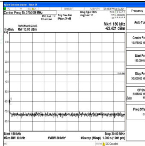
Band2-5MHz-QPSK-19175-1RB#0-0.15~30-PASS
