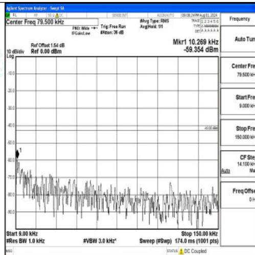
Band2-3MHz-QPSK-18615-1RB#0-0.009~0.15-PASS
