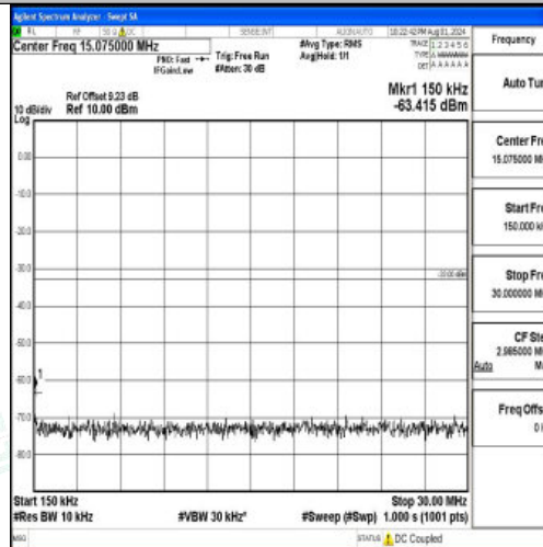
Band2-15MHz-QPSK-18675-1RB#0-0.15~30-PASS
