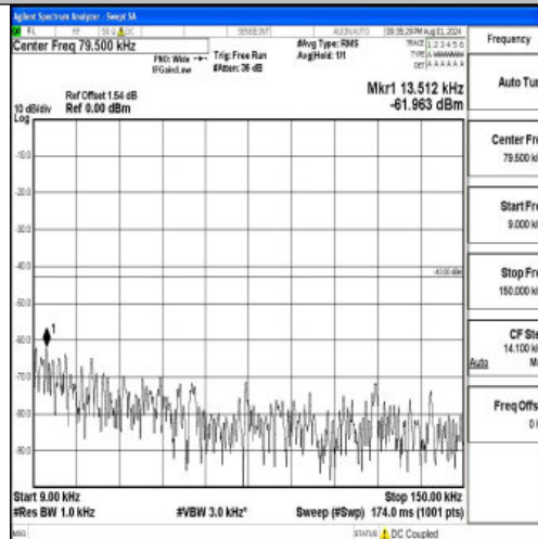
Band2-5MHz-QPSK-19175-1RB#0-0.009~0.15-PASS
