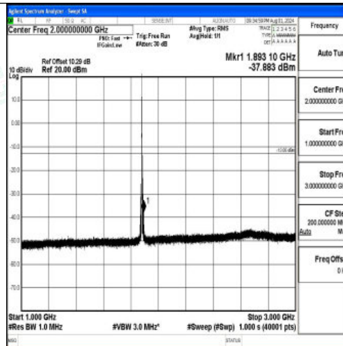
Band2-5MHz-16QAM-18900-1RB#0-1000~3000-PASS
