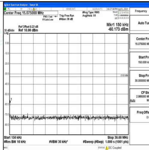
Band2-15MHz-QPSK-19125-1RB#0-0.15~30-PASS
