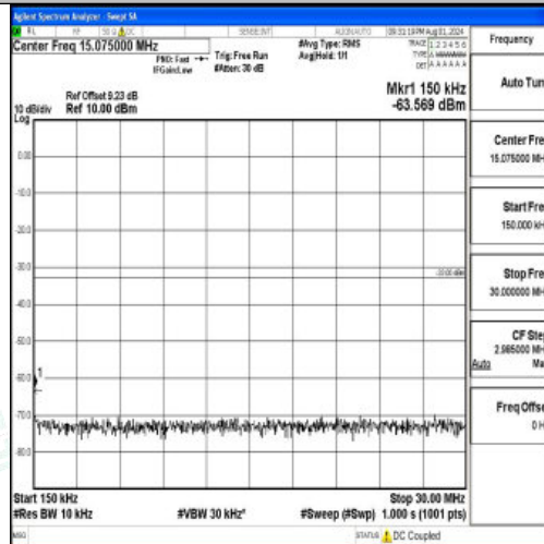
Band2-5MHz-QPSK-18625-1RB#0-0.15~30-PASS
