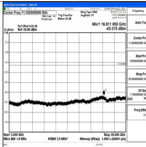
Band2-10MHz-QPSK-19150-1RB#0-3000~20000-PASS
