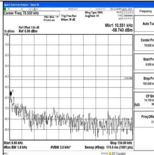
Band2-3MHz-QPSK-19185-1RB#0-0.009~0.15-PASS
