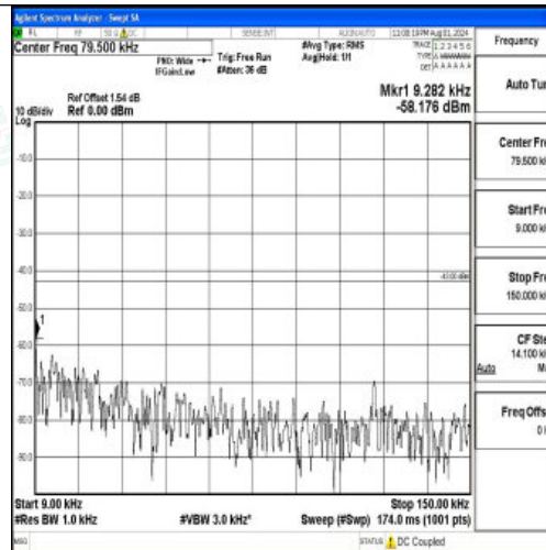
Band2-20MHz-16QAM-18900-1RB#0-0.009~0.15-PASS
