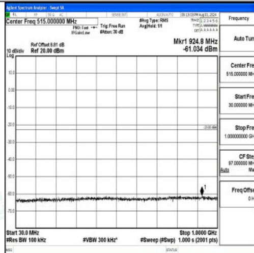
Band2-3MHz-QPSK-19185-1RB#0-30~1000-PASS
