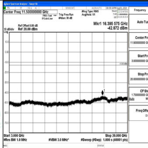
Band2-5MHz-16QAM-18900-1RB#0-3000~20000-PASS
