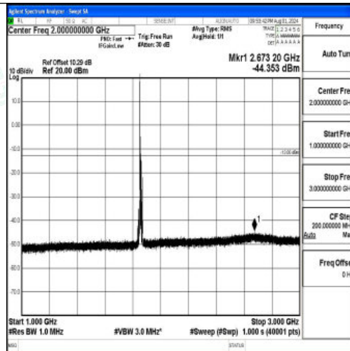
Band2-10MHz-QPSK-18650-1RB#0-1000~3000-PASS
