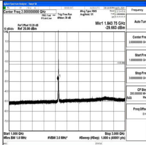
Band2-3MHz-16QAM-18615-1RB#0-1000~3000-PASS
