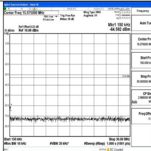
Band2-10MHz-QPSK-18900-1RB#0-0.15~30-PASS
