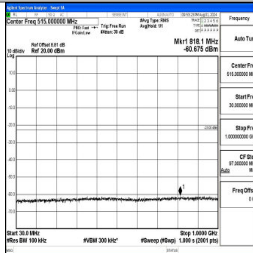
Band2-10MHz-QPSK-18650-1RB#0-30~1000-PASS
