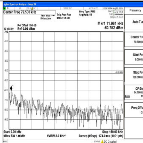
Band2-15MHz-QPSK-19125-1RB#0-0.009~0.15-PASS
