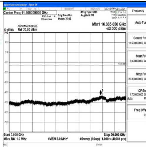
Band2-15MHz-16QAM-18675-1RB#0-3000~20000-PASS
