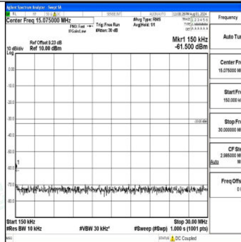
Band2-20MHz-16QAM-18900-1RB#0-0.15~30-PASS
