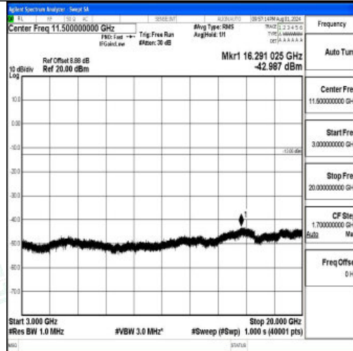
Band2-10MHz-16QAM-18900-1RB#0-3000~20000-PASS
