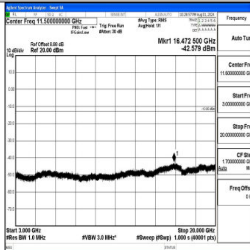
Band2-15MHz-16QAM-19125-1RB#0-3000~20000-PASS
