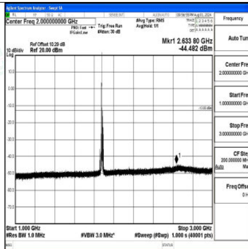
Band2-10MHz-16QAM-18900-1RB#0-1000~3000-PASS
