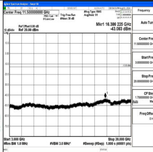
Band2-10MHz-QPSK-18650-1RB#0-3000~20000-PASS
