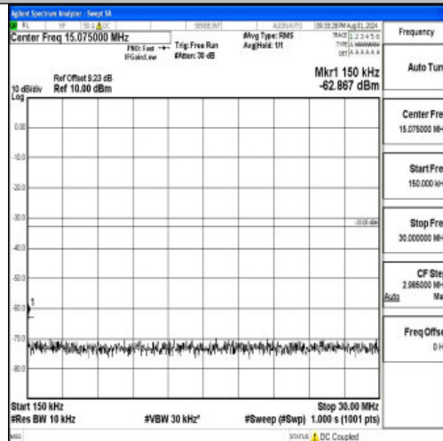
Band2-5MHz-QPSK-18900-1RB#0-0.15~30-PASS
