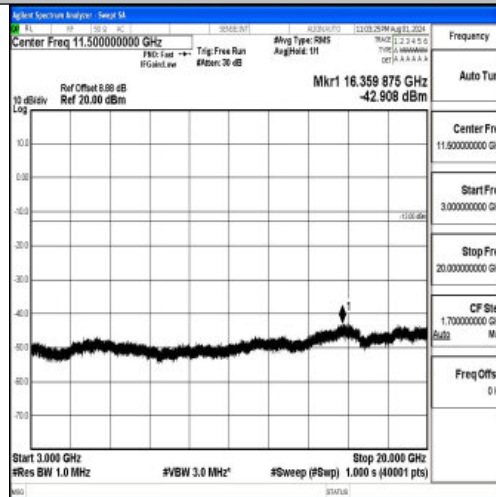
Band2-20MHz-16QAM-19100-1RB#0-3000~20000-PASS
