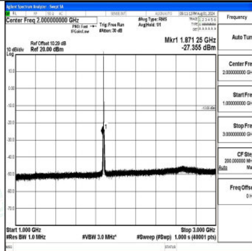
Band2-3MHz-QPSK-18900-1RB#0-1000~3000-PASS
