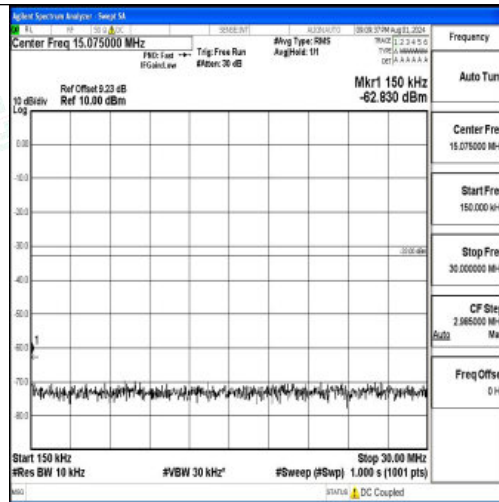
Band2-3MHz-16QAM-18615-1RB#0-0.15~30-PASS
