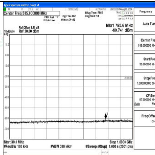
Band2-3MHz-QPSK-18900-1RB#0-30~1000-PASS
