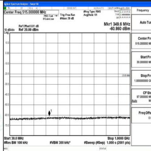
Band2-15MHz-QPSK-19125-1RB#0-30~1000-PASS
