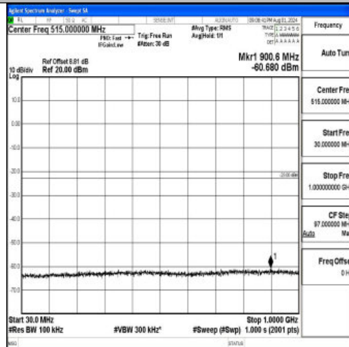
Band2-3MHz-QPSK-18615-1RB#0-30~1000-PASS
