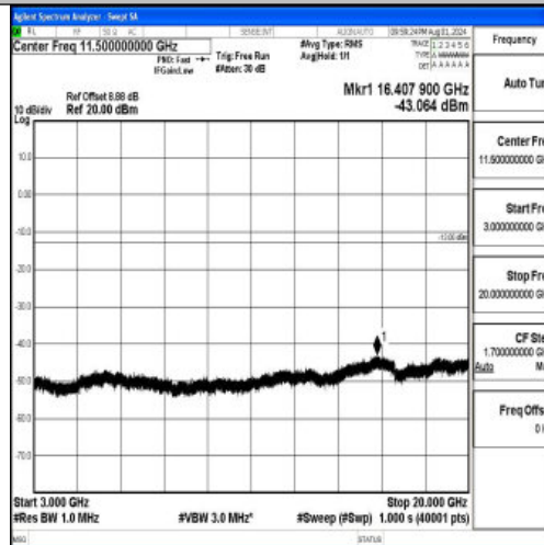
Band2-10MHz-16QAM-19150-1RB#0-3000~20000-PASS
