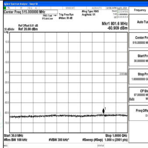
Band2-20MHz-16QAM-18700-1RB#0-30~1000-PASS
