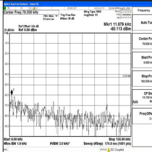
Band2-15MHz-QPSK-18900-1RB#0-0.009~0.15-PASS
