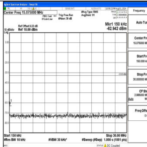
Band2-20MHz-QPSK-18900-1RB#0-0.15~30-PASS
