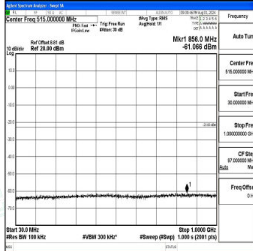
Band2-3MHz-16QAM-18615-1RB#0-30~1000-PASS
