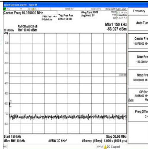
Band2-5MHz-16QAM-18625-1RB#0-0.15~30-PASS
