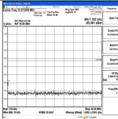
Band2-10MHz-QPSK-18650-1RB#0-0.15~30-PASS
