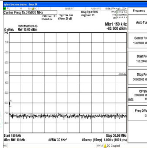
Band2-10MHz-16QAM-18900-1RB#0-0.15~30-PASS
