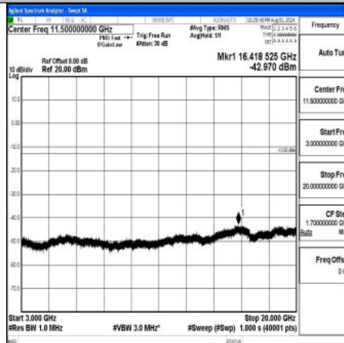
Band2-15MHz-QPSK-18900-1RB#0-3000~20000-PASS
