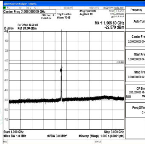
Band2-1.4MHz-16QAM-19193-1RB#0-1000~3000-PASS
