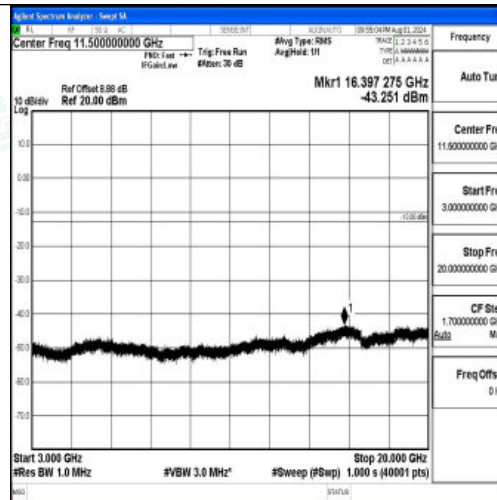
Band2-10MHz-16QAM-18650-1RB#0-3000~20000-PASS
