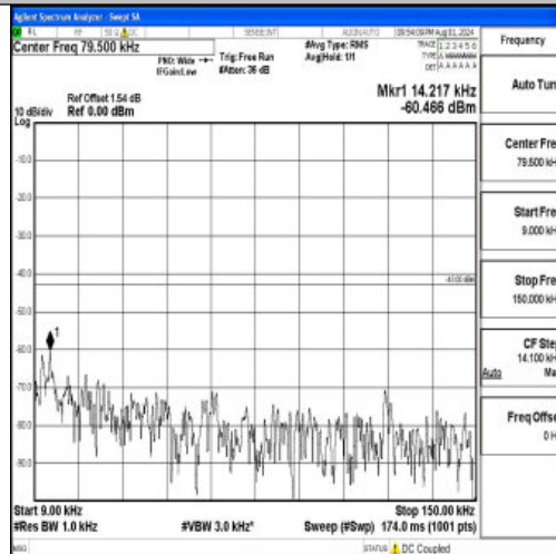
Band2-10MHz-16QAM-18650-1RB#0-0.009~0.15-PASS
