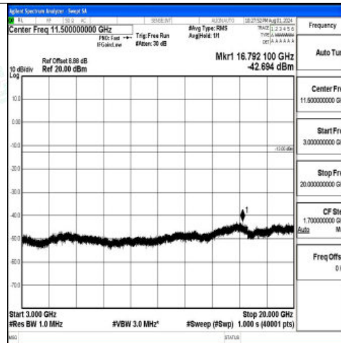
Band2-15MHz-QPSK-19125-1RB#0-3000~20000-PASS
