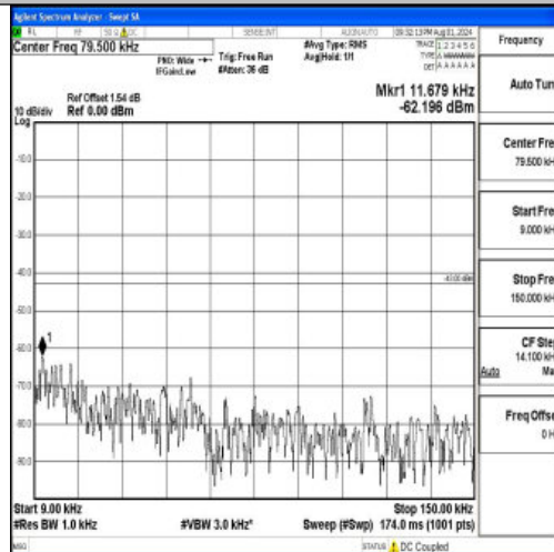
Band2-5MHz-16QAM-18625-1RB#0-0.009~0.15-PASS
