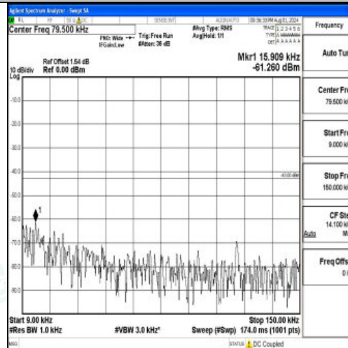
Band2-5MHz-16QAM-19175-1RB#0-0.009~0.15-PASS
