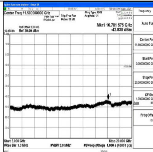
Band2-10MHz-QPSK-18900-1RB#0-3000~20000-PASS
