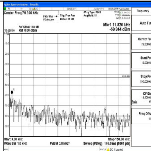
Band2-3MHz-16QAM-18615-1RB#0-0.009~0.15-PASS
