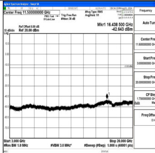
Band2-5MHz-QPSK-18900-1RB#0-3000~20000-PASS
