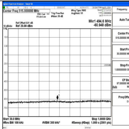
Band2-15MHz-16QAM-18900-1RB#0-30~1000-PASS
