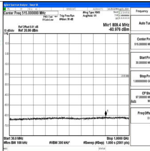
Band2-15MHz-QPSK-18900-1RB#0-30~1000-PASS
