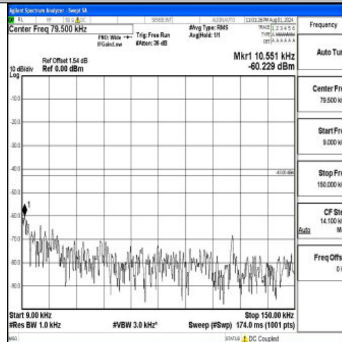
Band2-20MHz-QPSK-19100-1RB#0-0.009~0.15-PASS
