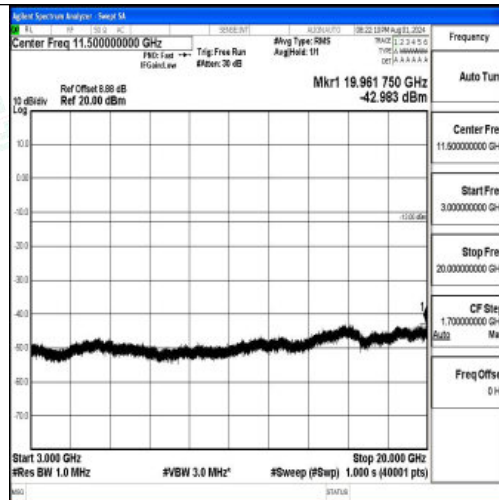
Band2-1.4MHz-QPSK-19193-1RB#0-3000~20000-PASS
