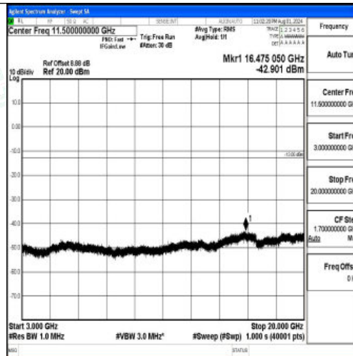
Band2-20MHz-QPSK-19100-1RB#0-3000~20000-PASS
