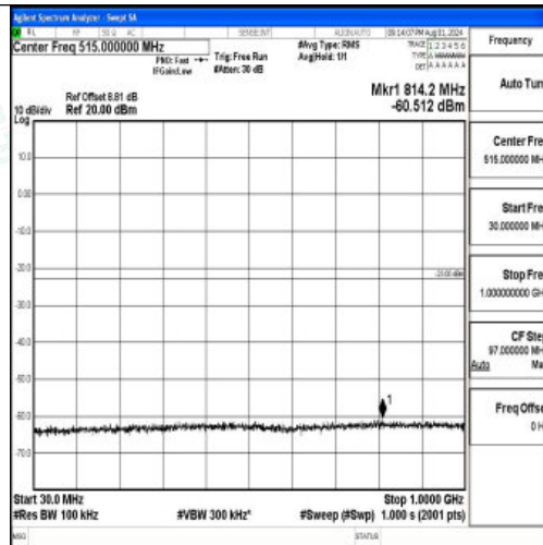
Band2-3MHz-16QAM-19185-1RB#0-30~1000-PASS
