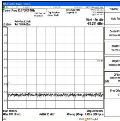
Band2-10MHz-QPSK-19150-1RB#0-0.15~30-PASS
