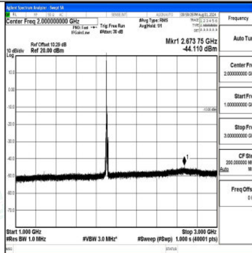
Band2-10MHz-16QAM-19150-1RB#0-1000~3000-PASS
