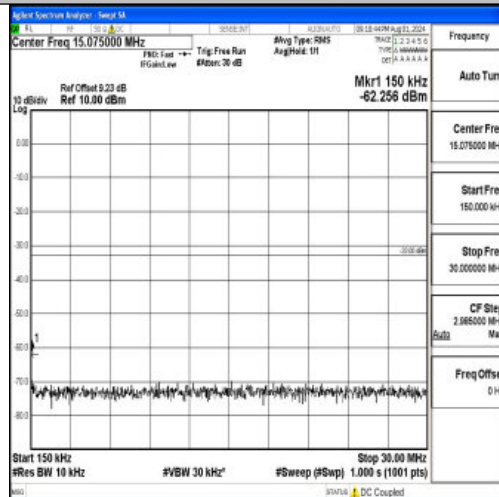
Band2-3MHz-QPSK-18900-1RB#0-0.15~30-PASS
