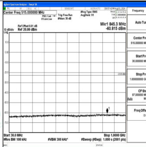
Band2-10MHz-QPSK-19150-1RB#0-30~1000-PASS
