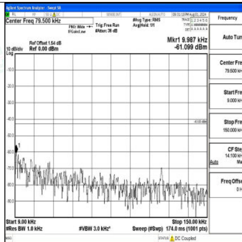
Band2-5MHz-QPSK-18625-1RB#0-0.009~0.15-PASS
