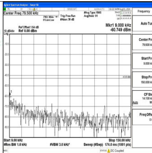
Band2-15MHz-QPSK-18675-1RB#0-0.009~0.15-PASS
