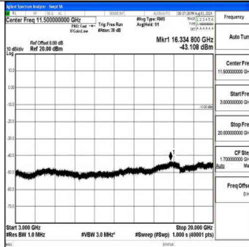
Band2-5MHz-16QAM-19175-1RB#0-3000~20000-PASS
