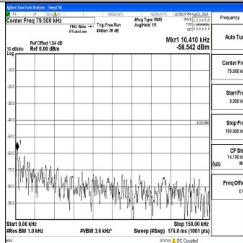
Band2-20MHz-16QAM-18700-1RB#0-0.009~0.15-PASS
