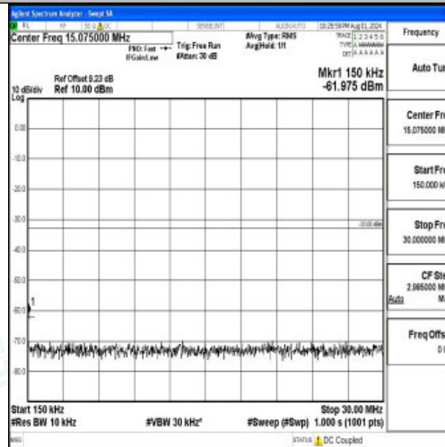
Band2-15MHz-16QAM-18900-1RB#0-0.15~30-PASS
