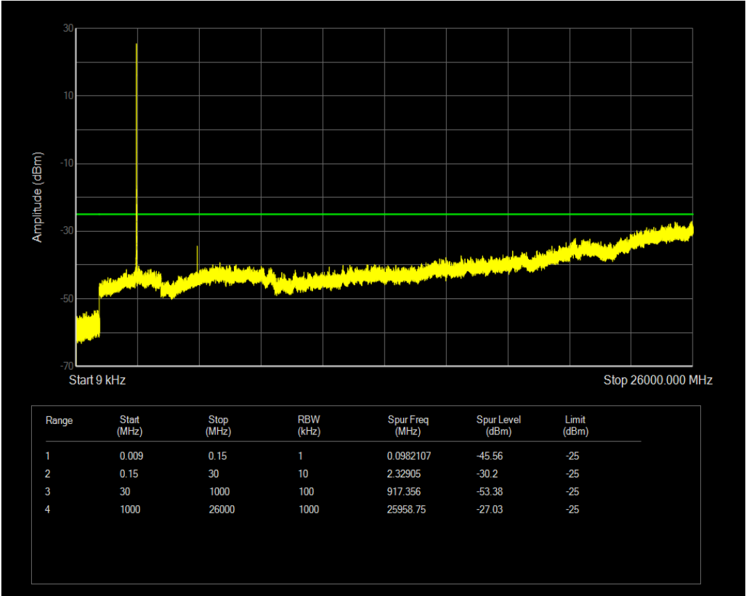
Band7 QPSK BW=15MHz Channel=21375 RB Size=1 Position=#Mid
