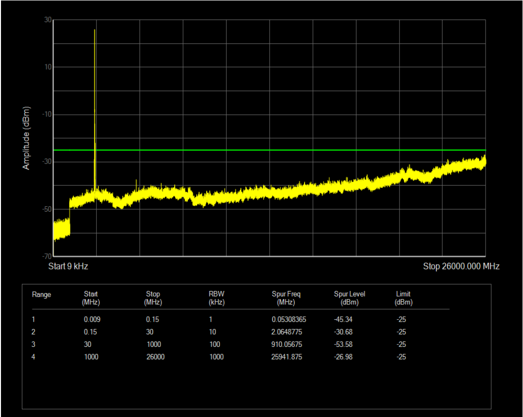
Band7 QPSK BW=20MHz Channel=20850 RB Size=1 Position=#Mid
