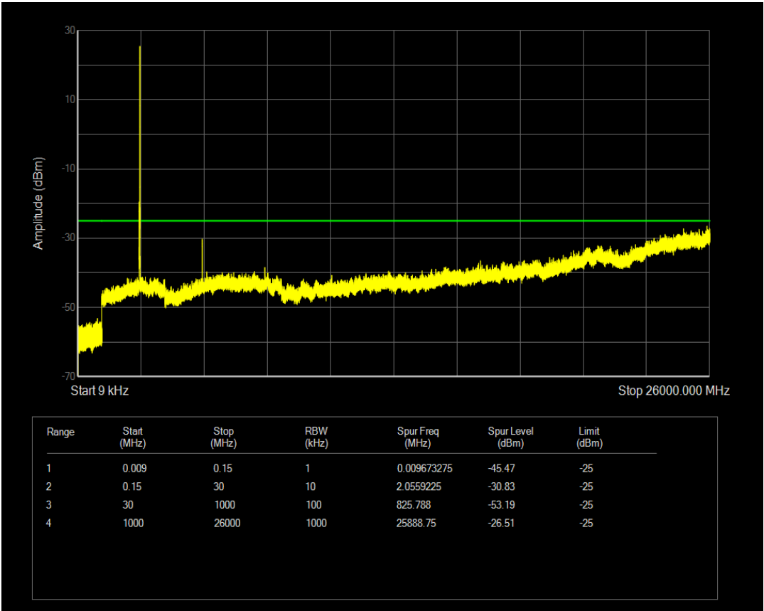
Band7 QAM16 BW=15MHz Channel=21375 RB Size=36 Position=#0
