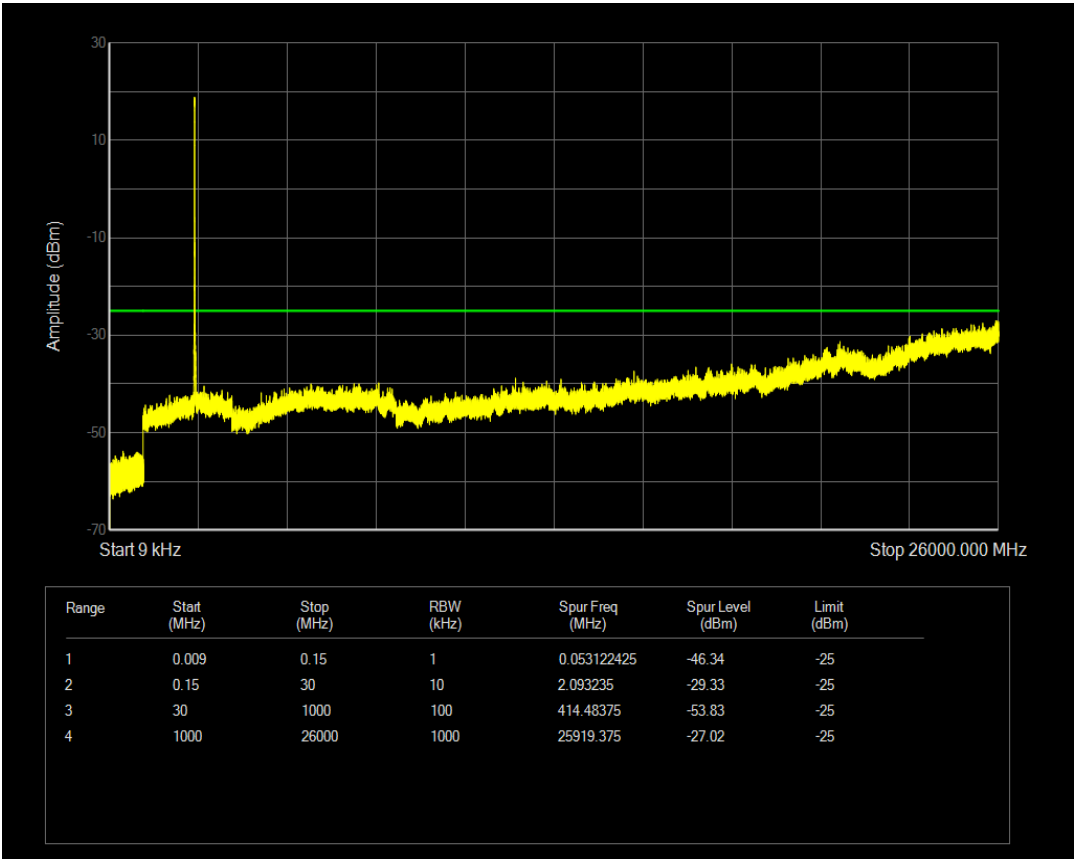
Band7 QAM16 BW=20MHz Channel=20850 RB Size=50 Position=#0
