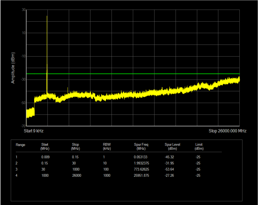
Band7 QPSK BW=15MHz Channel=21100 RB Size=1 Position=#Mid
