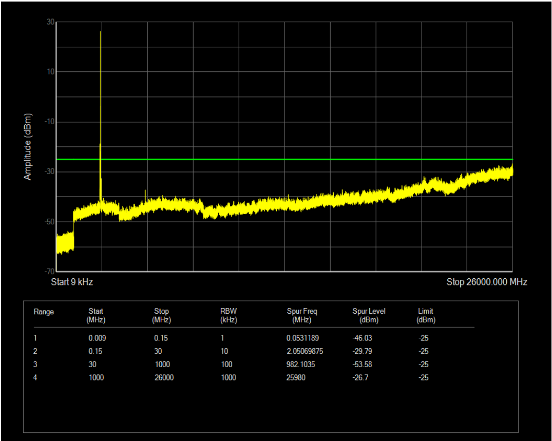
Band7 QAM16 BW=20MHz Channel=21100 RB Size=50 Position=#0
