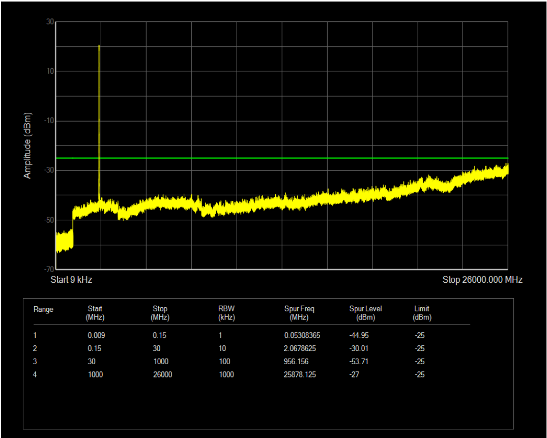
Band7 QAM16 BW=15MHz Channel=20825 RB Size=36 Position=#0
