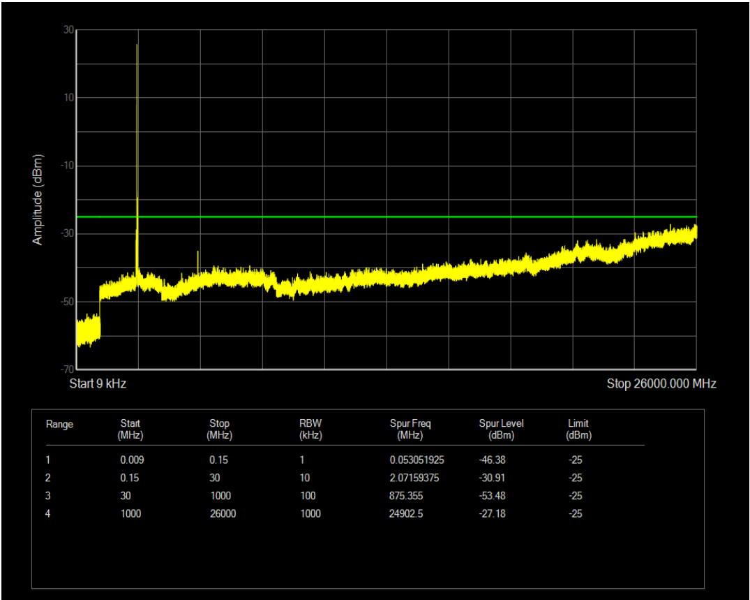
Band7 QPSK BW=20MHz Channel=21350 RB Size=1 Position=#Mid
