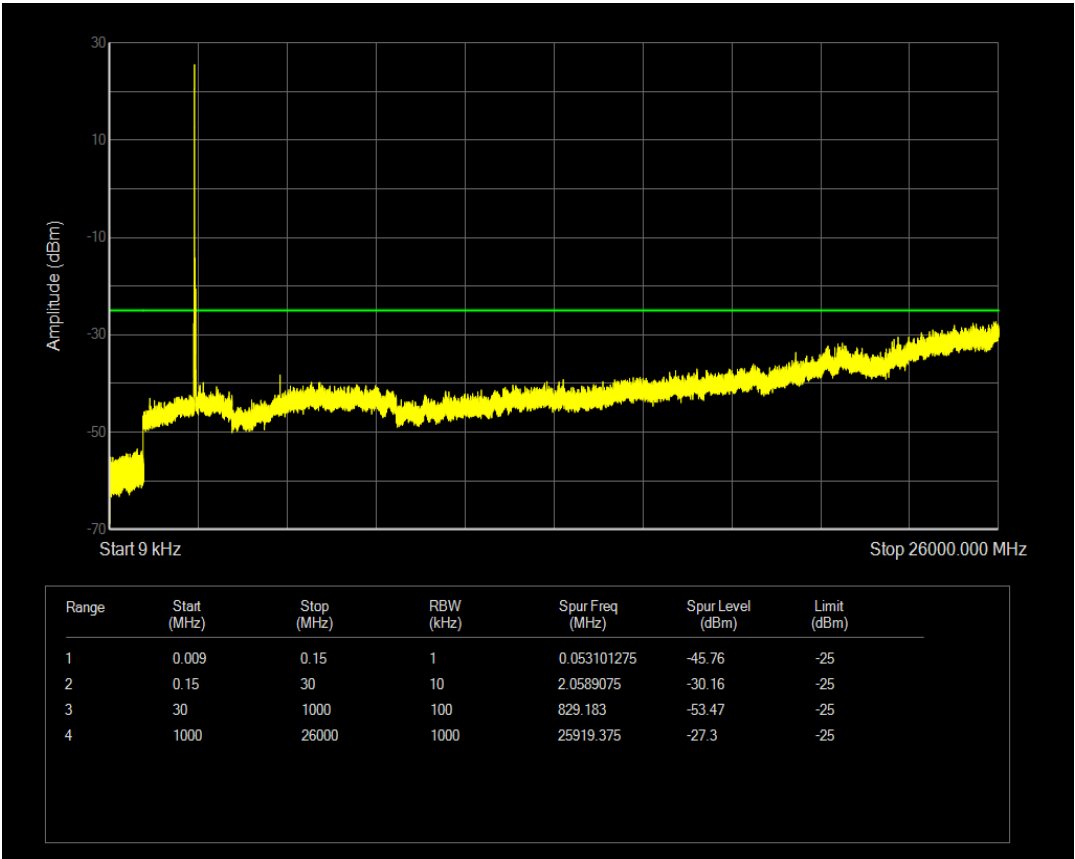
Band7 QAM16 BW=20MHz Channel=20850 RB Size=1 Position=#Mid
