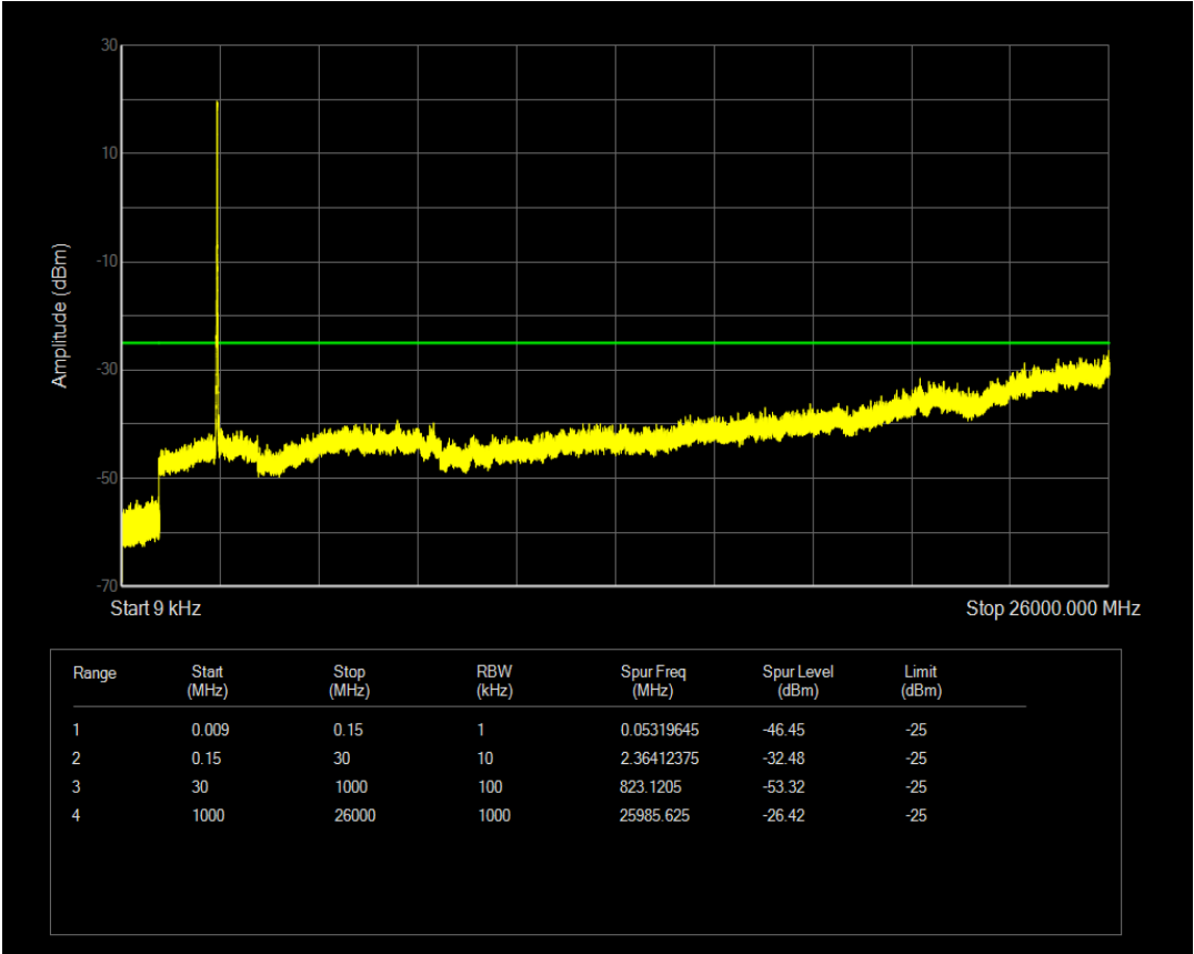
Band7 QPSK BW=20MHz Channel=21100 RB Size=50 Position=#0
