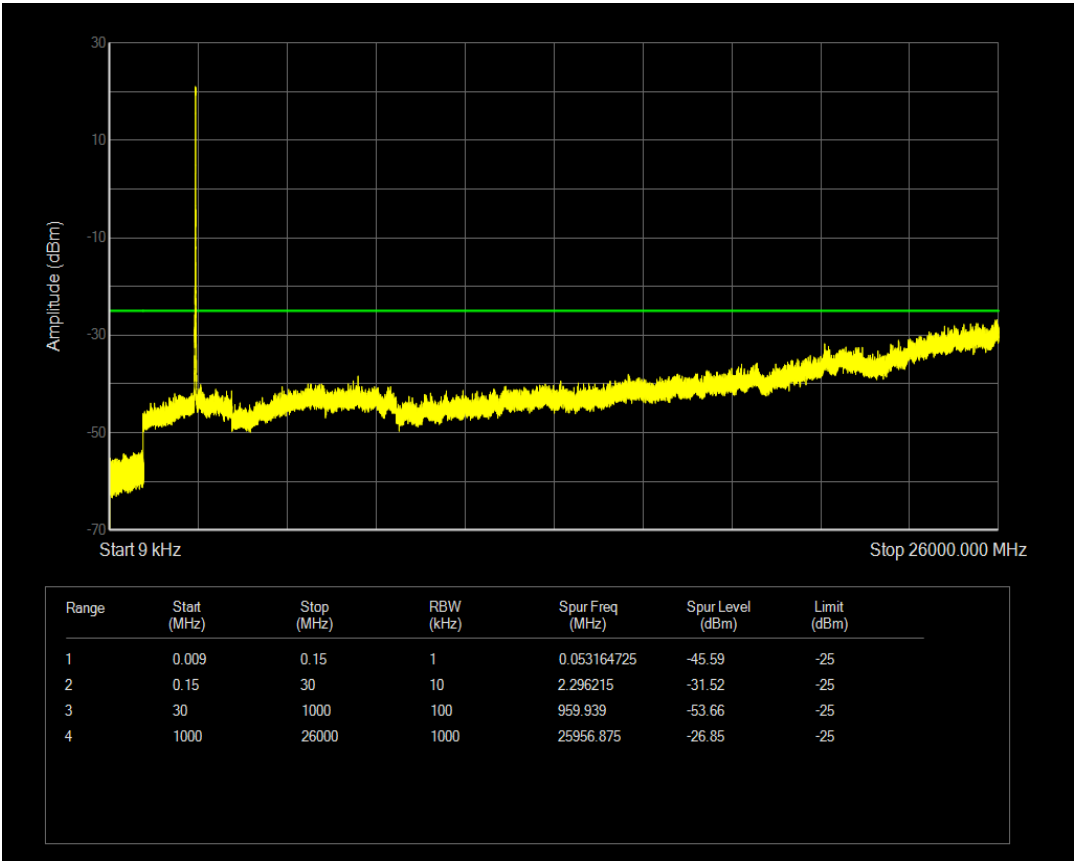
Band7 QPSK BW=15MHz Channel=21100 RB Size=36 Position=#0
