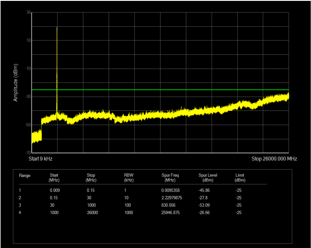
Band7 QAM16 BW=20MHz Channel=21350 RB Size=50 Position=#0
