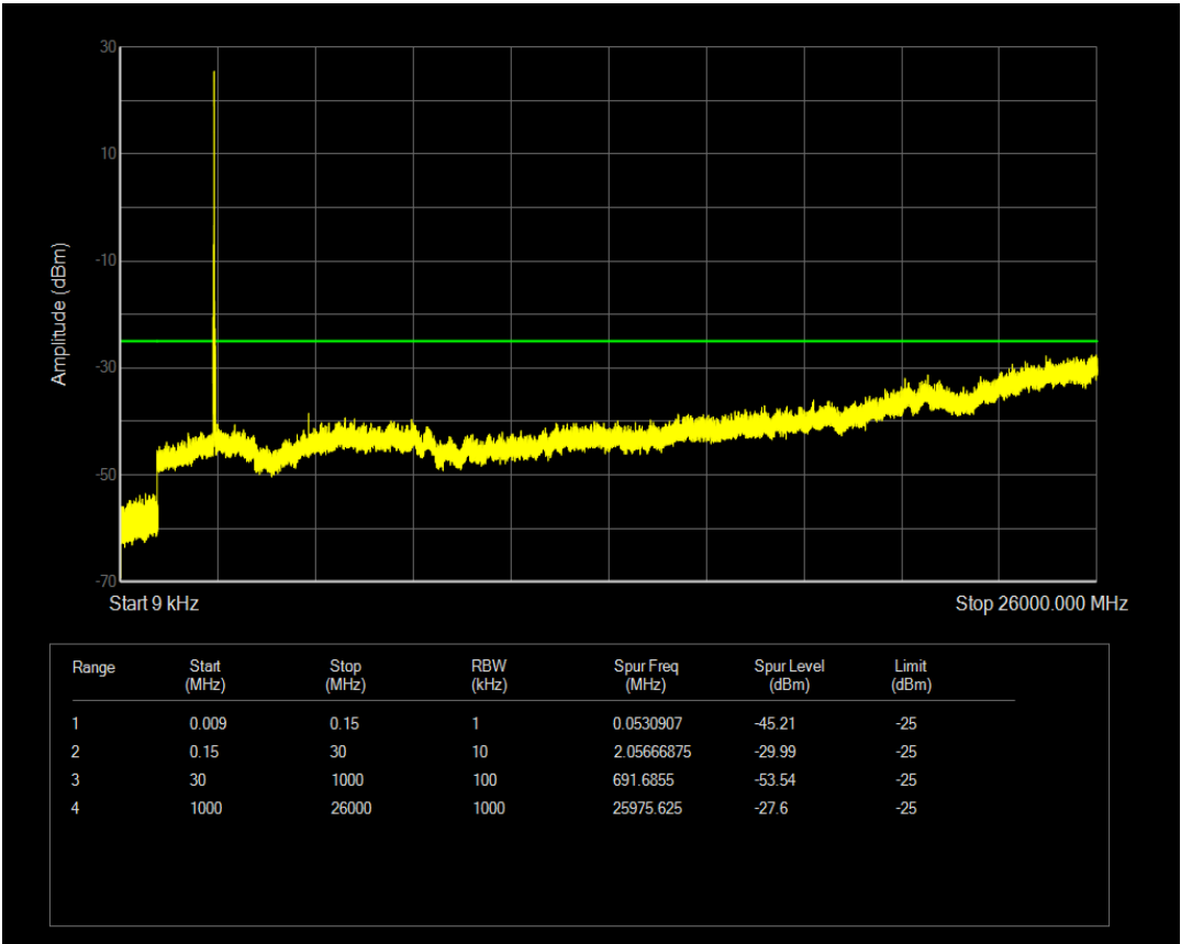
Band7 QPSK BW=15MHz Channel=20825 RB Size=36 Position=#0
