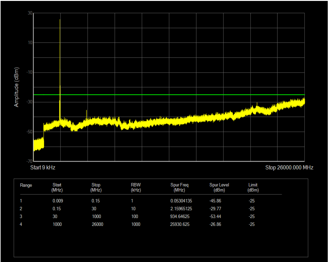
Band7 QAM16 BW=20MHz Channel=21350 RB Size=1 Position=#Mid
