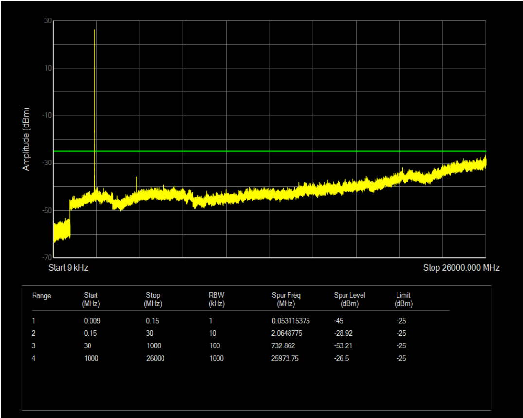
Band7 QAM16 BW=15MHz Channel=20825 RB Size=1 Position=#Mid
