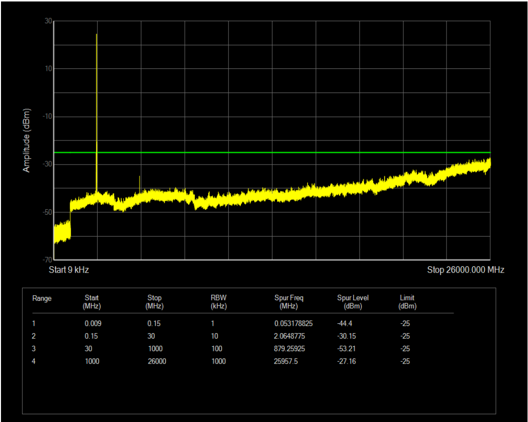
Band7 QAM16 BW=10MHz Channel=21400 RB Size=1 Position=#Mid
