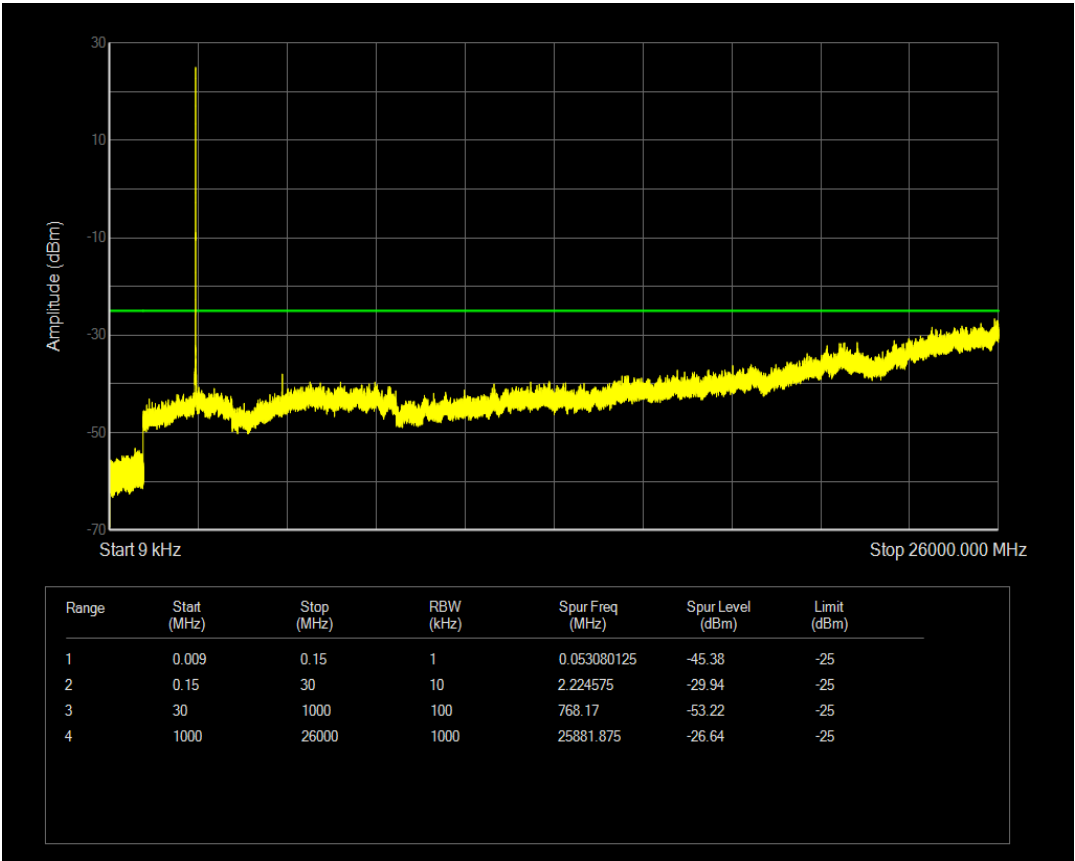
Band7 QPSK BW=20MHz Channel=21100 RB Size=1 Position=#Mid
