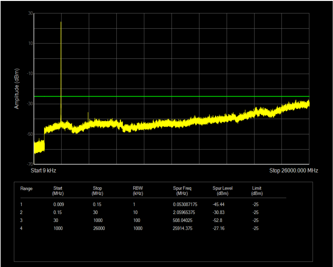
Band7 QAM16 BW=15MHz Channel=21375 RB Size=1 Position=#Mid
