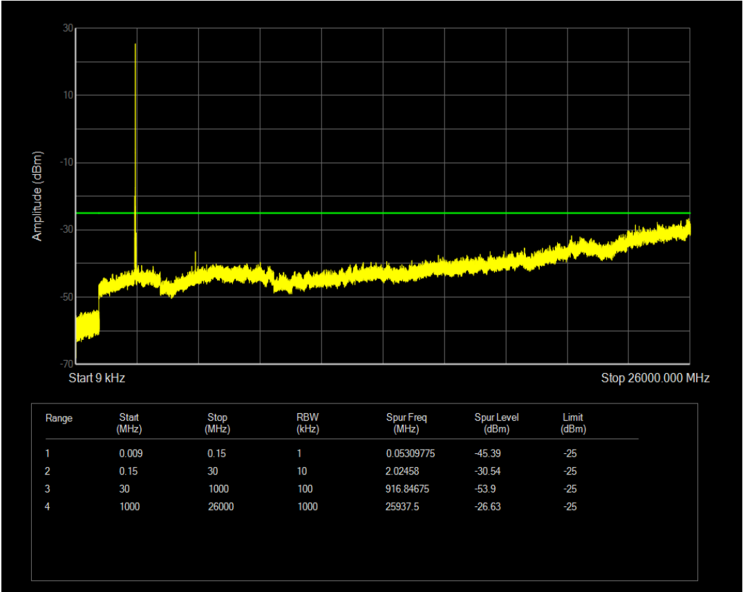
Band7 QAM16 BW=15MHz Channel=21100 RB Size=36 Position=#0
