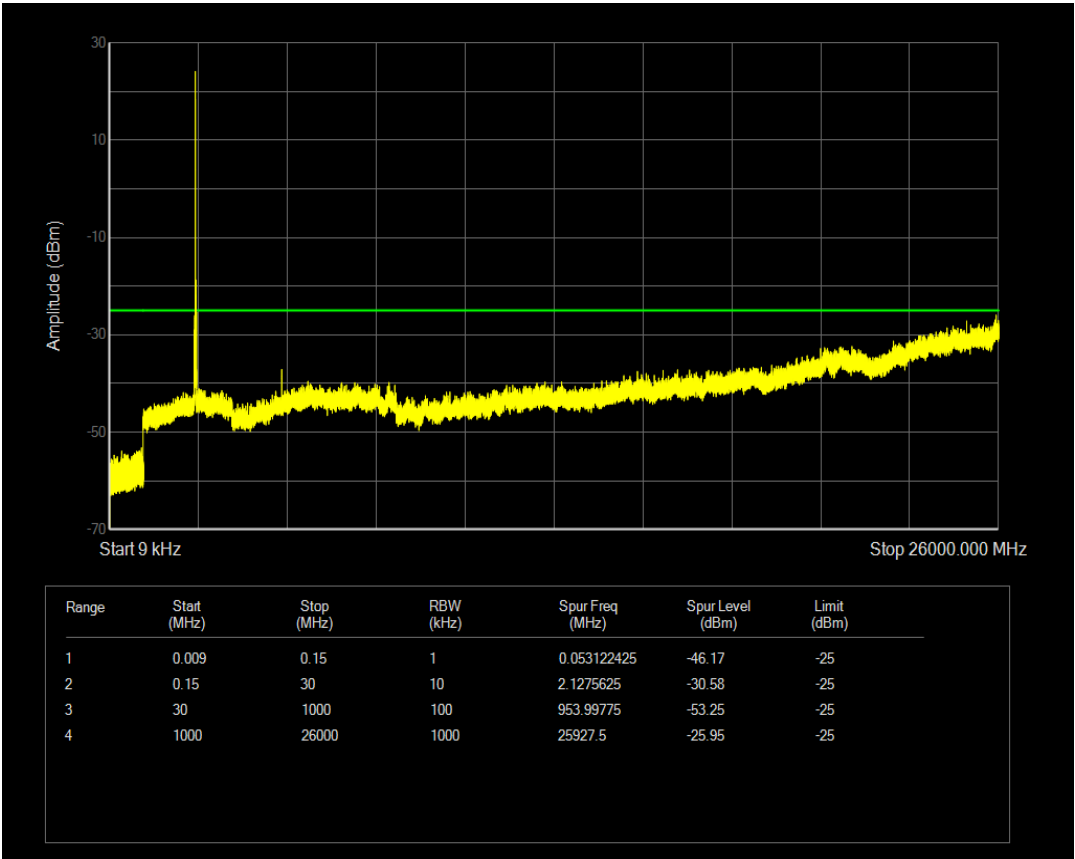
Band7 QAM16 BW=20MHz Channel=21100 RB Size=1 Position=#Mid
