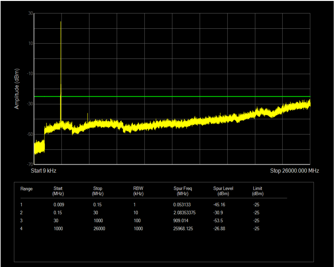
Band7 QAM16 BW=15MHz Channel=21100 RB Size=1 Position=#Mid
