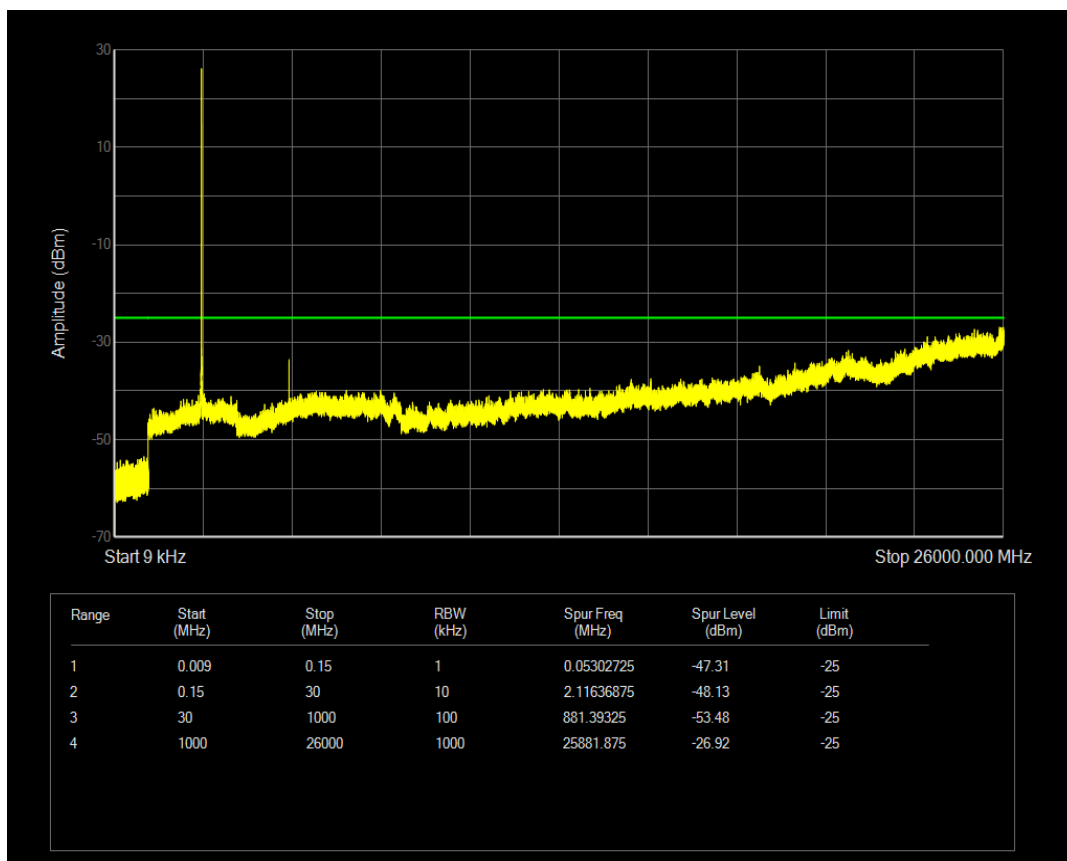
Band7 QAM16 BW=20MHz Channel=21350 RB Size=1 Position=#Mid
