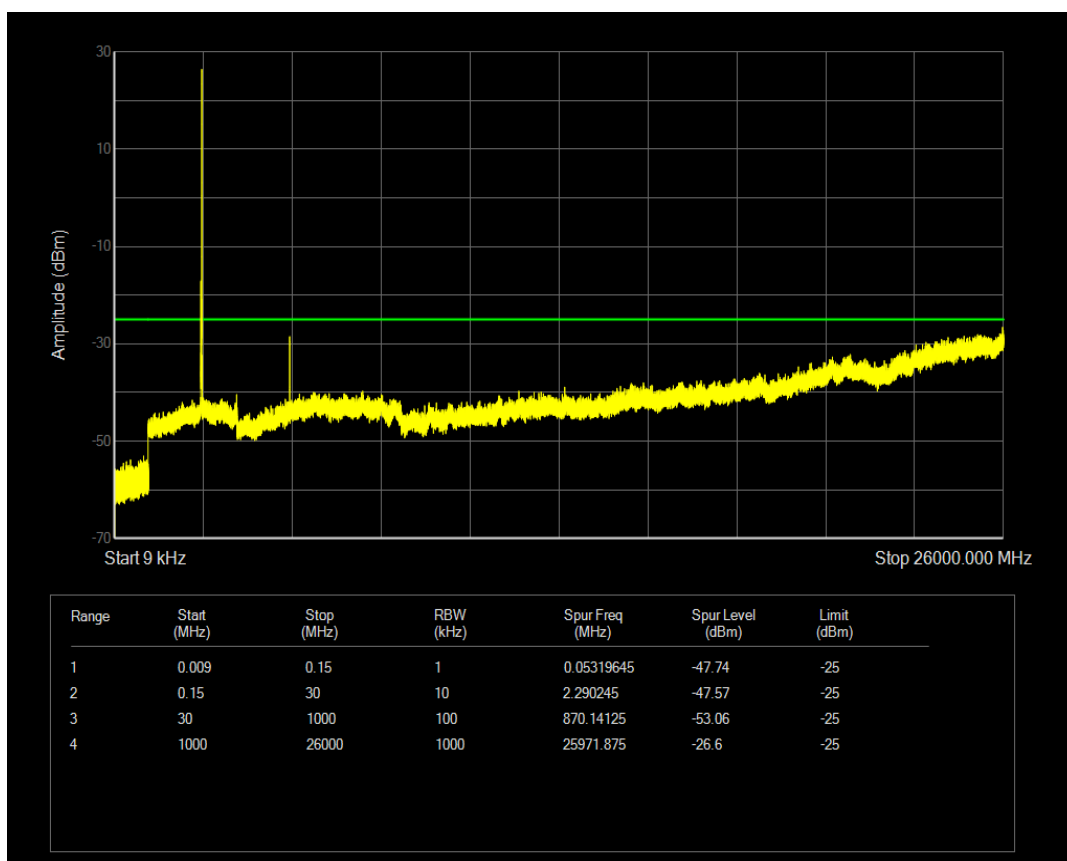
Band7 QPSK BW=15MHz Channel=21375 RB Size=36 Position=#0
