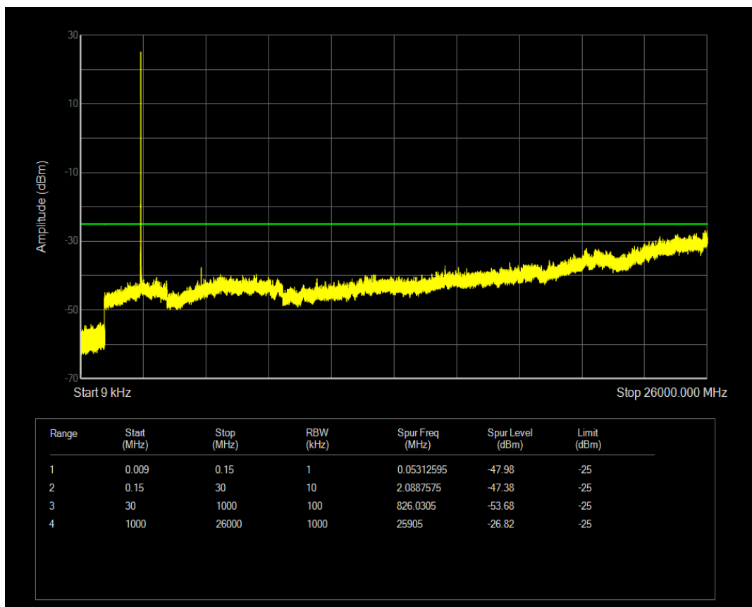
Band7 QAM16 BW=20MHz Channel=20850 RB Size=1 Position=#Mid
