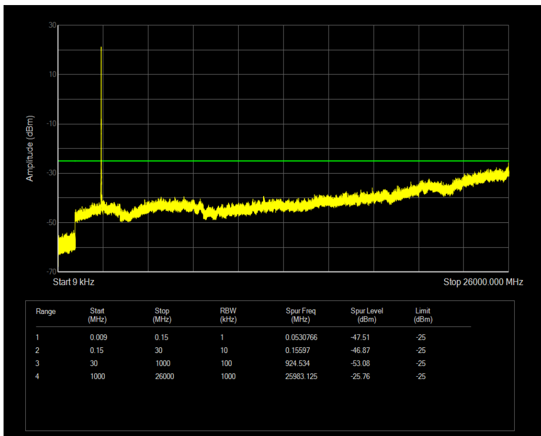
Band7 QPSK BW=15MHz Channel=20825 RB Size=36 Position=#0
