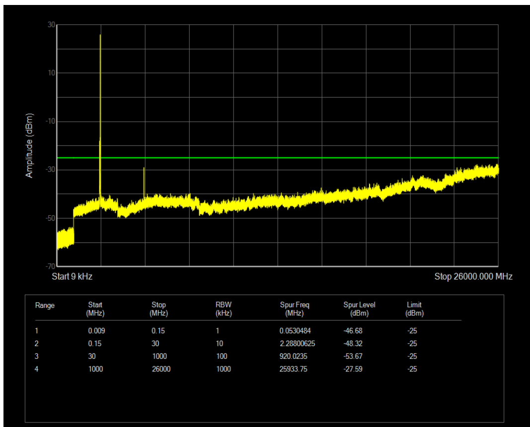
Band7 QPSK BW=20MHz Channel=21350 RB Size=50 Position=#0
