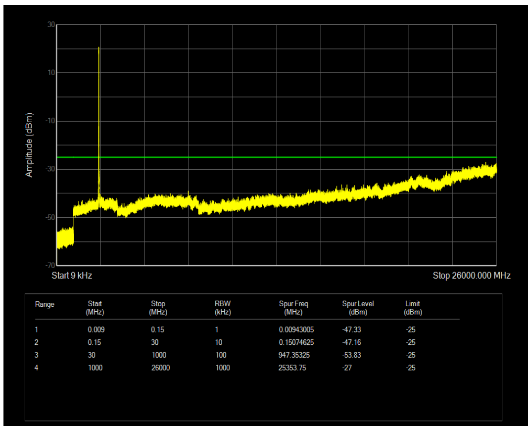
Band7 QAM16 BW=20MHz Channel=20850 RB Size=50 Position=#0
