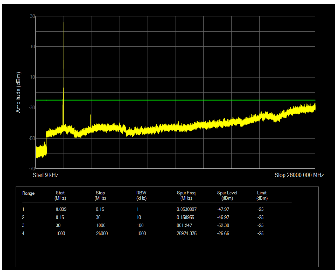
Band7 QPSK BW=15MHz Channel=21375 RB Size=1 Position=#Mid
