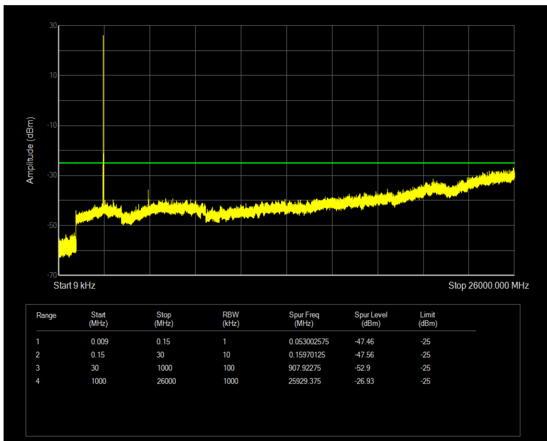
Band7 QAM16 BW=10MHz Channel=21400 RB Size=1 Position=#Mid
