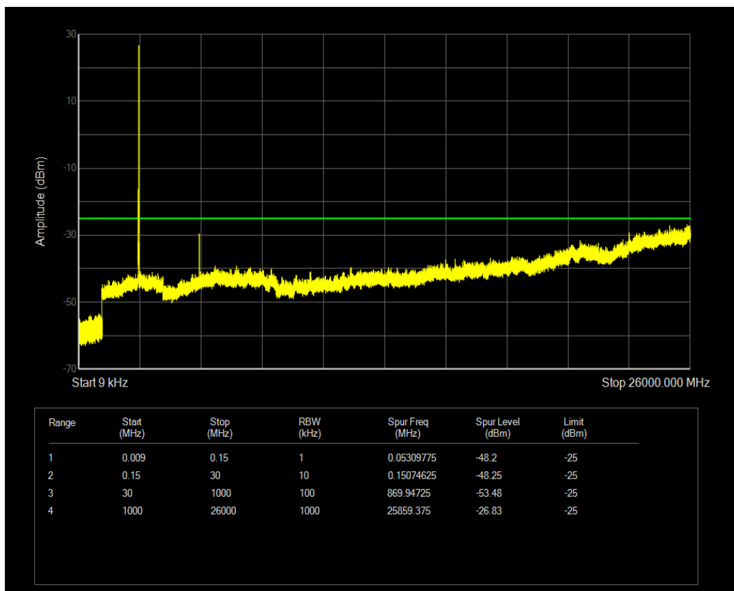
Band7 QAM16 BW=15MHz Channel=21375 RB Size=36 Position=#0
