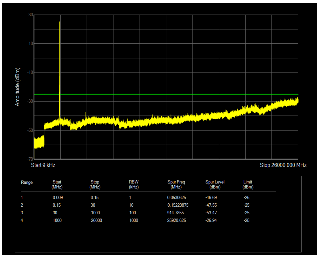
Band7 QAM16 BW=20MHz Channel=21100 RB Size=1 Position=#Mid
