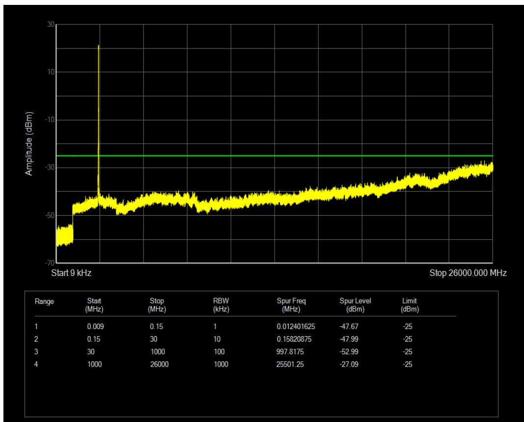
Band7 QAM16 BW=15MHz Channel=21100 RB Size=36 Position=#0
