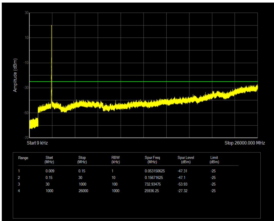
Band7 QPSK BW=20MHz Channel=21100 RB Size=50 Position=#0
