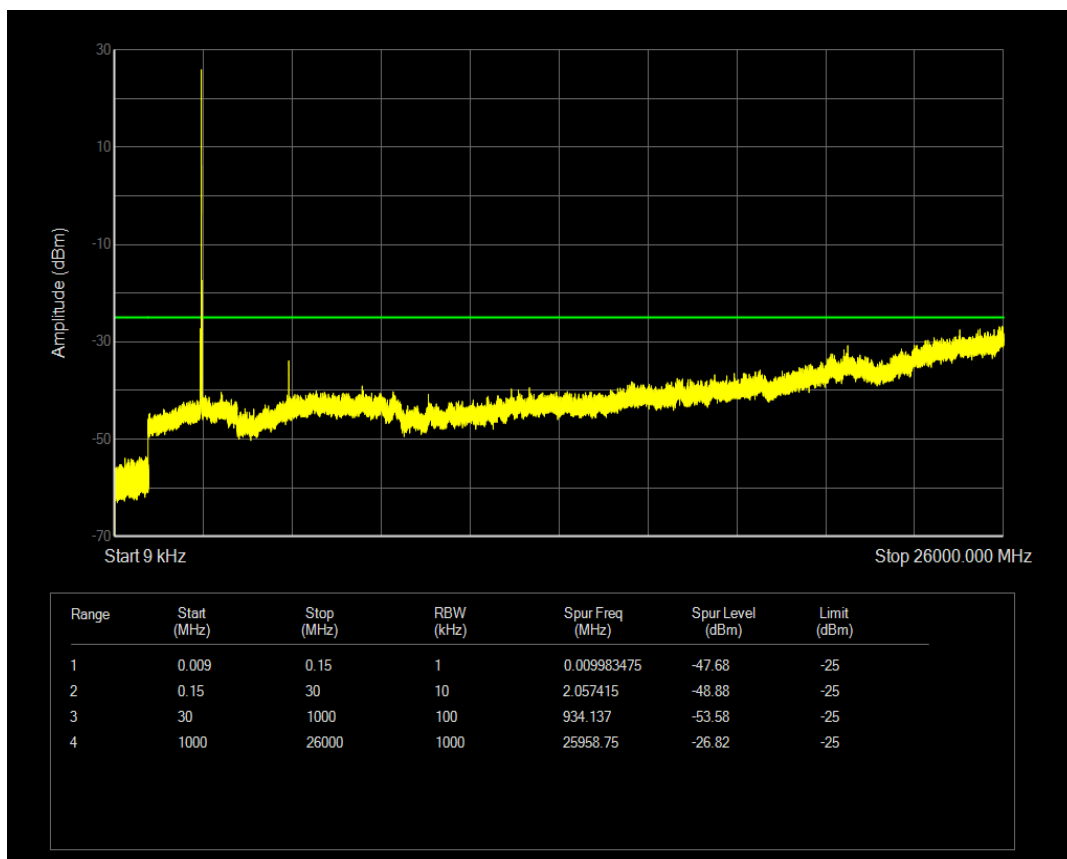
Band7 QAM16 BW=15MHz Channel=21375 RB Size=1 Position=#Mid
