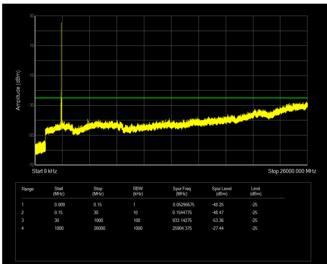
Band7 QPSK BW=20MHz Channel=20850 RB Size=50 Position=#0
