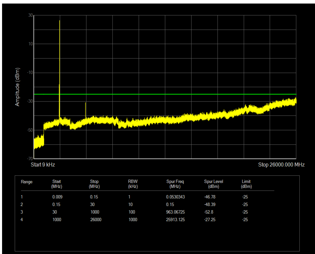
Band7 QAM16 BW=20MHz Channel=21350 RB Size=50 Position=#0
