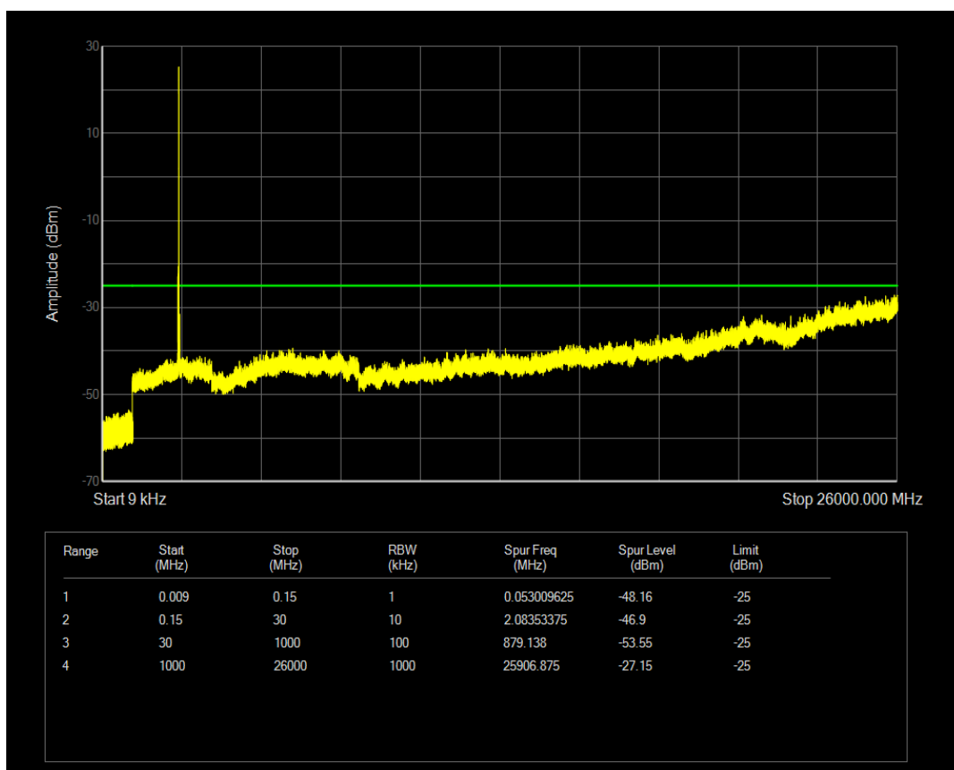
Band7 QAM16 BW=15MHz Channel=20825 RB Size=36 Position=#0
