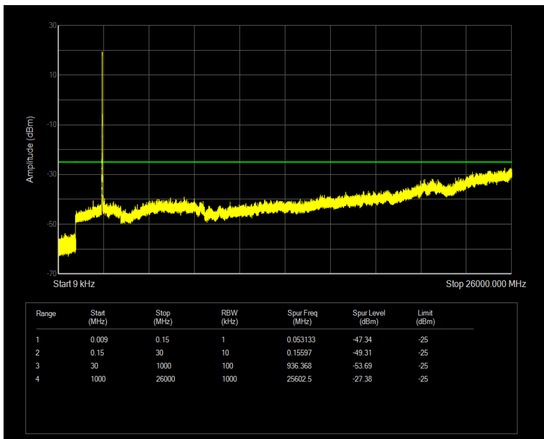
Band7 QAM16 BW=20MHz Channel=21100 RB Size=50 Position=#0
