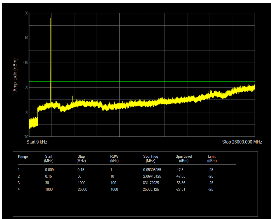
Band7 QAM16 BW=15MHz Channel=20825 RB Size=1 Position=#Mid
