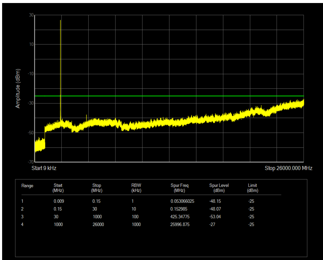
Band7 QPSK BW=20MHz Channel=20850 RB Size=1 Position=#Mid
