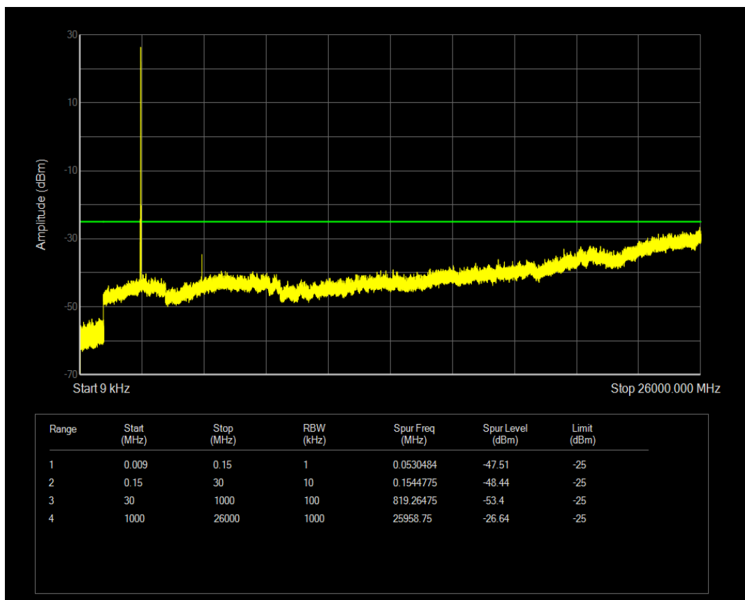
Band7 QPSK BW=10MHz Channel=21400 RB Size=1 Position=#Mid
