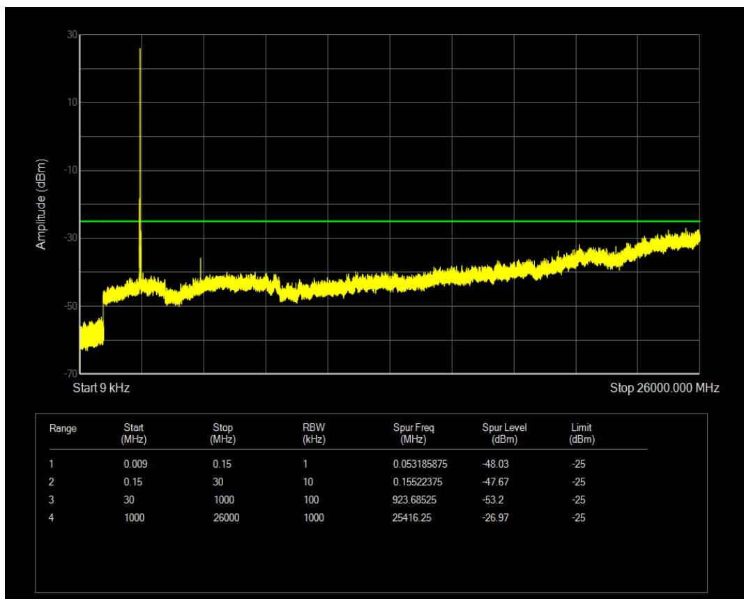
Band7 QPSK BW=15MHz Channel=21100 RB Size=36 Position=#0
