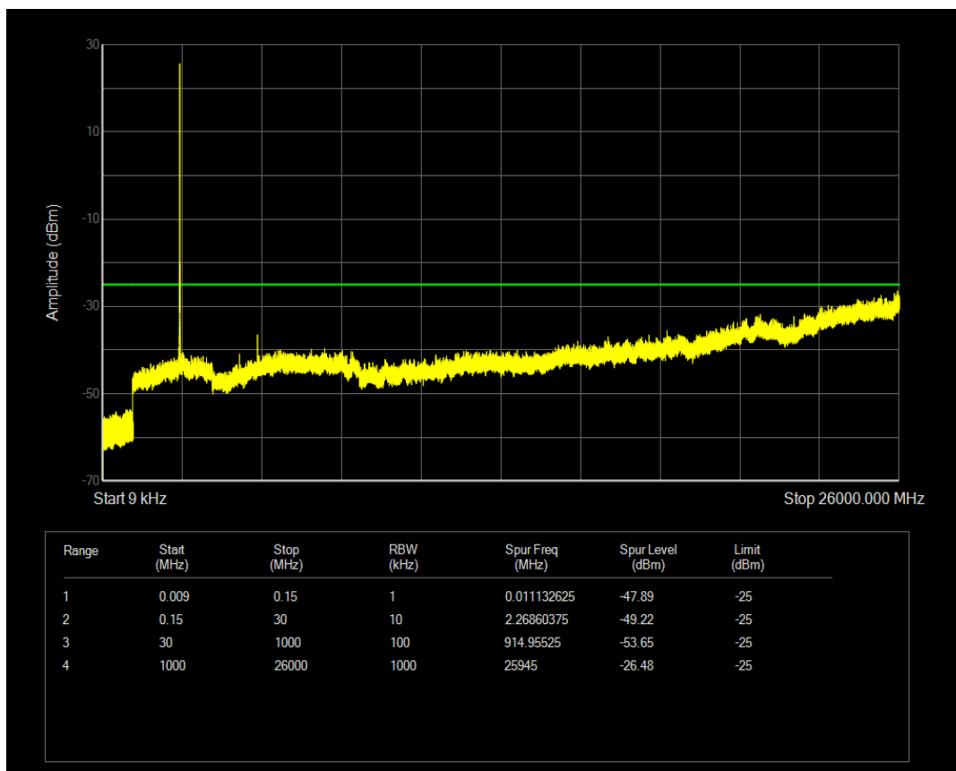
Band7 QPSK BW=15MHz Channel=21100 RB Size=1 Position=#Mid
