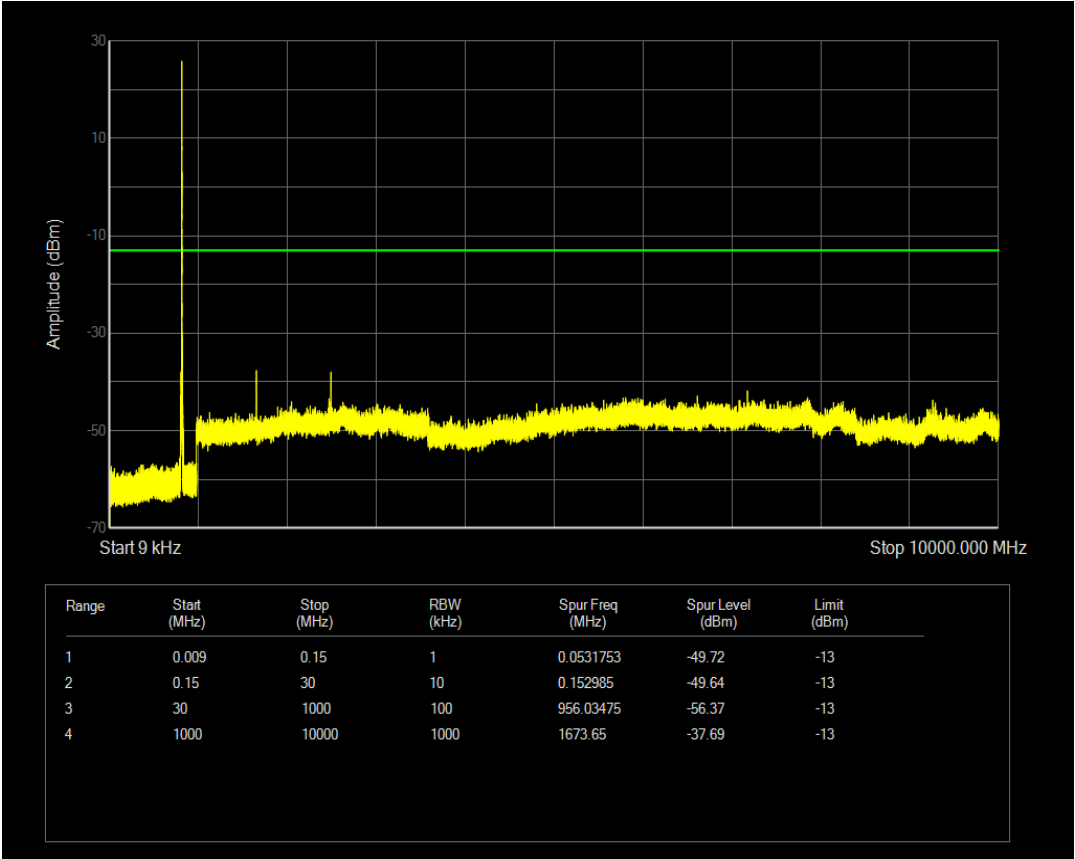
Band5 QPSK BW=10MHz Channel=20525 RB Size=1 Position=#Mid
