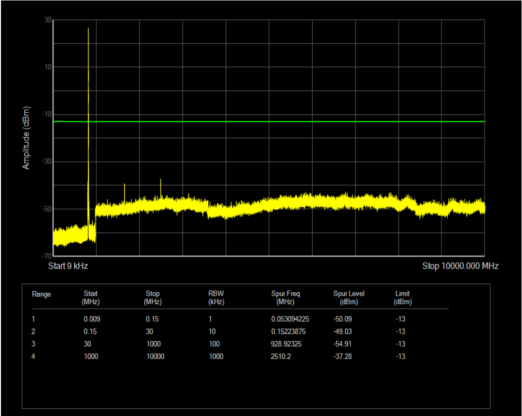
Band5 QAM16 BW=10MHz Channel=20525 RB Size=1 Position=#Mid
