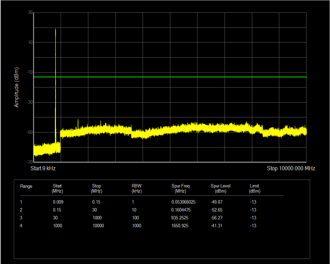
Band5 QPSK BW=5MHz Channel=20425 RB Size=12 Position=#0
