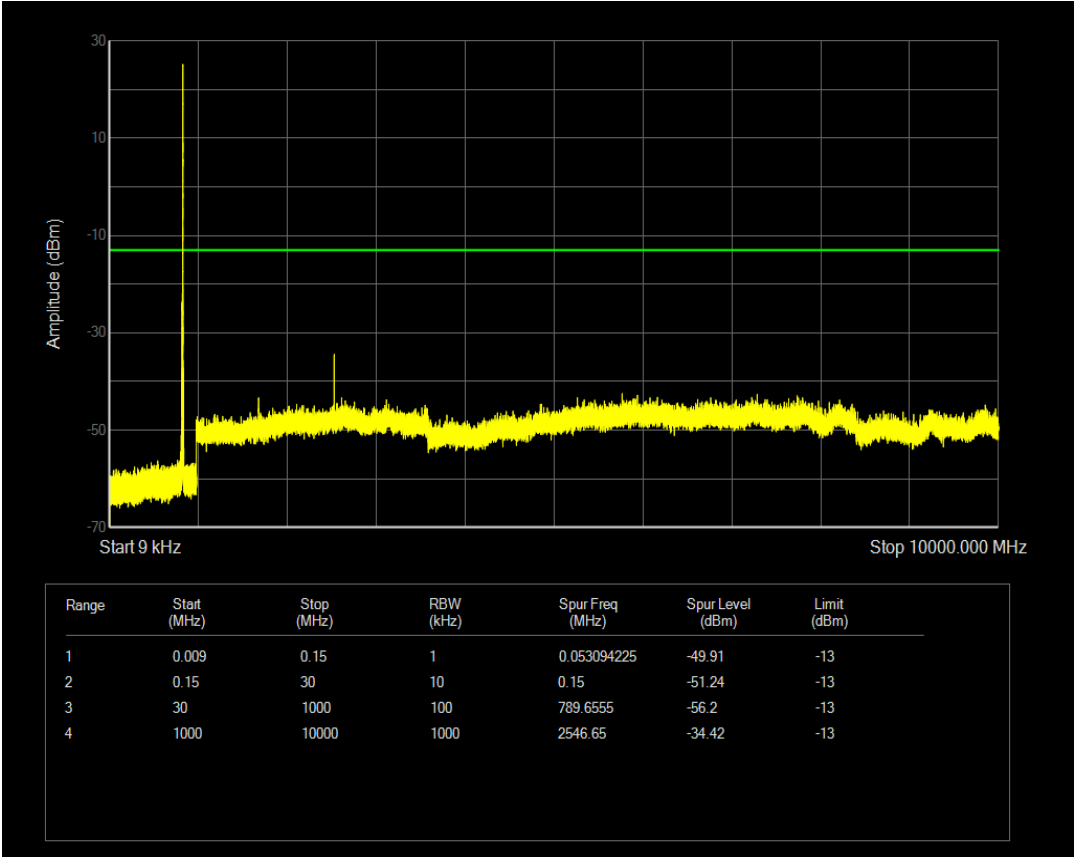
Band5 QPSK BW=5MHz Channel=20625 RB Size=12 Position=#0
