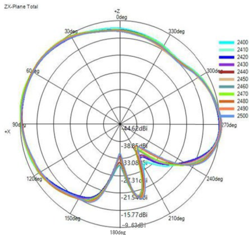
(1) X-Z Plane(unit:dBi):
