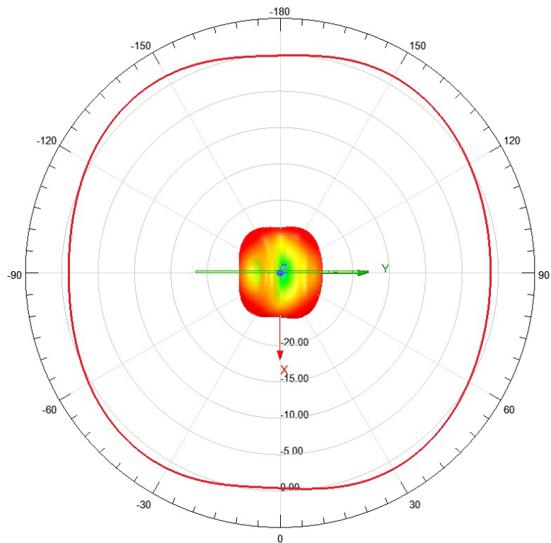
Figure 2- Azimuth cut (XY plane)
