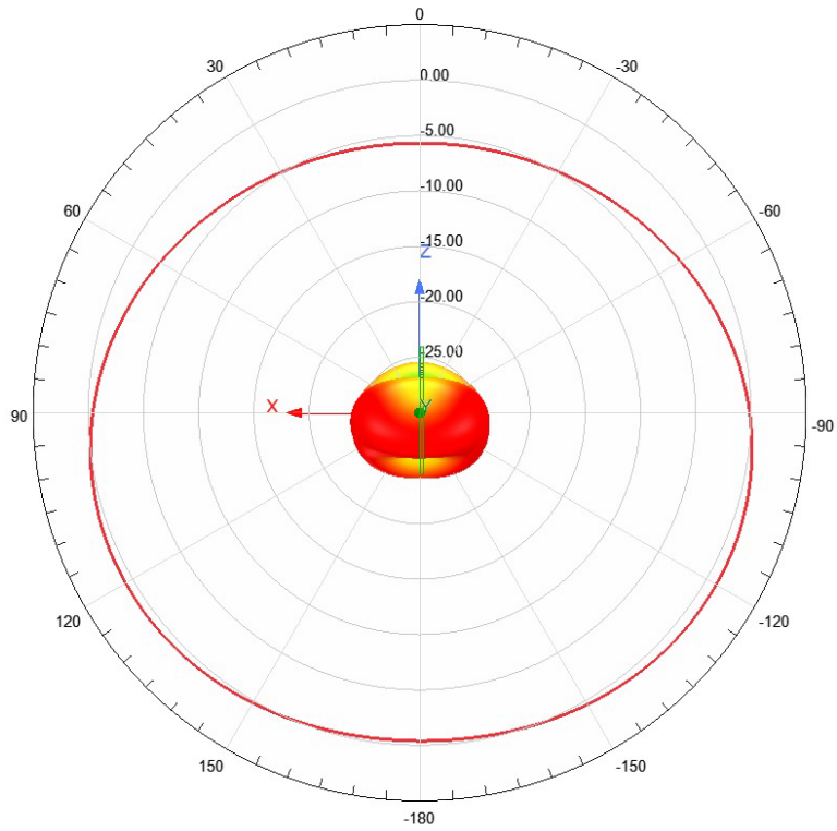
Figure 3- Elevation cut (ZX plane)
