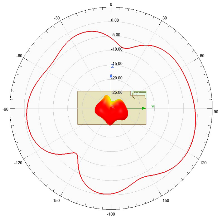
Figure 4- Elevation cut (ZY plane)
