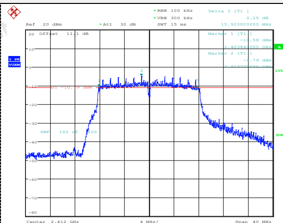
802.11g
