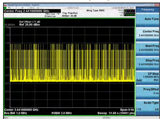
Accumulate(3DH5)
