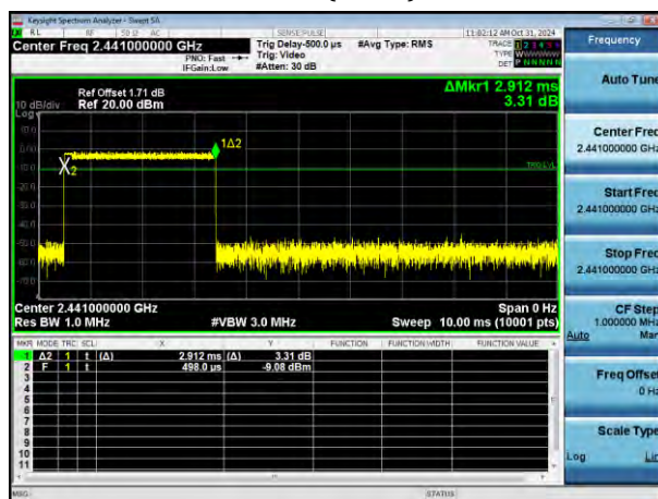
Burst(3DH5)
