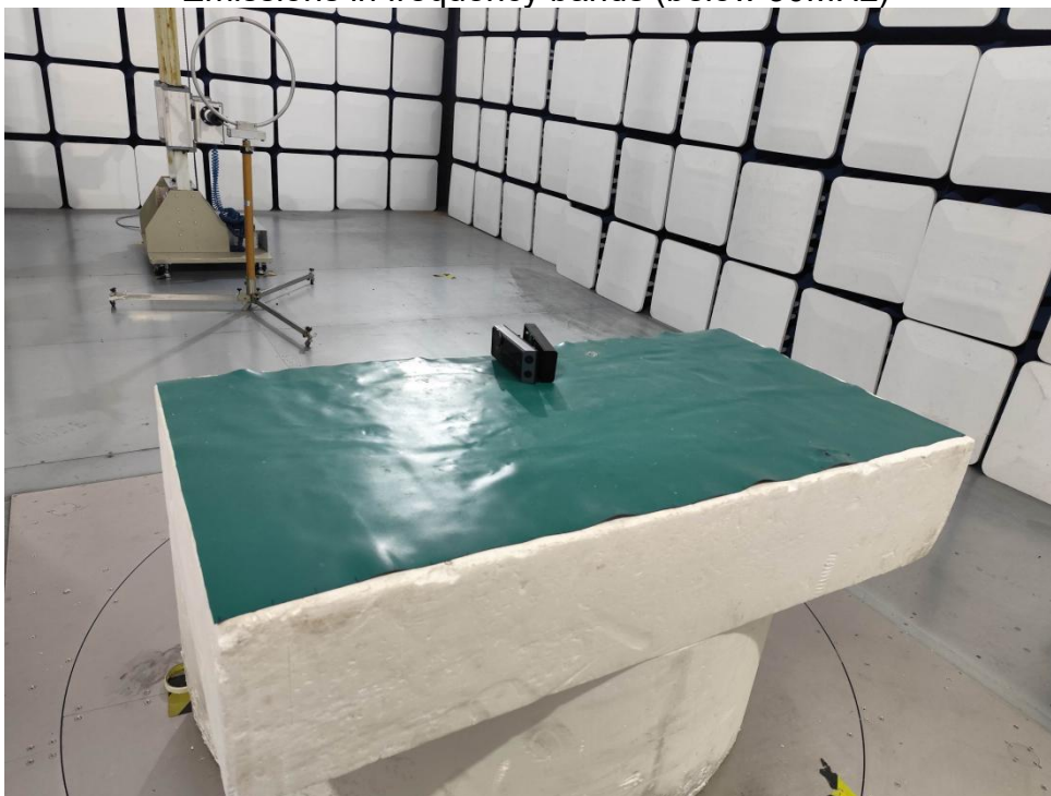
Emissions in frequency bands (below 30MHz)
