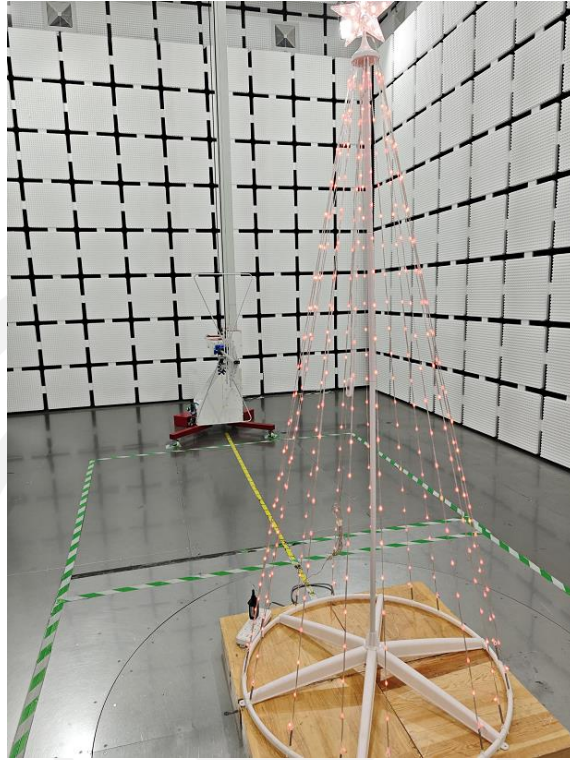
Spurious Radiation Emissions Test (<1G)
