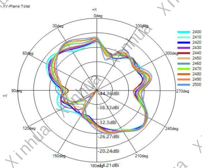
(1) X-Y Plane(unit:dBi):
