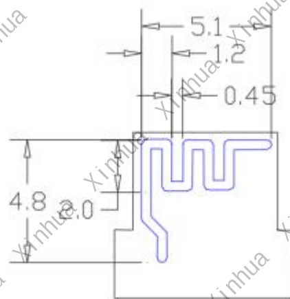
Antenna Dimensions
