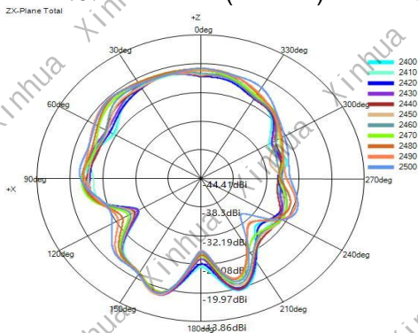
(3) Z-X Plane(unit:dBi):
