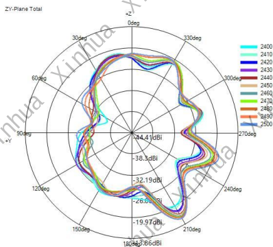
(2) Z-Y Plane(unit:dBi):
