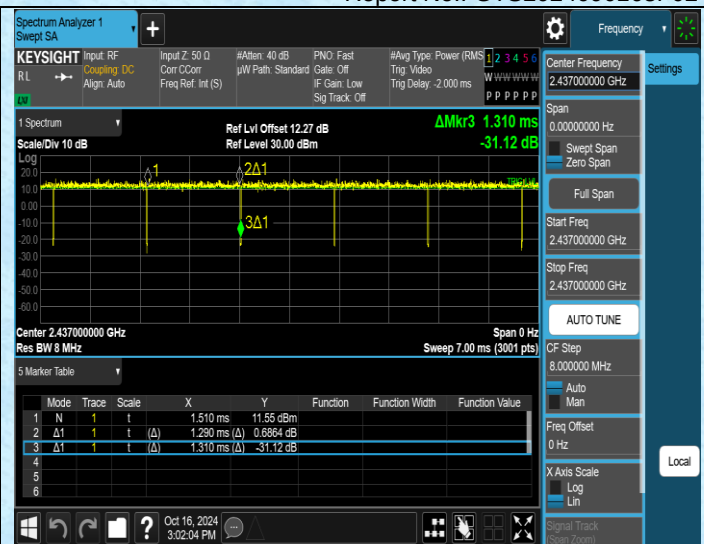
NTNV-11N20SISO-Ant1-2437
