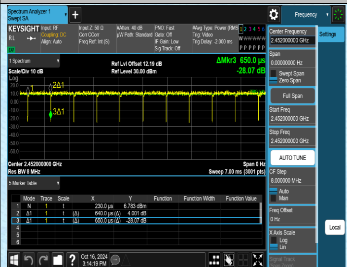
NTNV-11N40SISO-Ant1-2452
