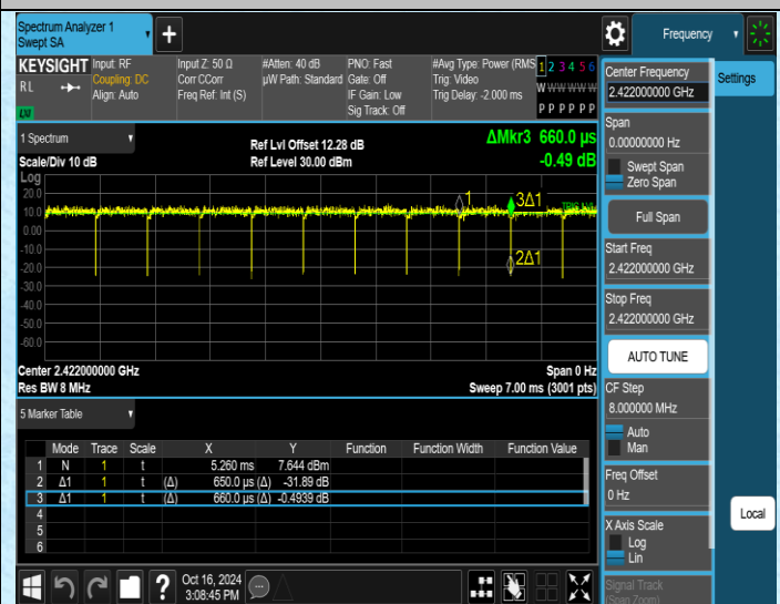
NTNV-11N40SISO-Ant1-2422
