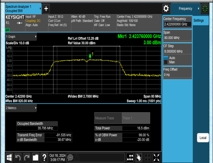
11N40SISO-Ant1-2422
