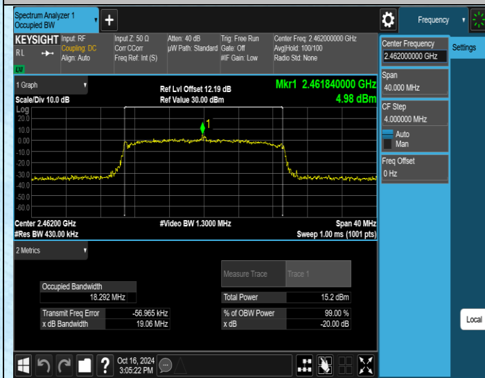
11N20SISO-Ant1-2462
