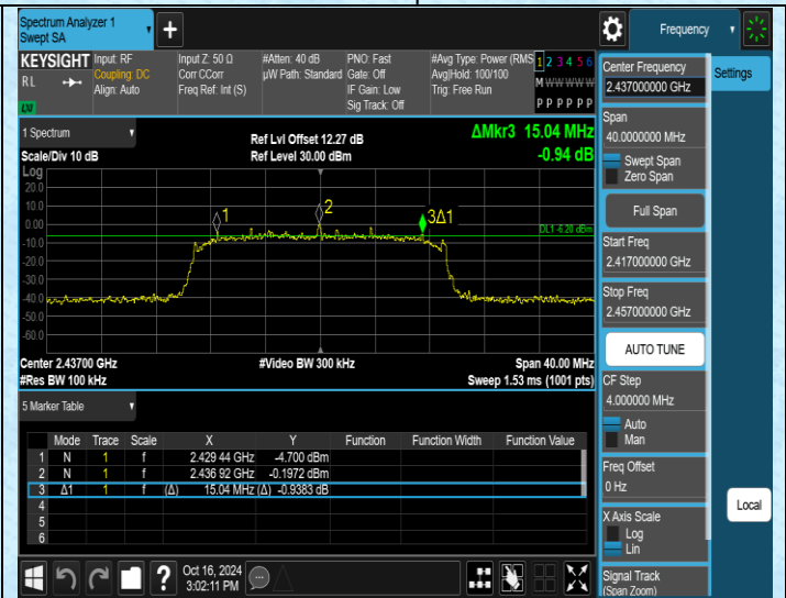
11N20SISO-Ant1-2437-PASS
